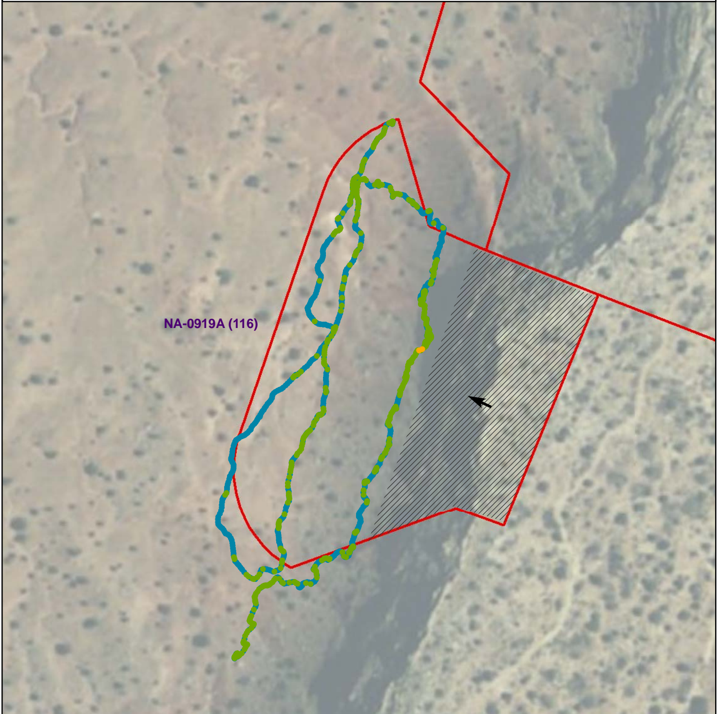
Figure 2 - Gamma Radiation Measurements NA-0919A (116) Teec Nos Pos Chapter, Navajo Nation
