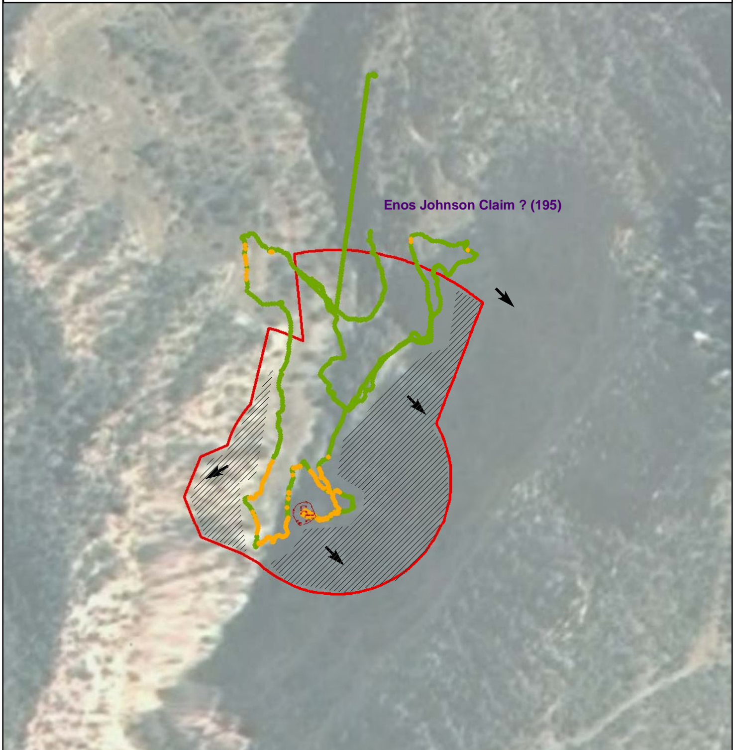
Figure 1 - Gamma Radiation Measurements, Above Two Times Background Enos Johnson Claim? (195) Sanostee Chapter, Navajo Nation, Arizona
