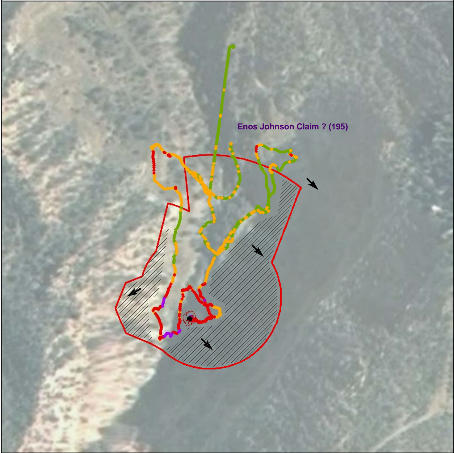
Figure 2 - Gamma Radiation Measurements Enos Johnson Claim ? (195) Sanostee Chapter, Navajo Nation, Arizona
