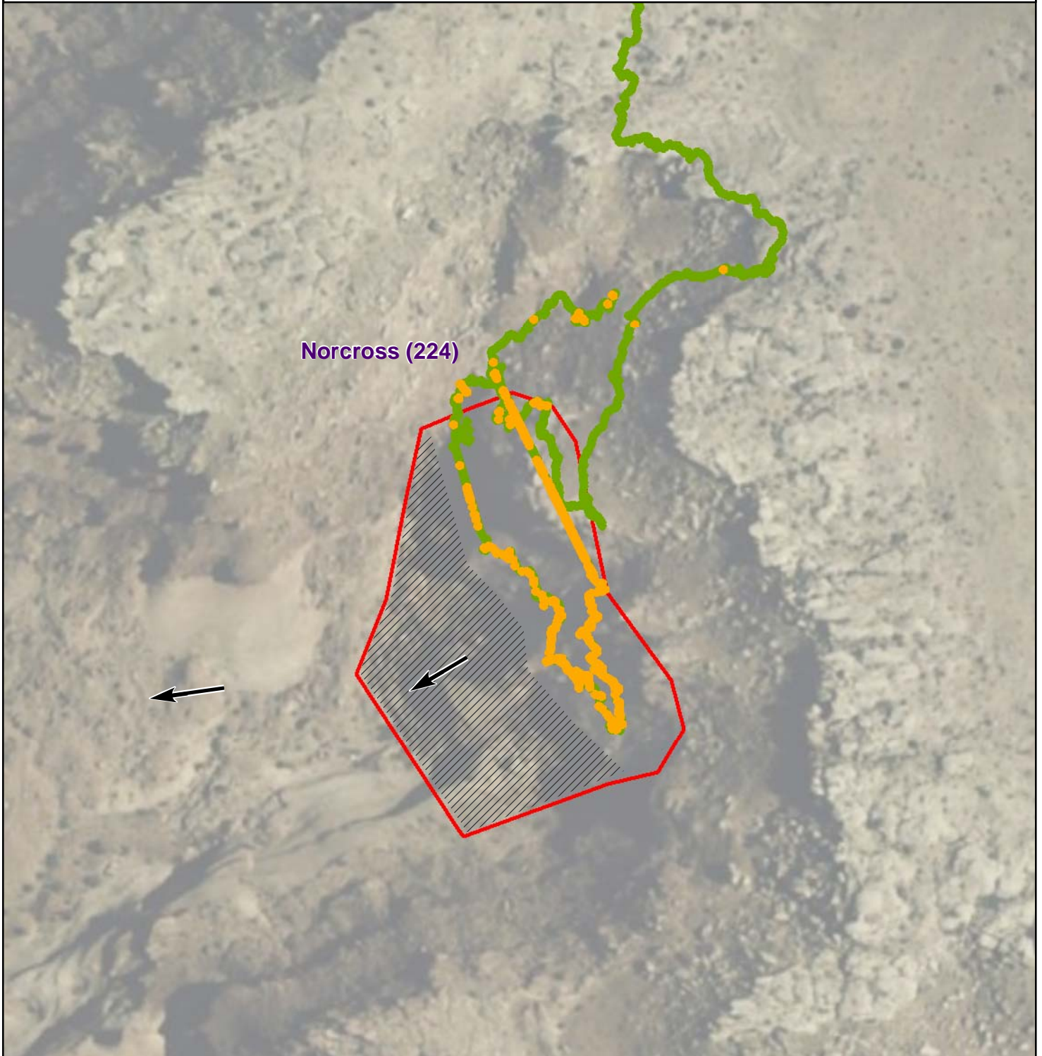
Figure 1 - Gamma Radiation Measurements, Above Two Times Background Norcross (224) Oljato Chapter, Navajo Nation
