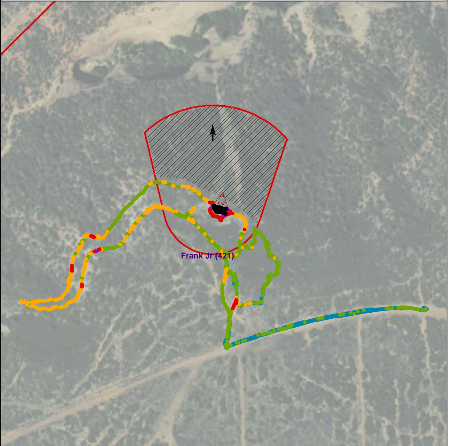
Figure 2 - Gamma Radiation Measurements Frank Jr (421) Cove Chapter, Navajo Nation, Arizona
