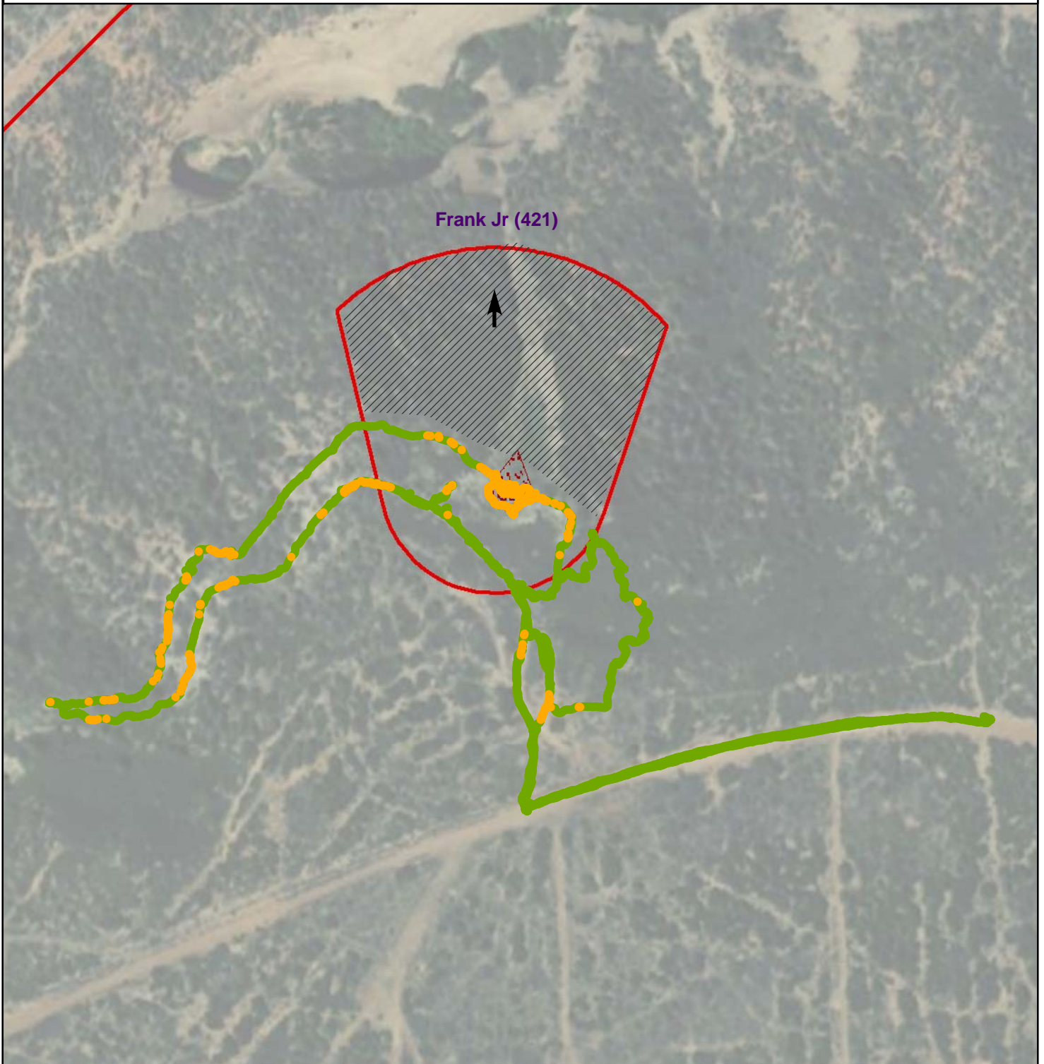
Figure 1 - Gamma Radiation Measurements, Above Two Times Background Frank Jr (421) Cove Chapter, Navajo Nation, Arizona
