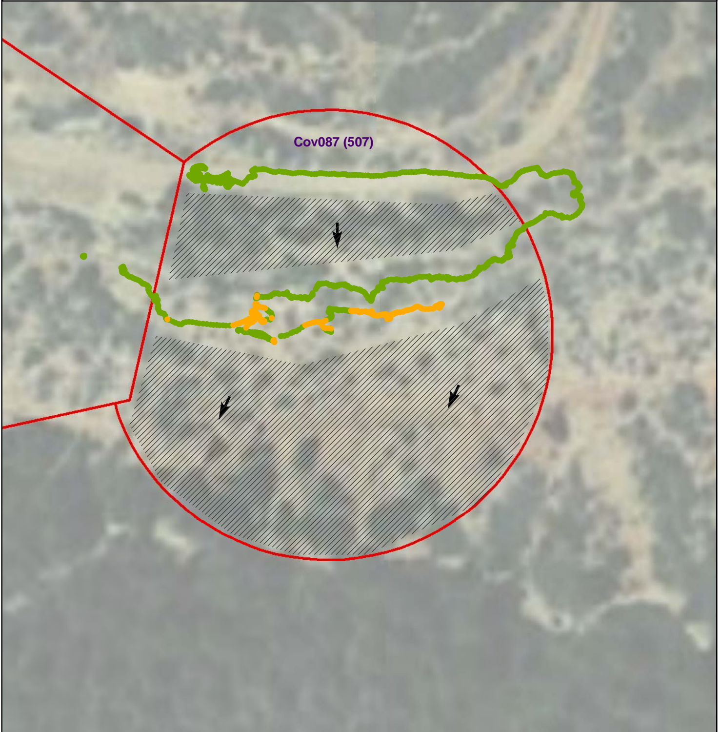
Figure 1 - Gamma Radiation Measurements, Above Two Times Background Cov087 (507) Cove Chapter, Navajo Nation, Arizona
