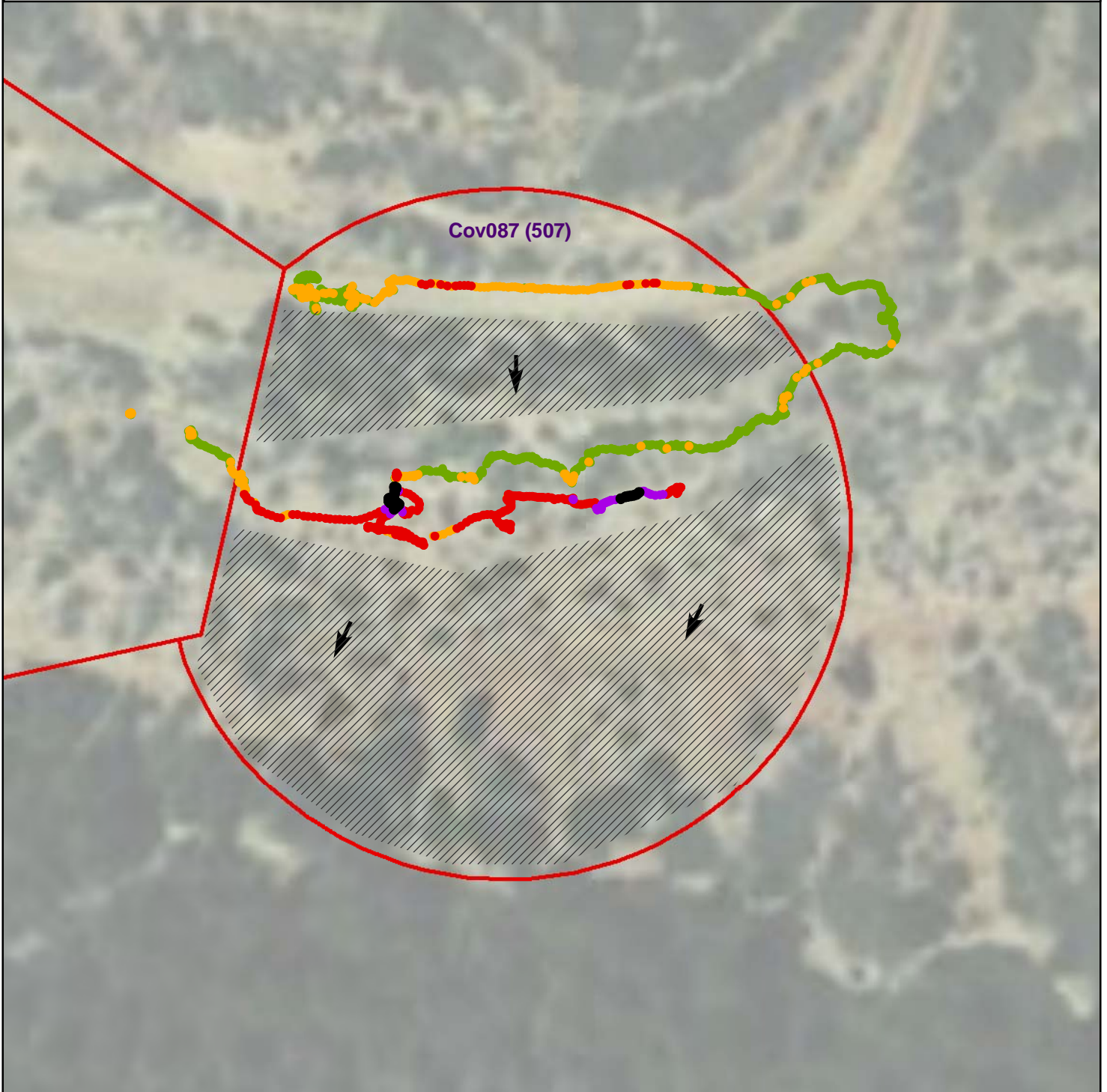
Figure 2 - Gamma Radiation Measurements Cov087 (507) Cove Chapter, Navajo Nation, Arizona
