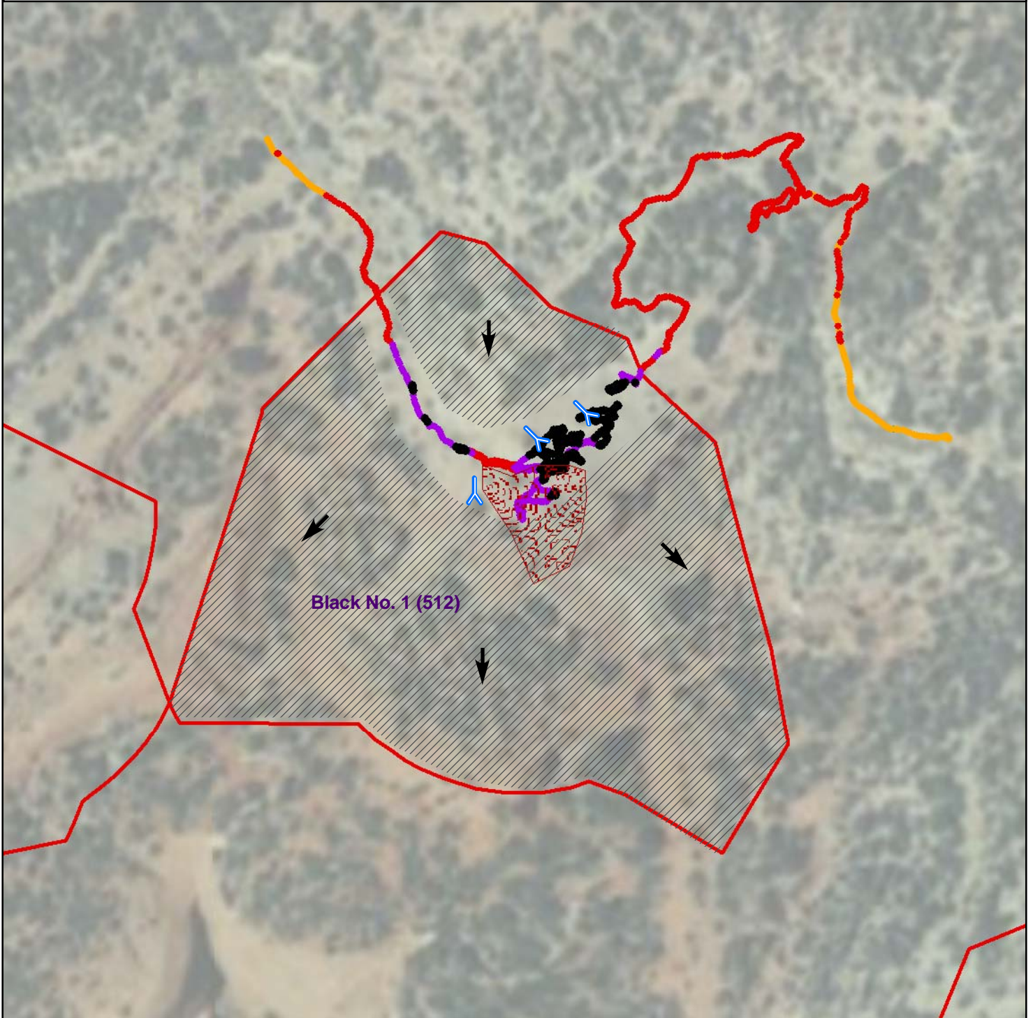
Figure 2 - Gamma Radiation Measurements Black No. 1 Mine (512) Round Rock Chapter, Navajo Nation, Arizona
