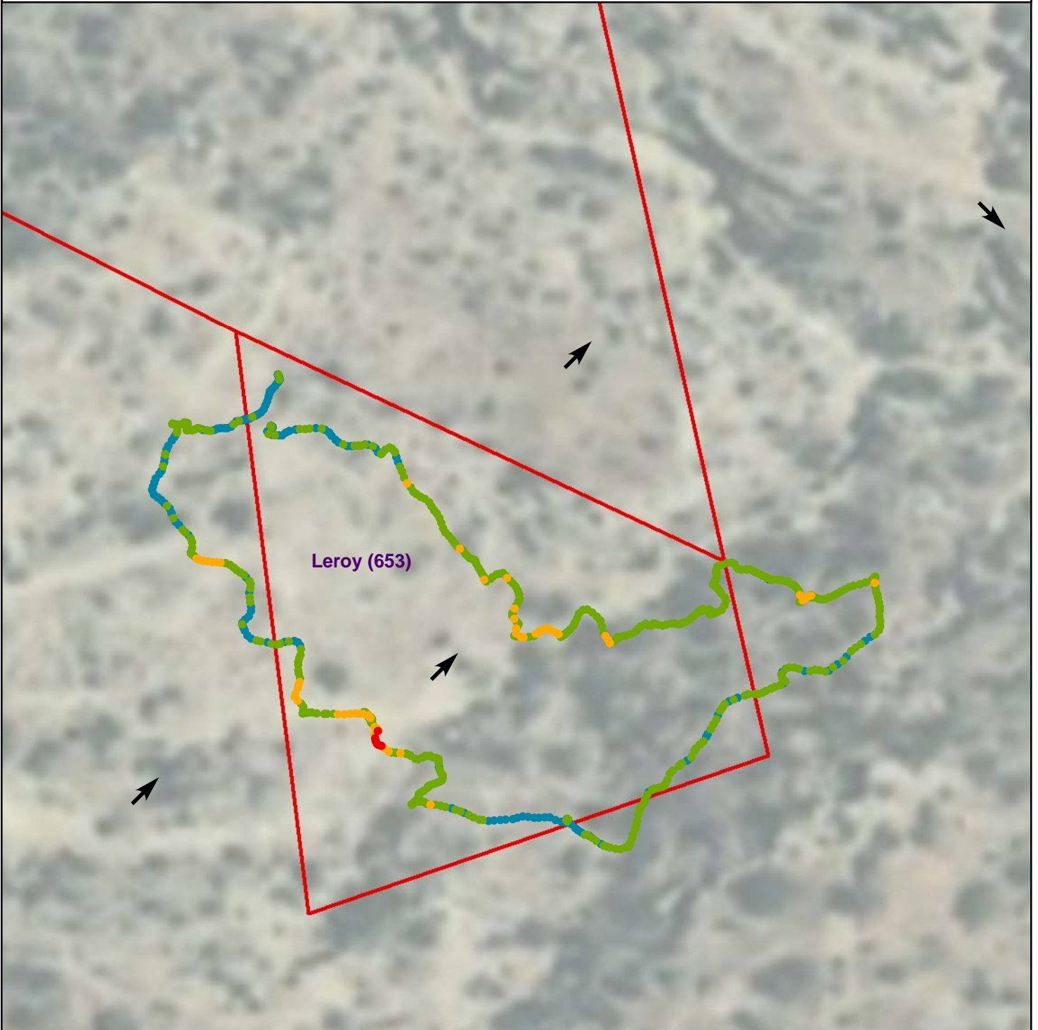
Figure 2 - Gamma Radiation Measurements Leroy (653) Red Valley Chapter, Navajo Nation, Arizona
