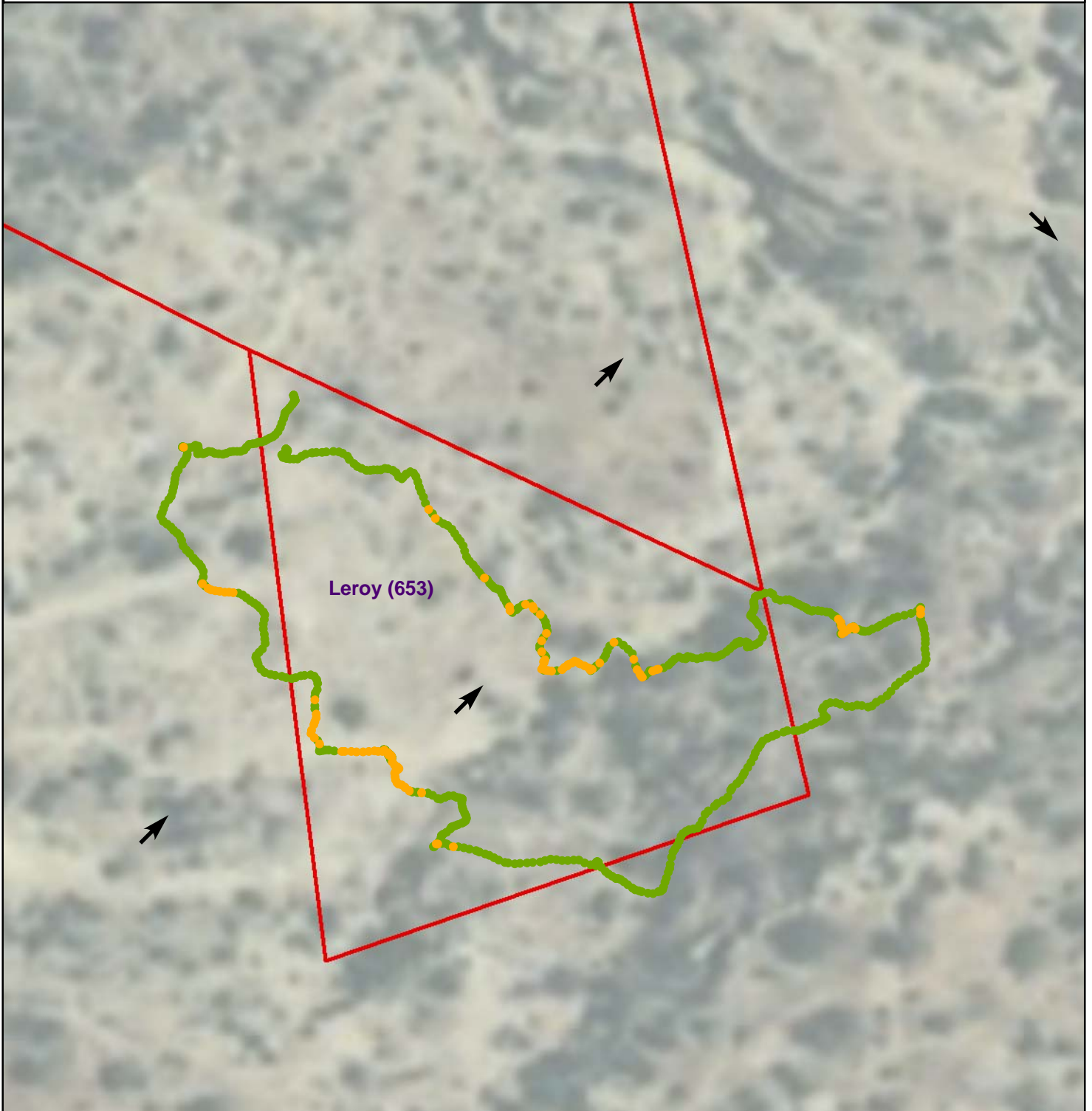
Figure 1 - Gamma Radiation Measurements, Above Two Times Background Leroy (653) Red Valley Chapter, Navajo Nation, Arizona
