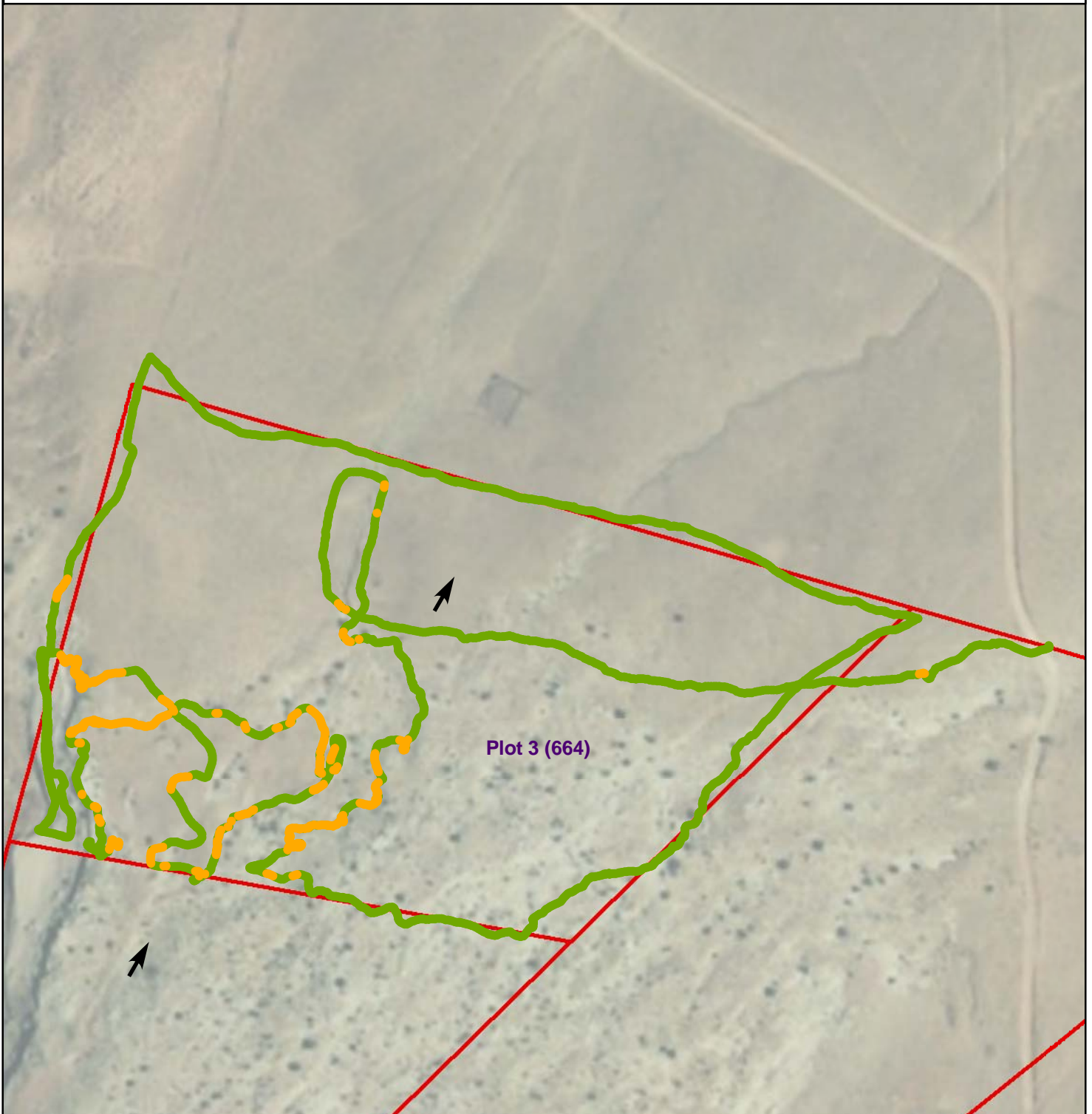
Figure 1 - Gamma Radiation Measurements, Above Two Times Background Plot 3 (664) Teec Nos Pos Chapter, Navajo Nation
