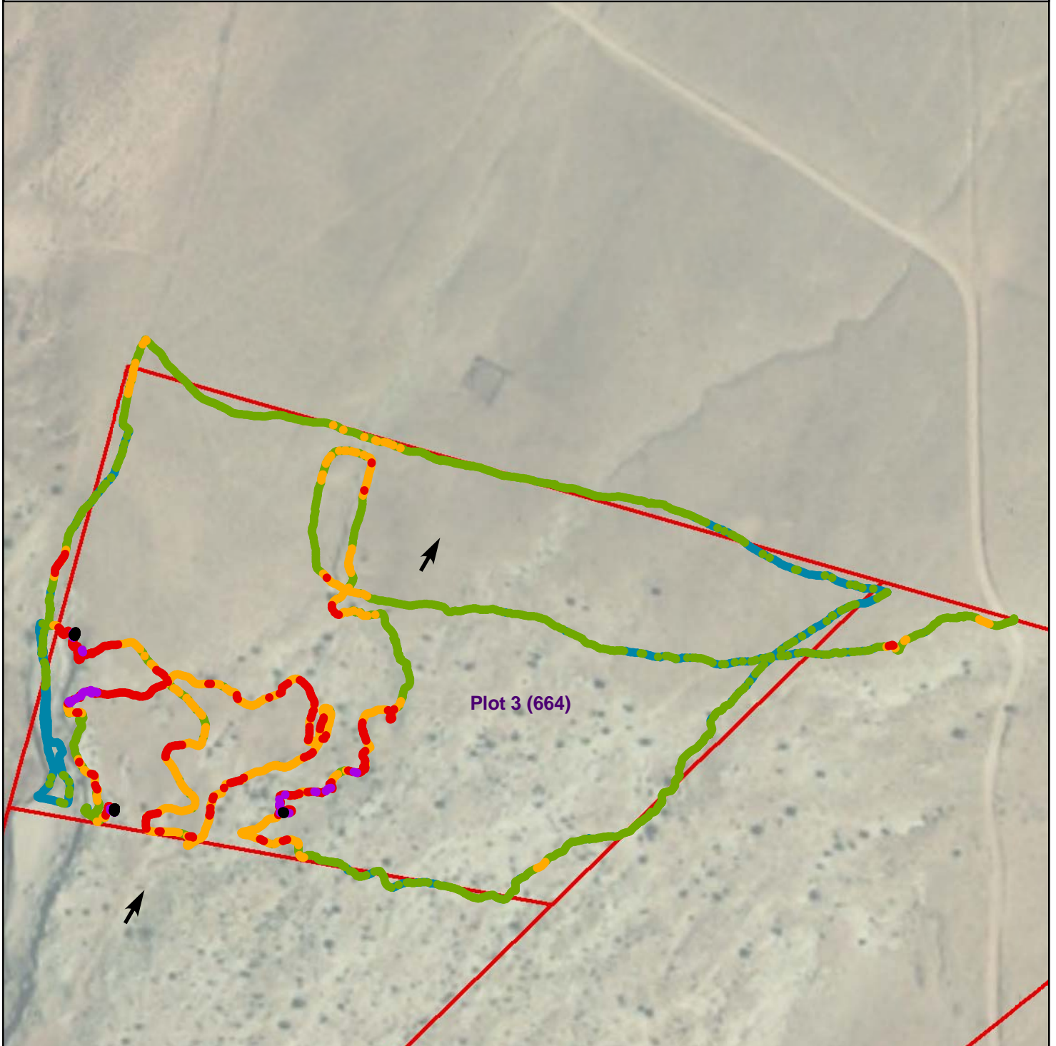
Figure 2 - Gamma Radiation Measurements Plot 3 (664) Teec Nos Pos Chapter, Navajo Nation
