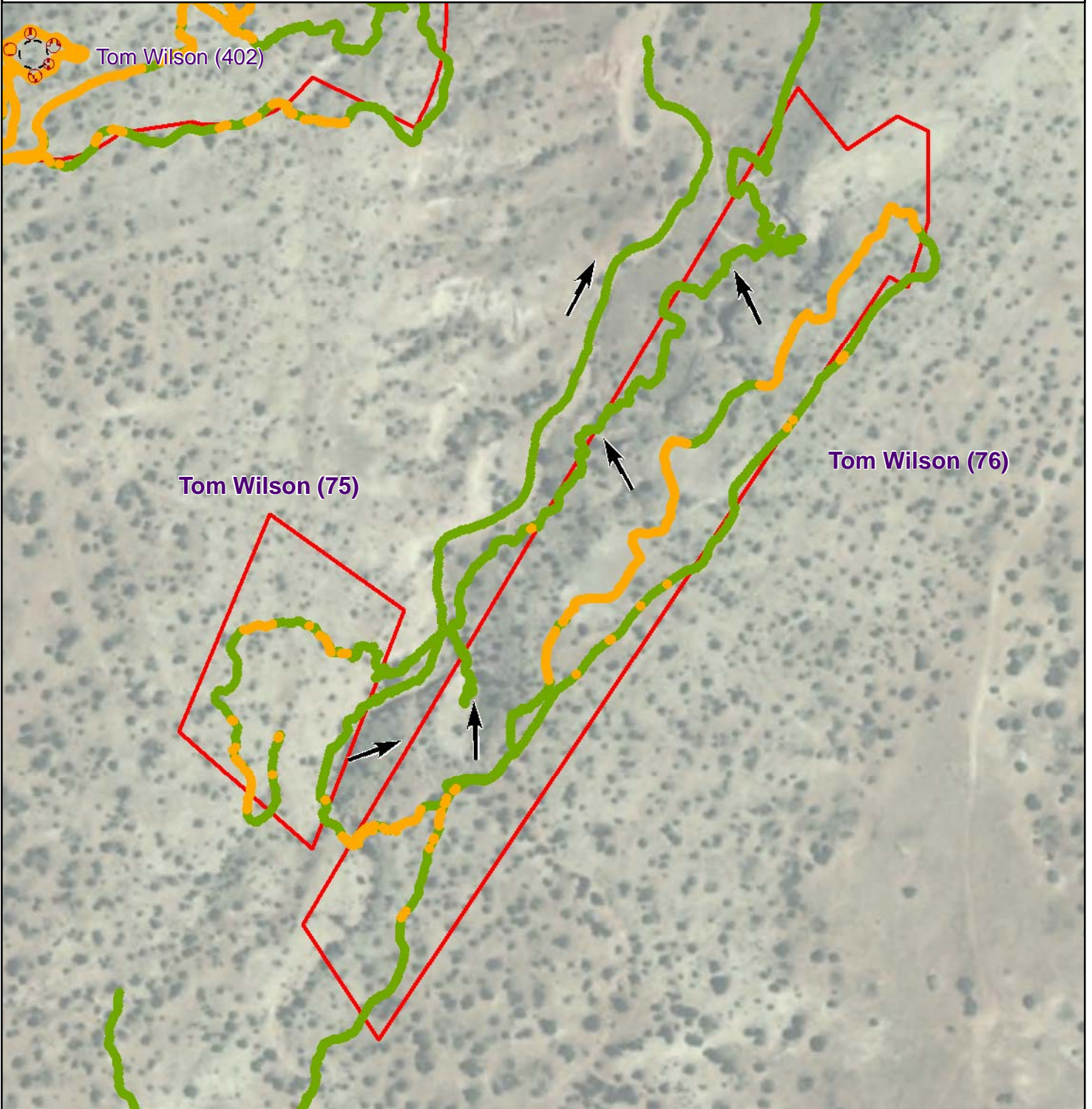
Figure 3 - Gamma Radiation Measurements, Above Two Times Background Tom Wilson (75, 76) Chilchinbito Chapter, Navajo Nation
