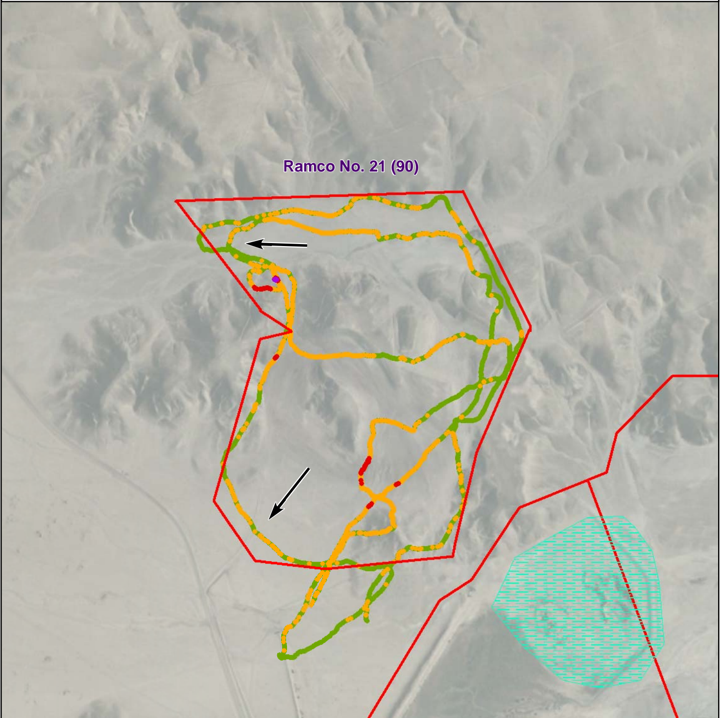
Figure 2 - Gamma Radiation Measurements Ramco No. 21 (90) Coalmine Mesa Chapter, Navajo Nation
