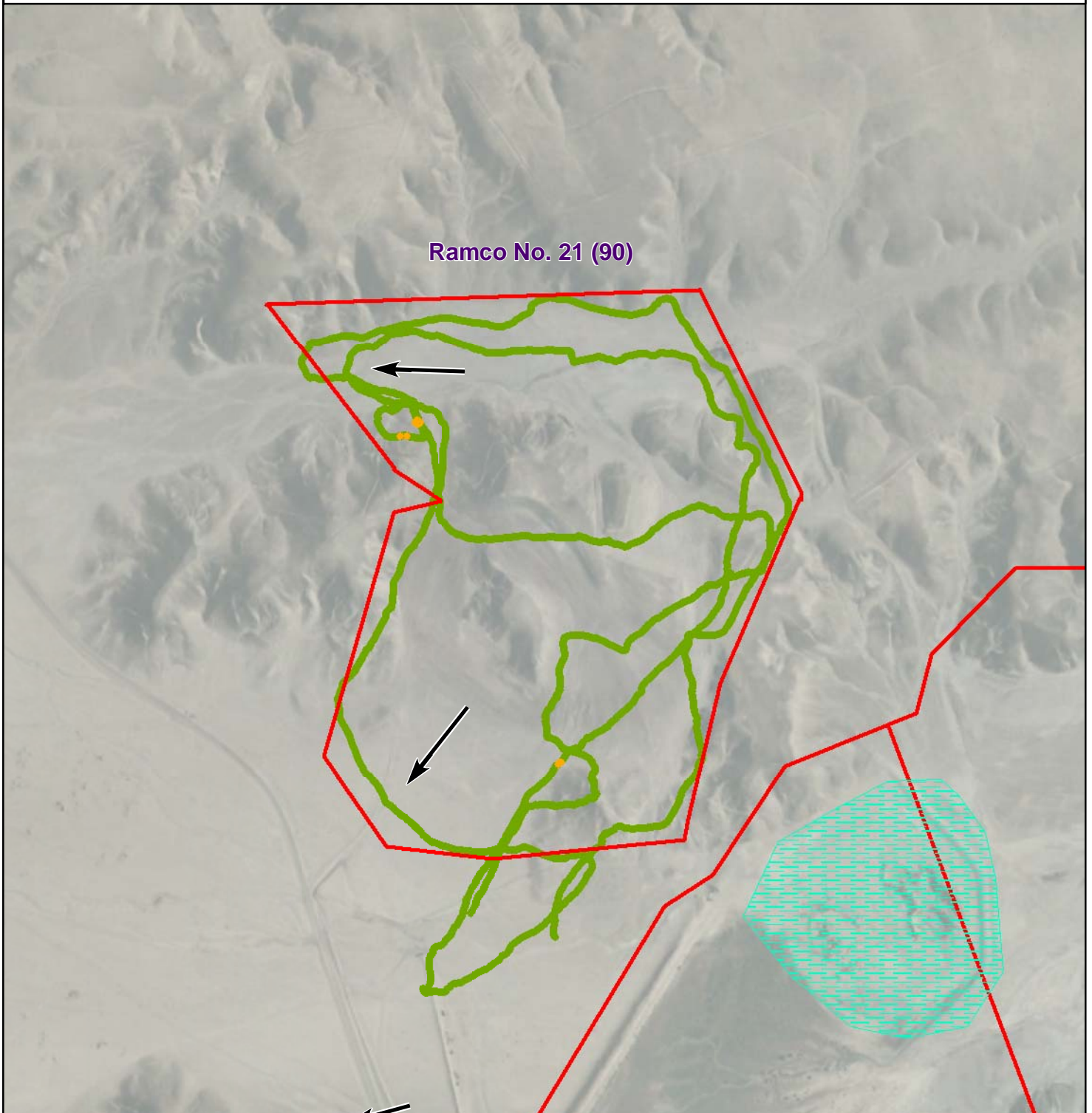
Figure 1 - Gamma Radiation Measurements, Above Two Times Background Ramco No. 21 (90) Coalmine Mesa Chapter, Navajo Nation
