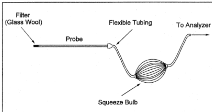
Figure 3-1. Grab-Sampling Train.
