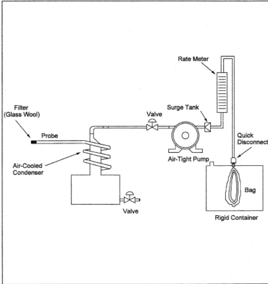
Figure 3-2. Integrated Gas-Sampling Train.
