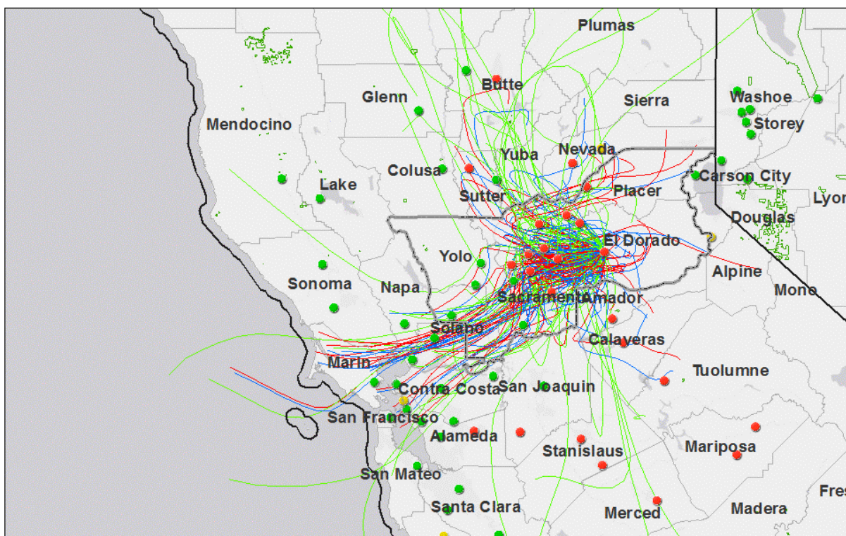
Figure 13.6a HYSPLIT Back Trajectories for Placerville (06-017-0010).
