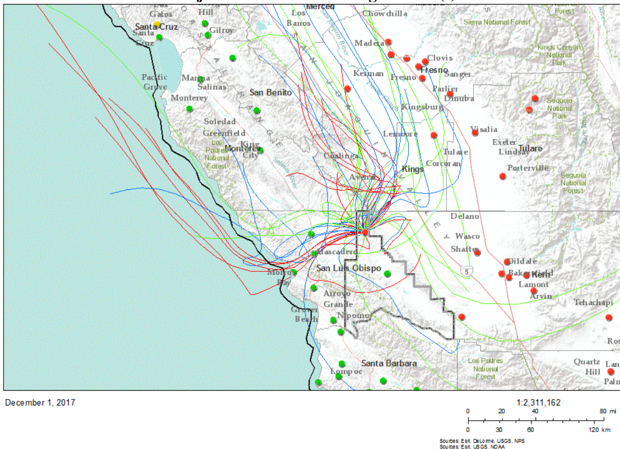
Figure 17.6 HYSPLIT Back Trajectories for the Violating Monitor(s).
