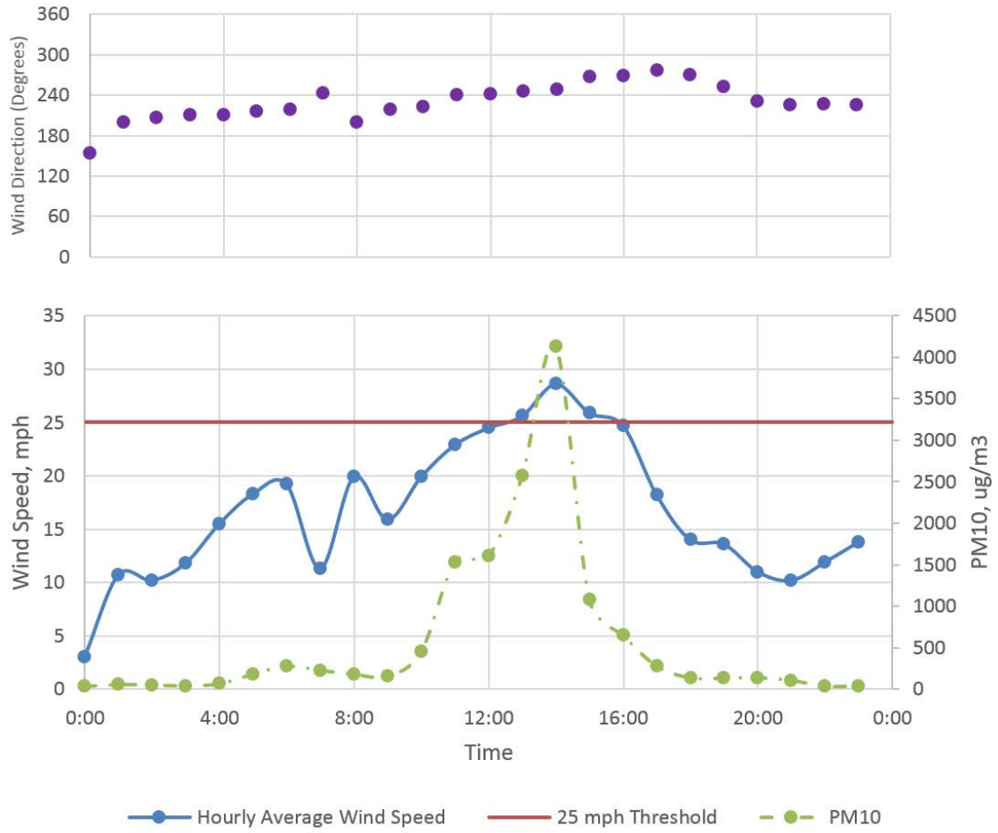
Figure 10. Hourly Average Wind Speed, PM 10 and Wind Direction at KENMETA on August 14, 2015
