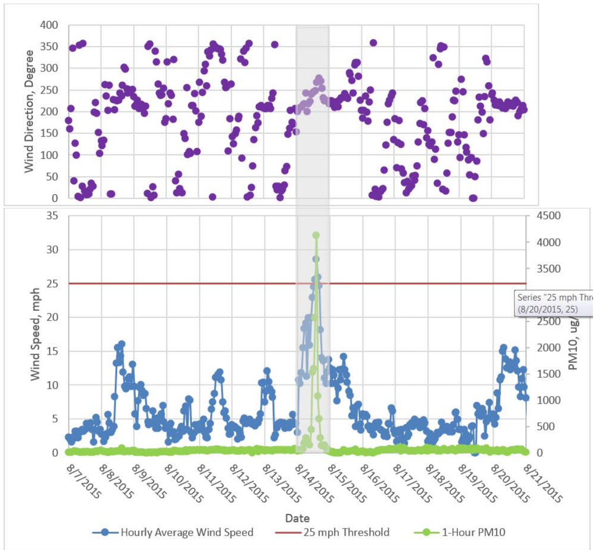
Figure 26. Hourly average wind speed, PM 10 and wind direction at KENMETA with the surrounding two weeks of the event day on August 14, 2015
