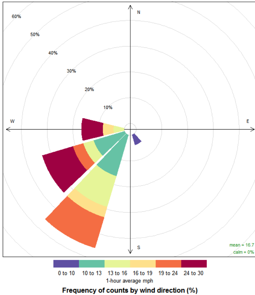
Kennewick Metaline Wind Rose, 8/14/2015
