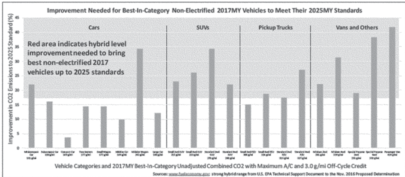
Figure 2: Figure submitted by the Alliance (p. 18) titled “Figure 5: Improvement in CO 2 Emissions Required in the Best MY 2017 Non-Electrified Vehicles to Meet MY 2025 Targets” 16
