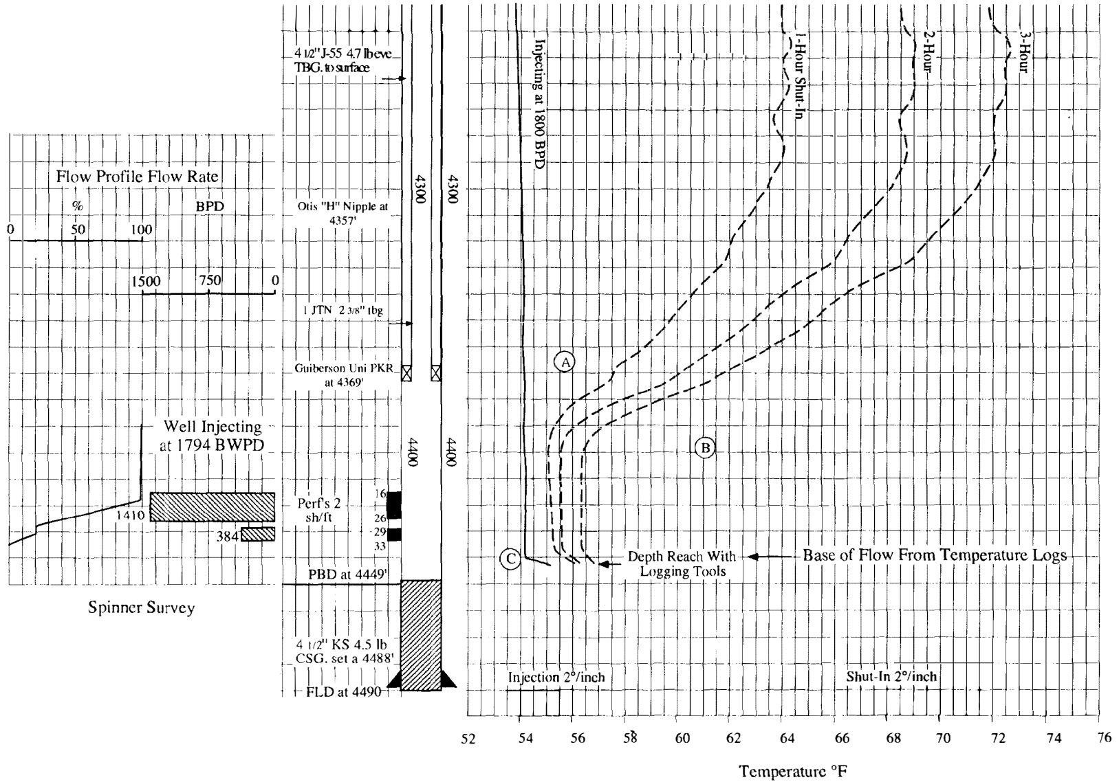
Figure 29. Surveys from an old injection well taking 1,800 BPD water.
