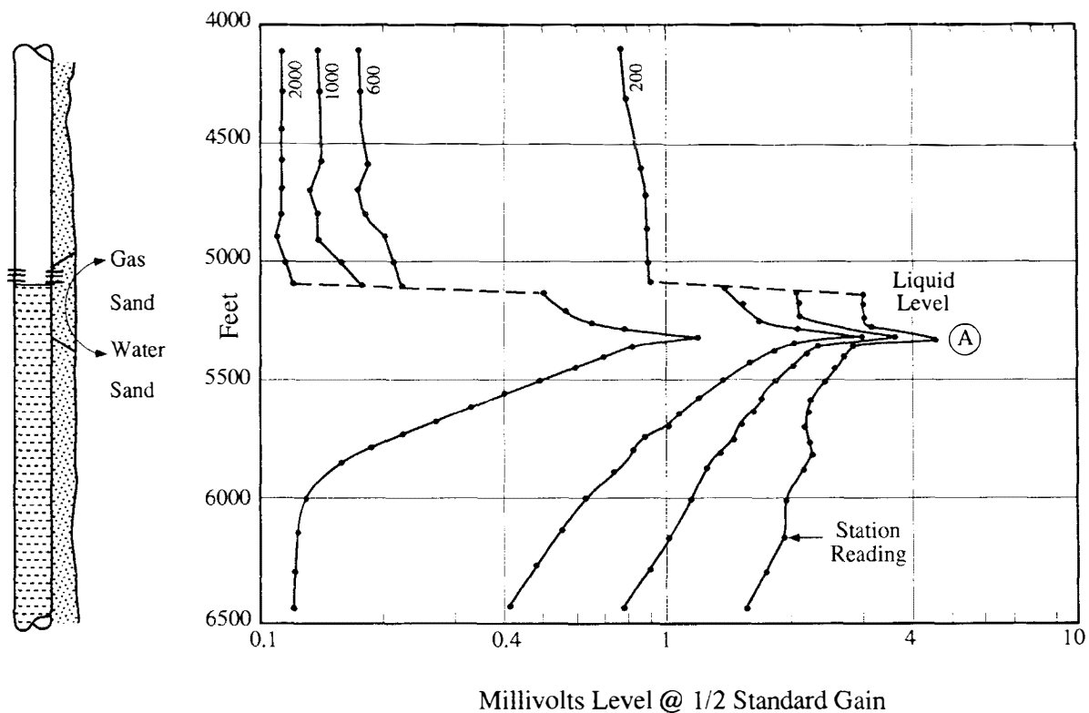
Figure 79. Noise log format with a 20-BPD water flow behind pipe into a gas zone depleted by 250 PSI.
