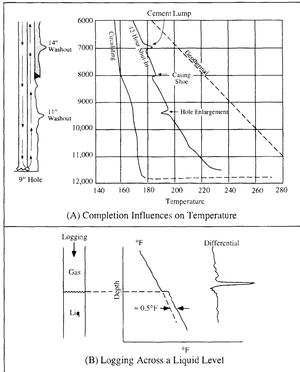
Figure 8. Wellbore influence on temperature surveys.
