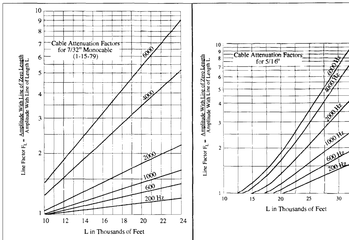
Figure 80. Logging cable attenuation factors for two wireline sizes.
