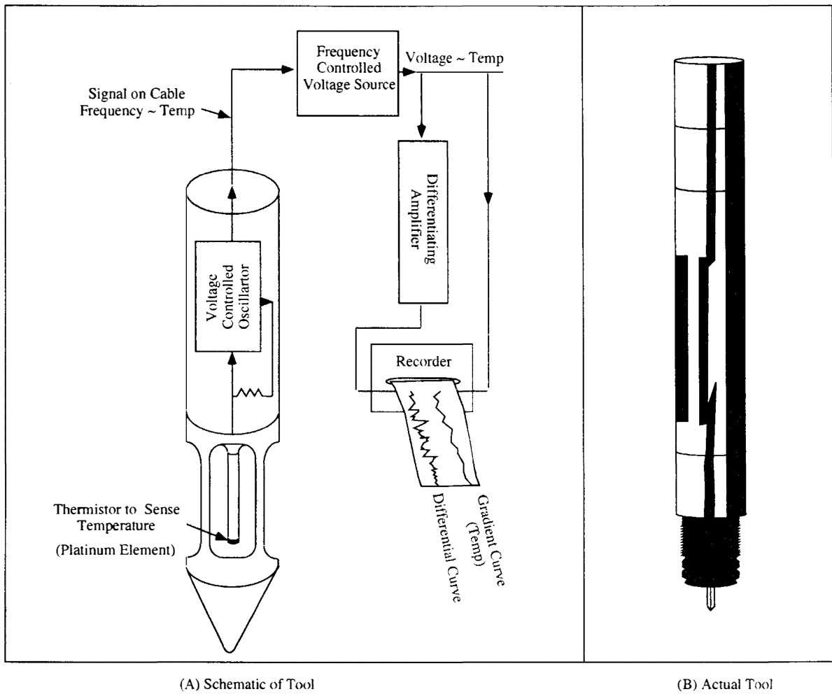
Figure 1. A surface recording, continuous thermometer.
