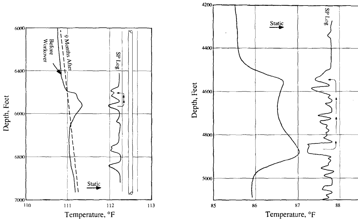
(A) Six-Hour Shut-In Surveys Before and After Workover
