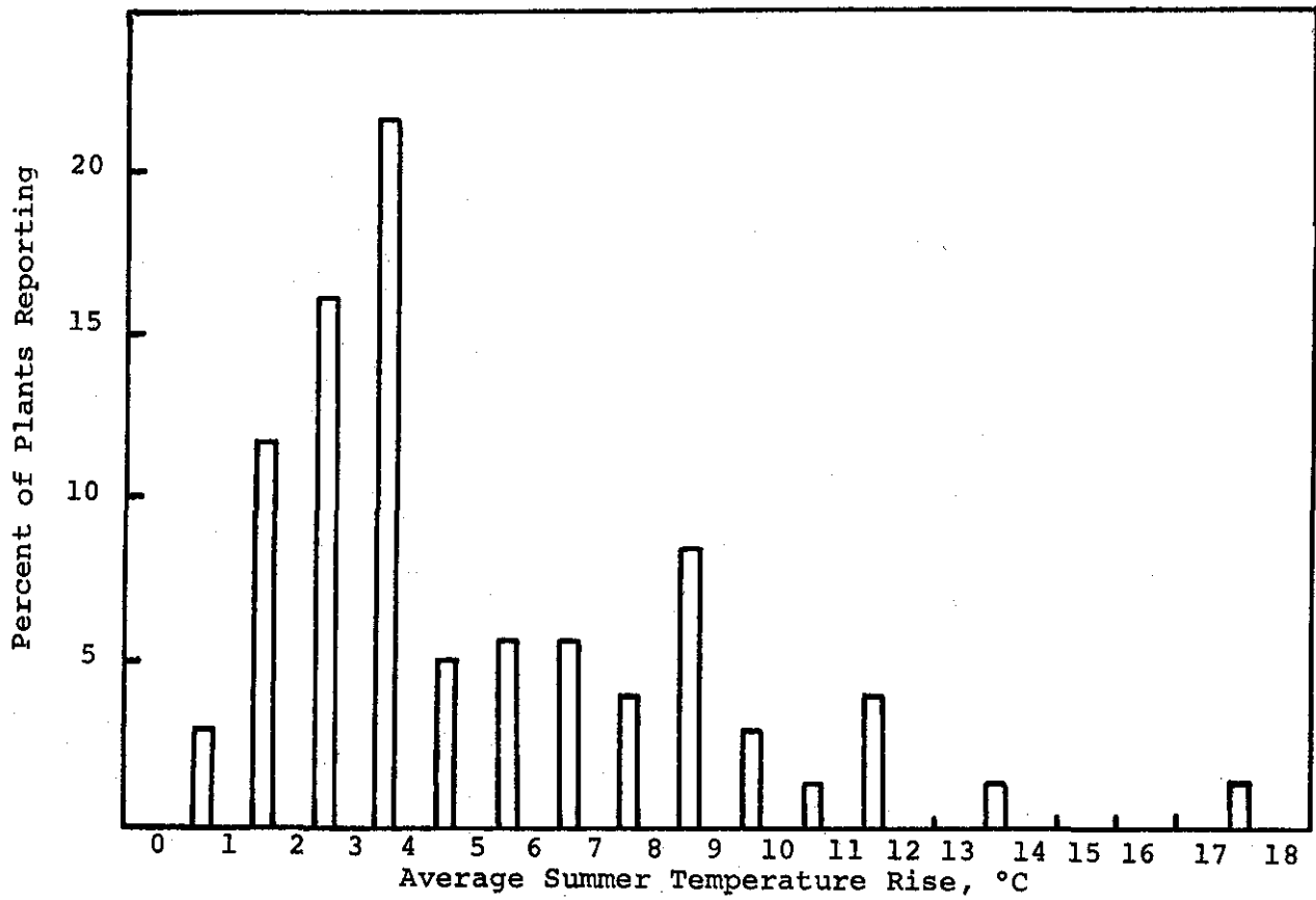
Figure 9. Distribution of Calculated Average Temperature Rise.
