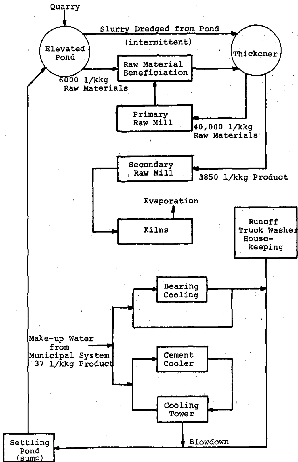
Figure 13. Diagram of Water-Management Plan for Plant A
