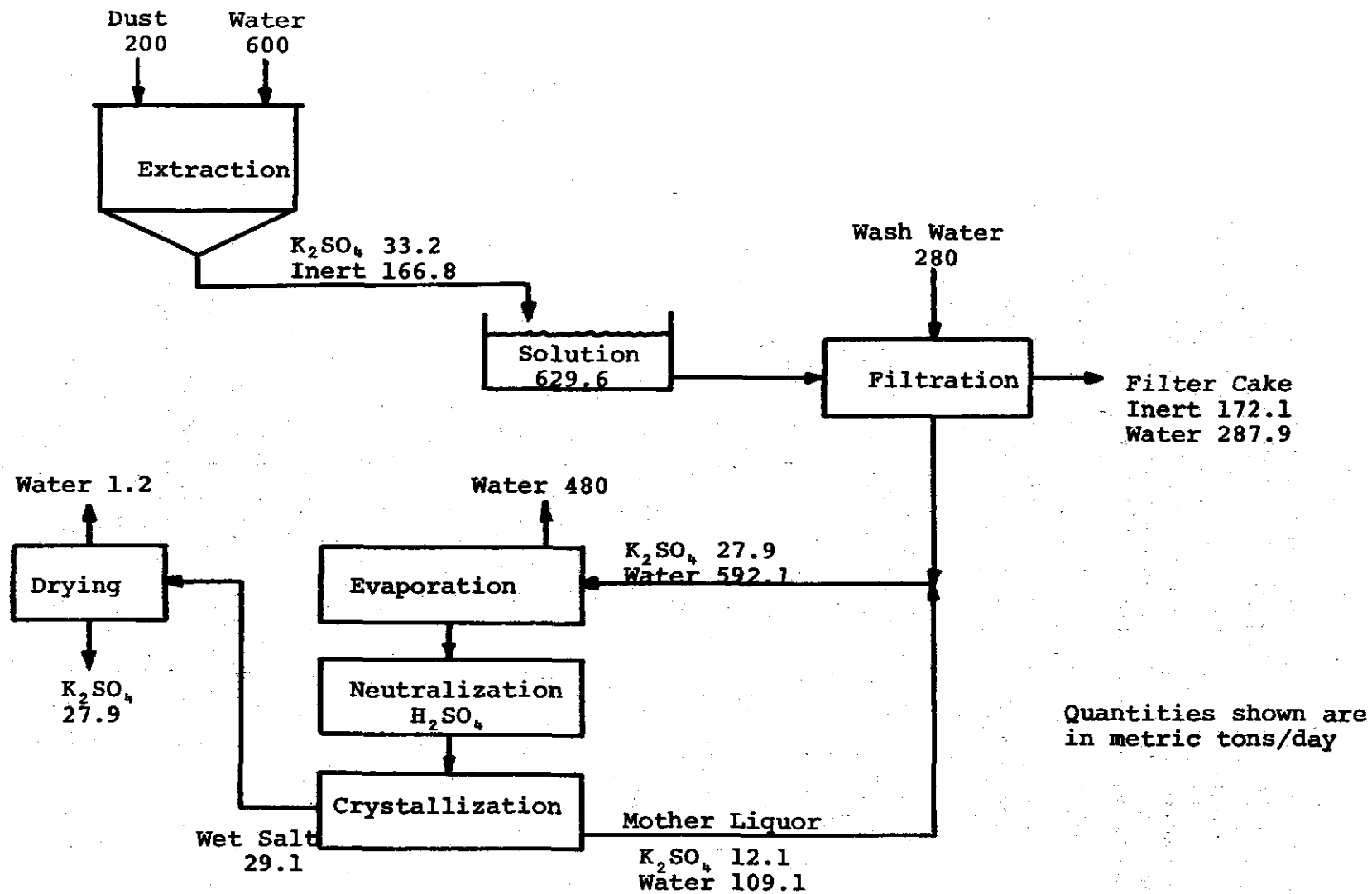
Figure 12. Flow Sheet for the Recovery of K_2SO_4 from Cement Kiln Dust.
