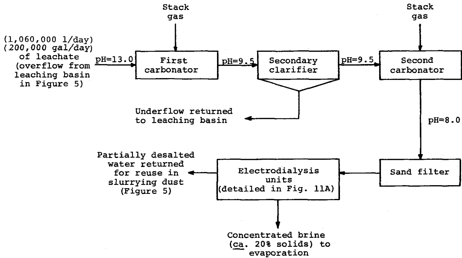
Figure 11. Flow Diagram Showing Steps in Electrolytic Concentration of Leachate
