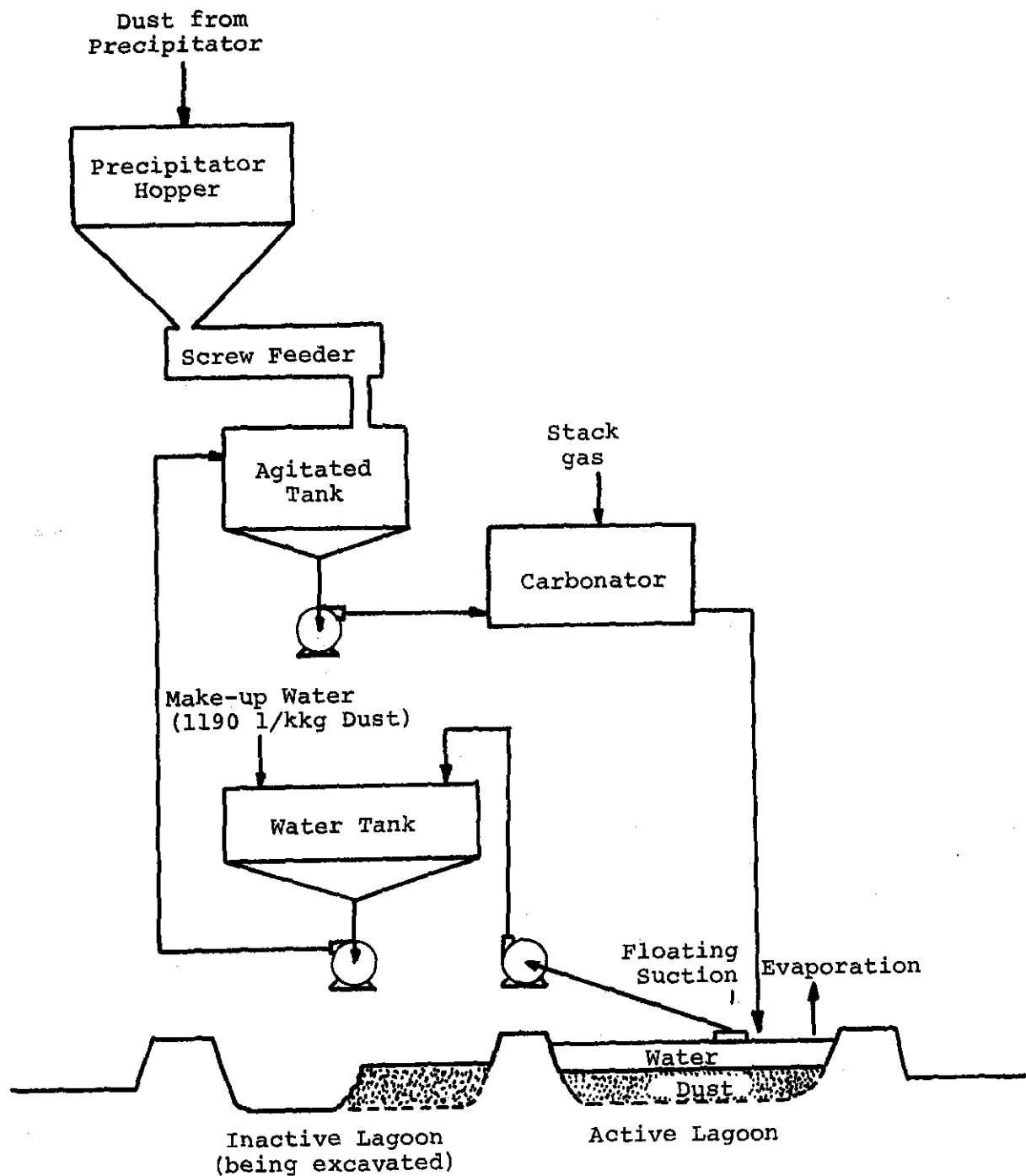
Figure 18. Diagram of Dust-Handling System at Plant H
