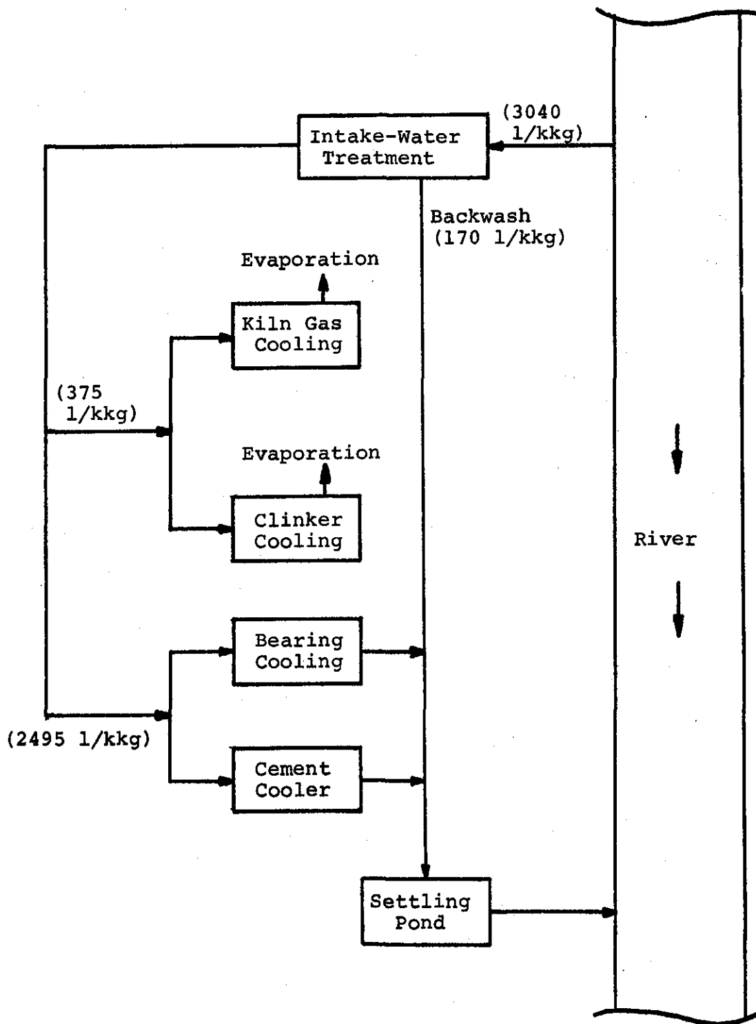
Figure 17. Diagram of Water-Management Plan for Plant G
