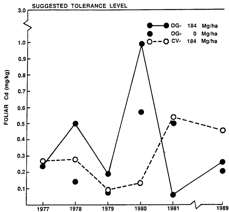
Figure 5. Mean foliar concentration of Cd in orchardgrass and crownvetch collected from the control and sludge-amended plots.
