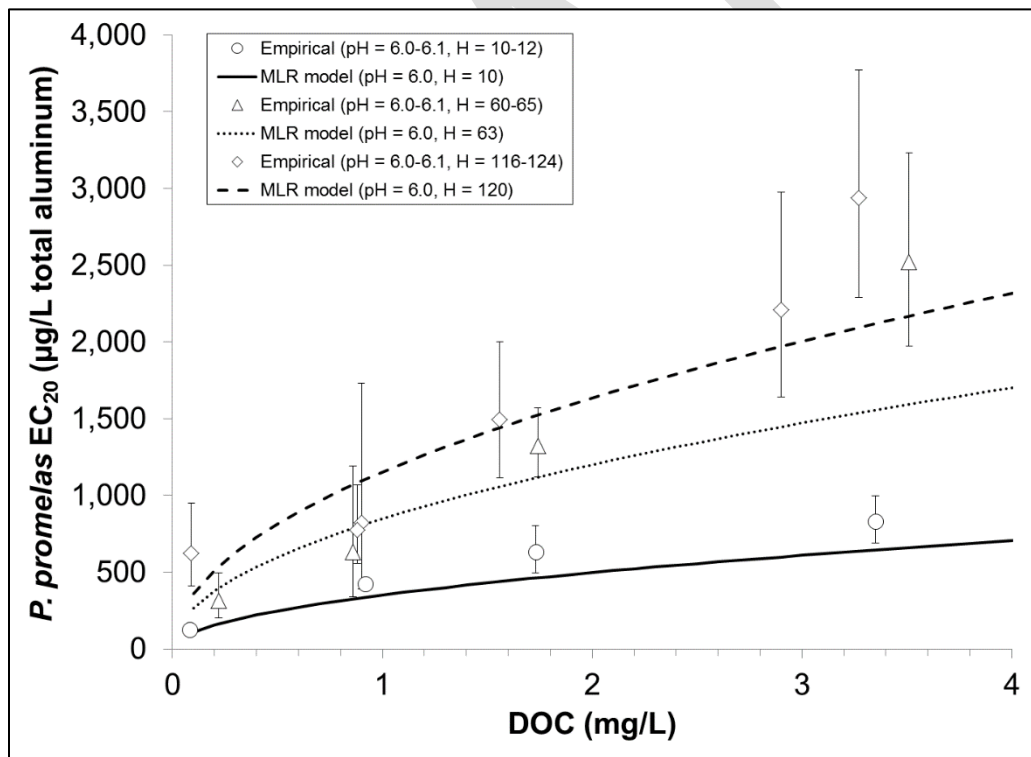
Figure 6. Observed and MLR-Predicted Aluminum EC_{20} s ( \pm 95\% CLs) for P. promelas where DOC was Varied.
