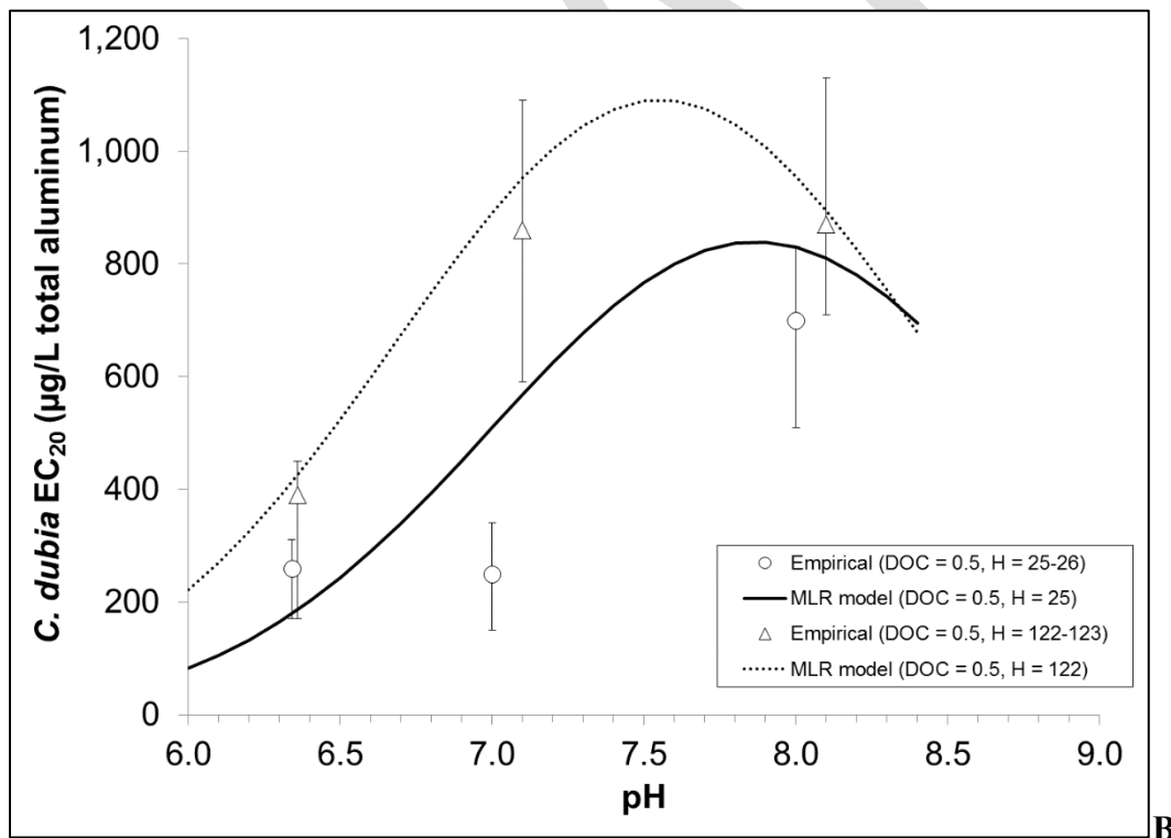
Figure 4. Observed and MLR-Predicted Aluminum EC 20 s ( \pm 95\% CLs) for C. dubia where DOC or pH was Varied.
