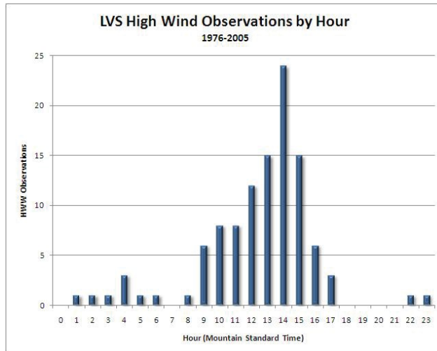
Figure 17. Frequency of high wind events by season (left) and by hour (right) at Las Vegas Airport.
