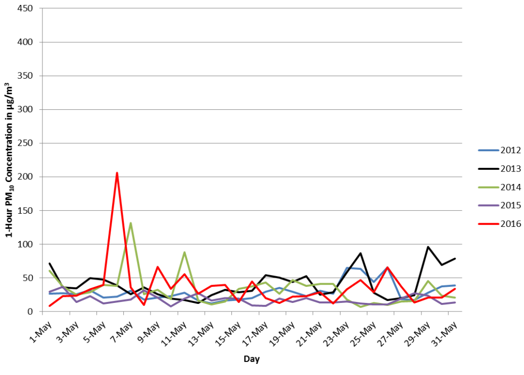
Comparison of 24-Hour Concentration results South Valley Site for the month of May for years 2012-2016
