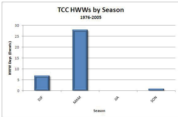
Figure 19. Frequency of high wind events by season (left) and by hour (right) at Tucumcari Airport.
