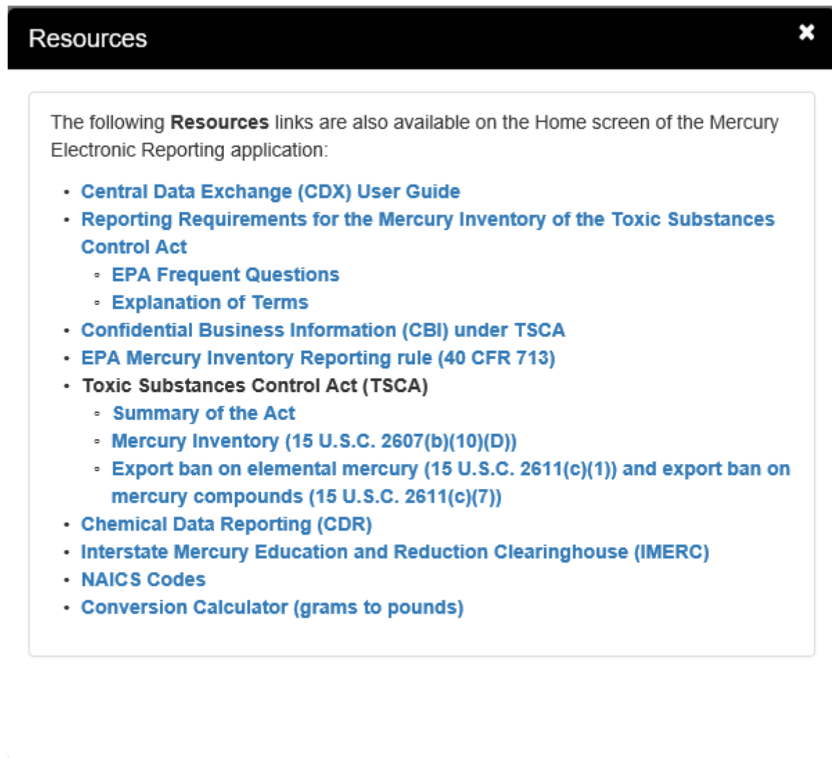
Exhibit 3-11 Resources Window
