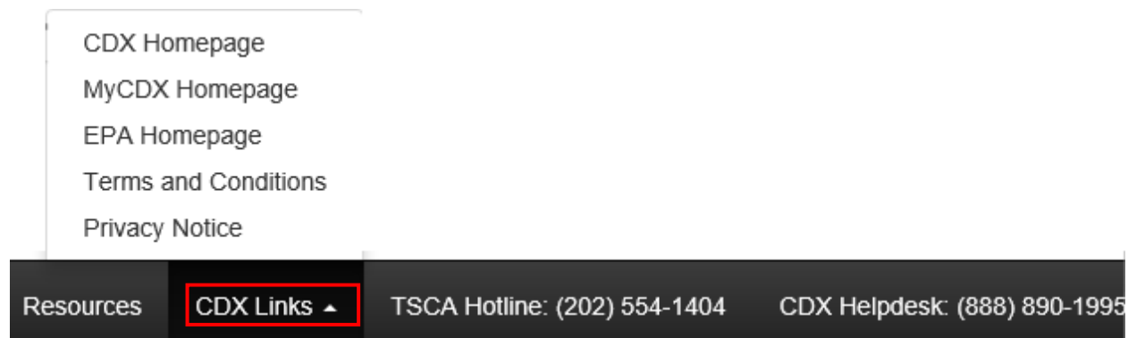
Exhibit 3-12 CDX Links
