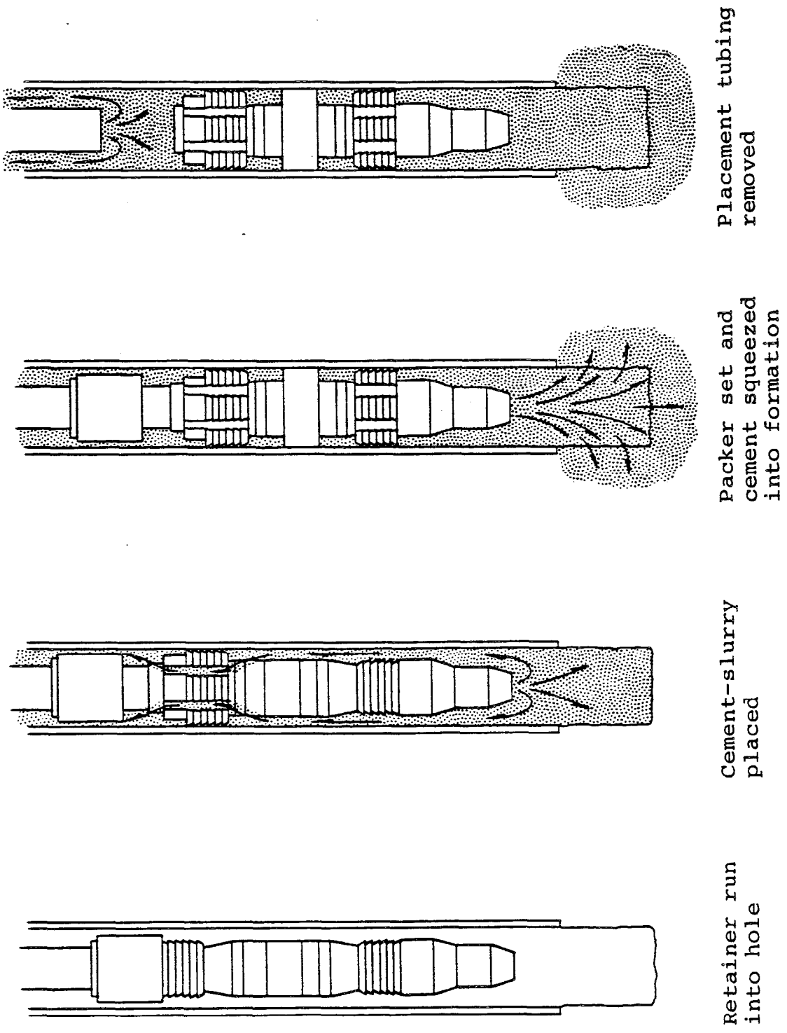
Figure 3. Principles of Retainer Method
