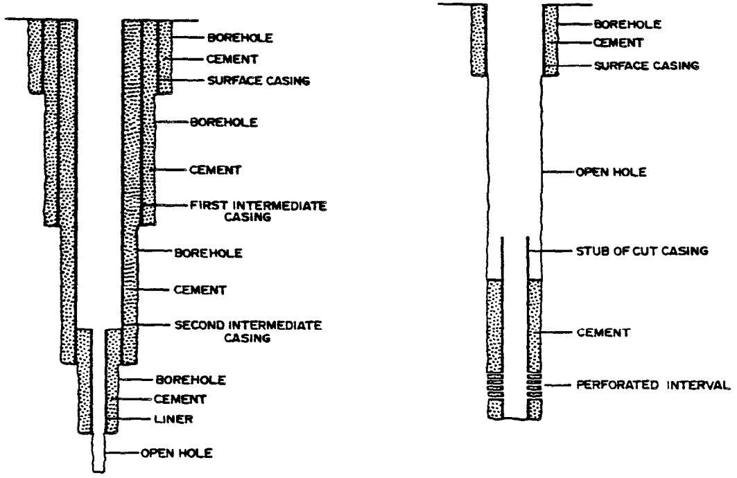
Figure 1. Common well configuration after well preparation
