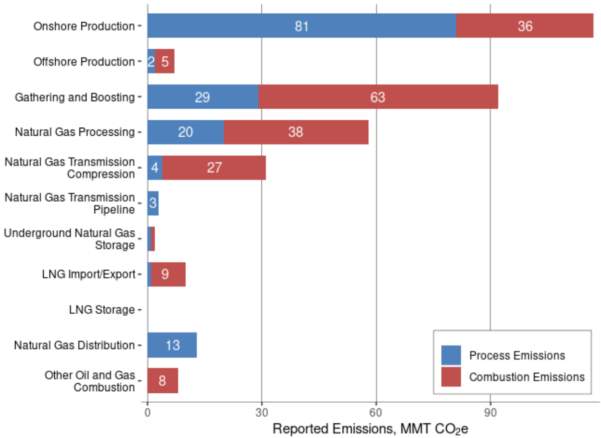
Figure 3: 2019 Reported Combustion and Process Emissions
