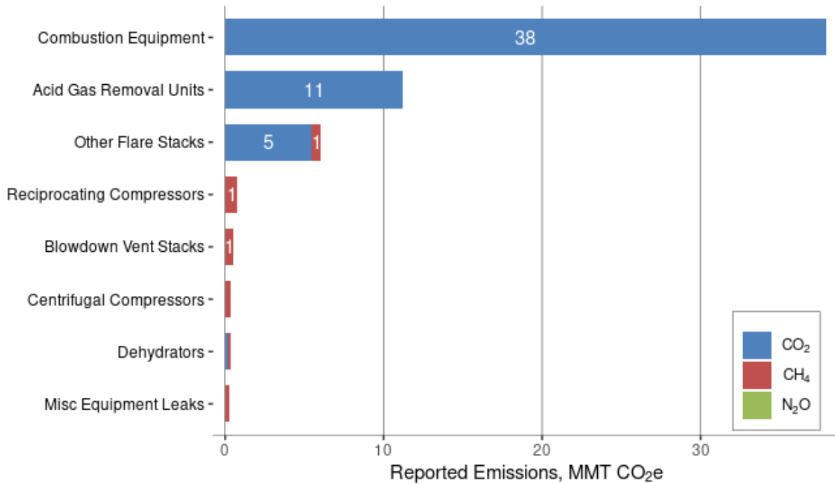
Figure 11: 2019 Natural Gas Processing: Top Reported Emission Sources
