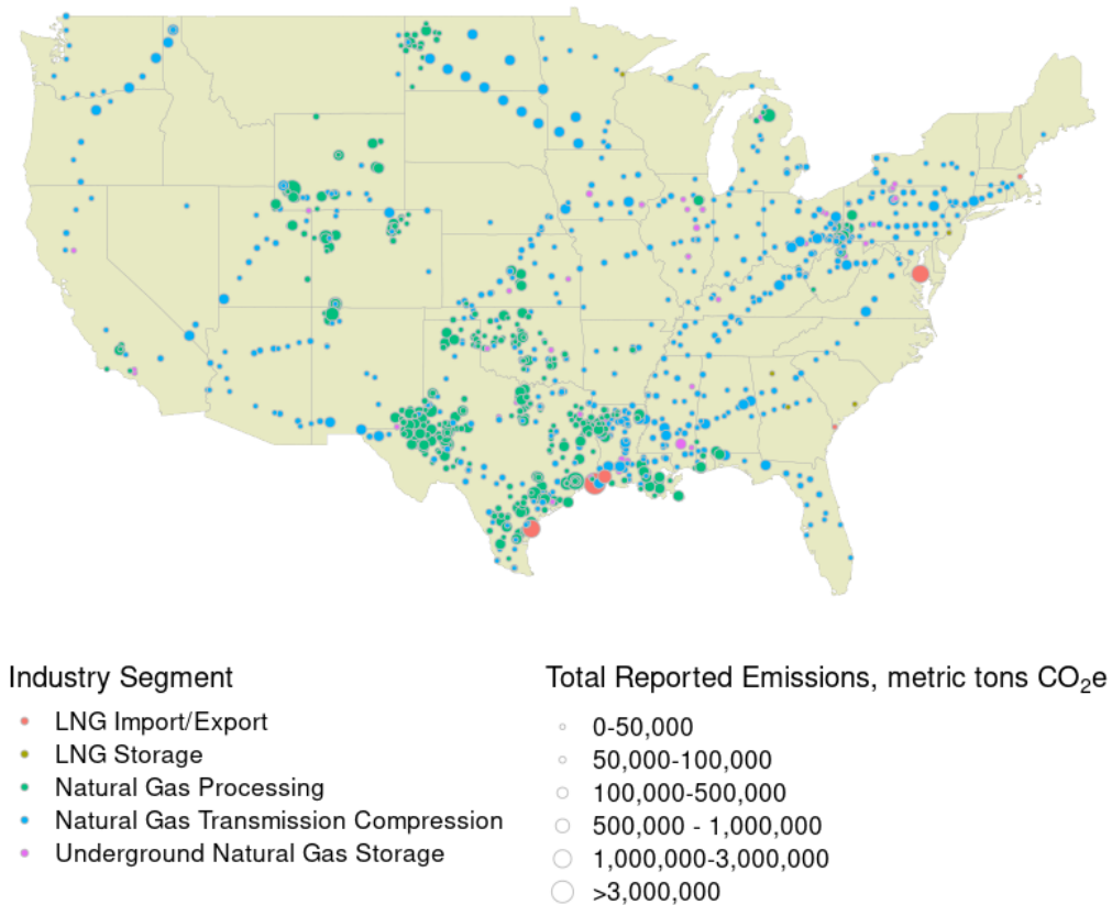
Figure 15: 2019 Facility Locations and Reported Emissions by Industry Sectors (CO 2 e)
