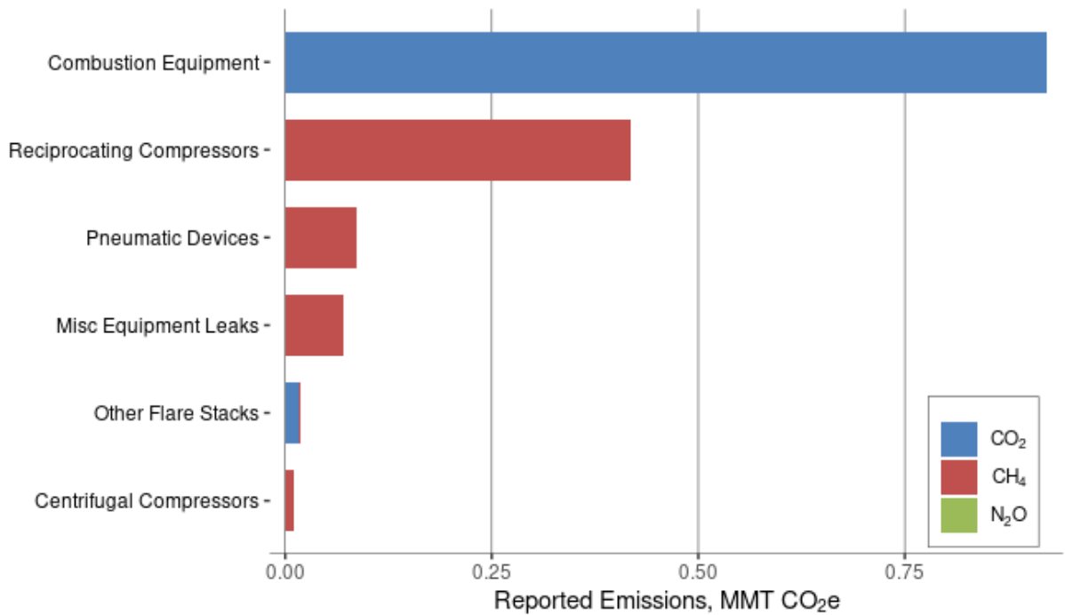
Figure 13: 2019 Underground Natural Gas Storage: Top Reported Emission Sources
