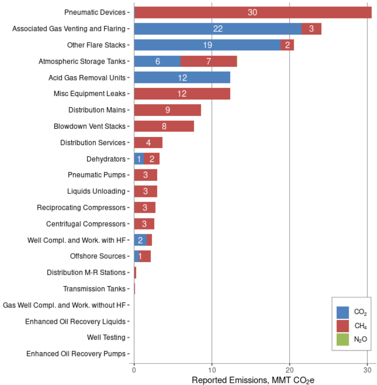
Figure 4: 2019 Reported Process Emission Sources
