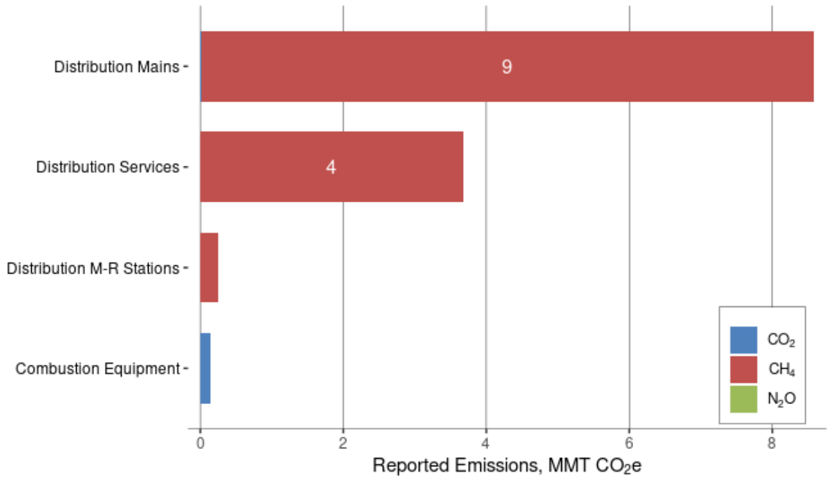
Figure 14: 2019 Natural Gas Distribution: Top Reported Emission Sources
