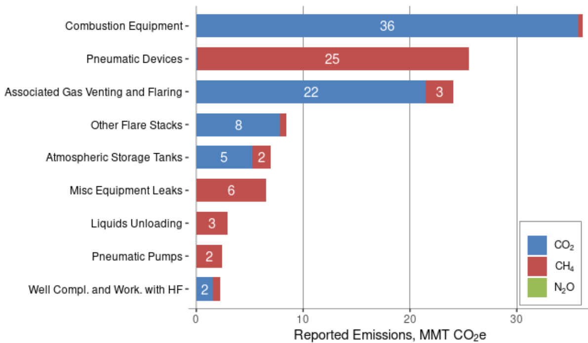
Figure 5: 2019 Onshore Production: Top Reported Emission Sources
