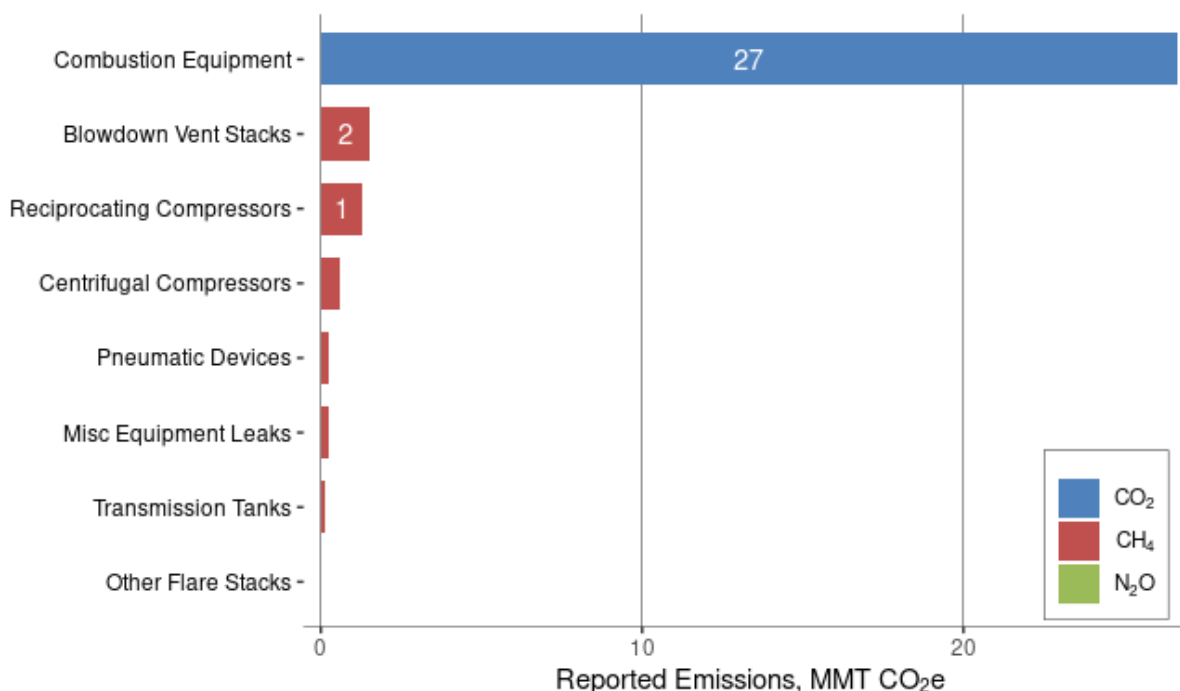
Figure 12: 2019 Natural Gas Transmission Compression: Top Reported Emission Sources
