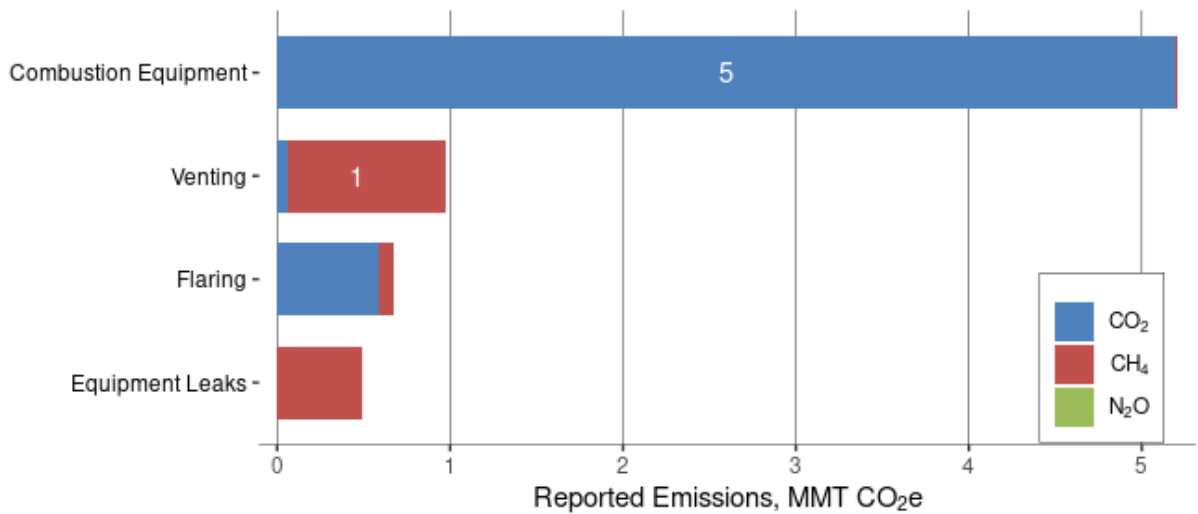
Figure 8: 2019 Offshore Production: Top Reported Emission Sources
