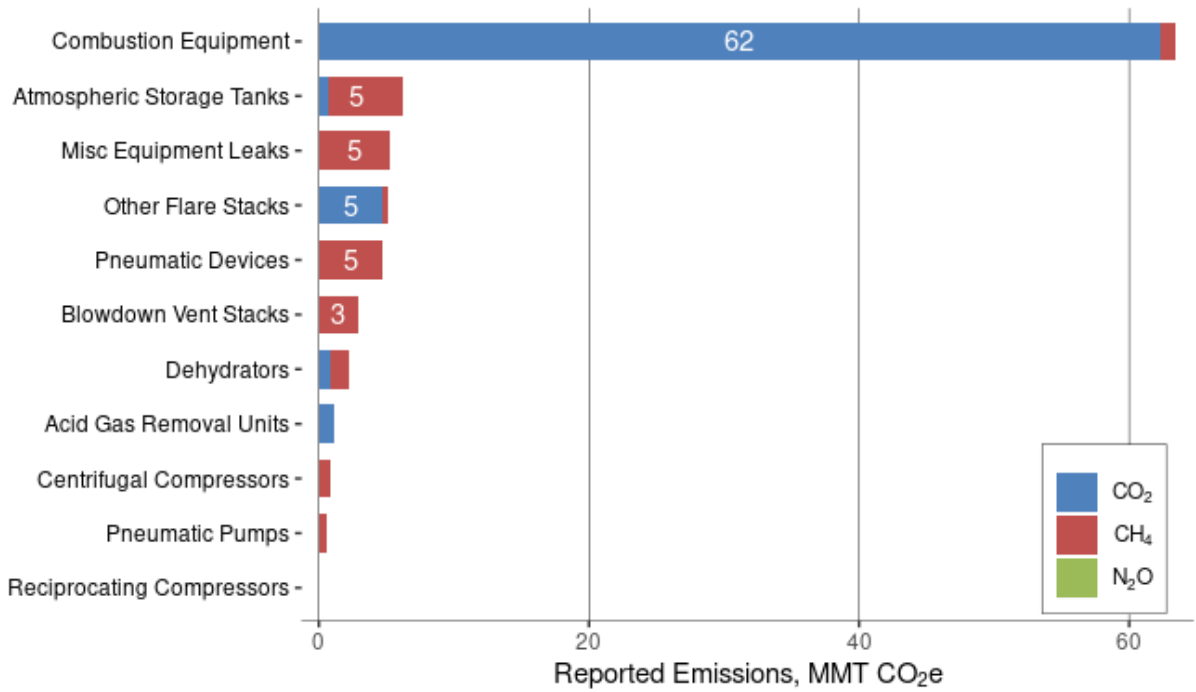
Figure 9: 2019 Gathering and Boosting: Top Reported Emission Sources
