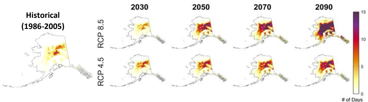
Figure 1.10. Number of Days above 80°F across Alaska (Average across the Two SNAP GCMs)
