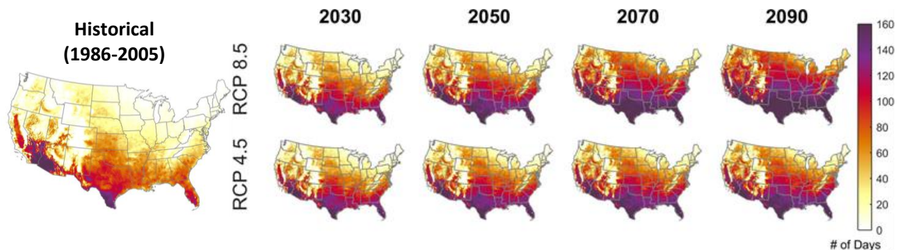
Figure 1.9. Number of Days above 90°F across the Contiguous U.S. (Average across the Five LOCA GCMs)
