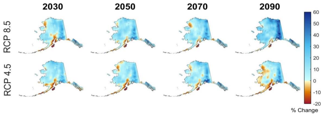
Figure 1.14. Percent Change from Reference Period in Maximum Monthly Precipitation across Alaska (Average across the Two SNAP GCMs)
