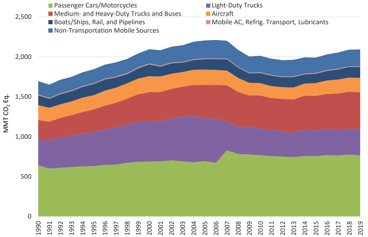
Figure A-4: Domestic Greenhouse Gas Emissions by Mode and Vehicle Type, 1990 to 2019
