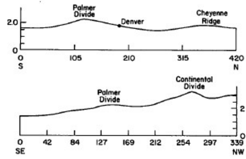
Figure 17. Topography of eastern Colorado 20
