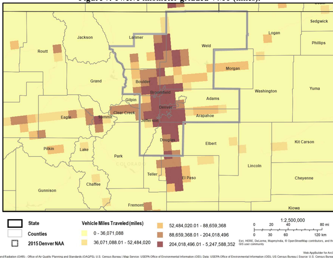
Figure 7. Twelve kilometer gridded VMT (miles).
