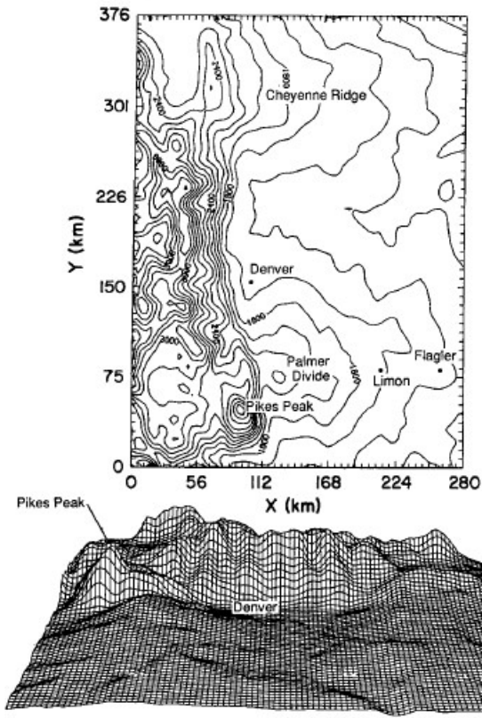
Figure 17. Topography of eastern Colorado 20
