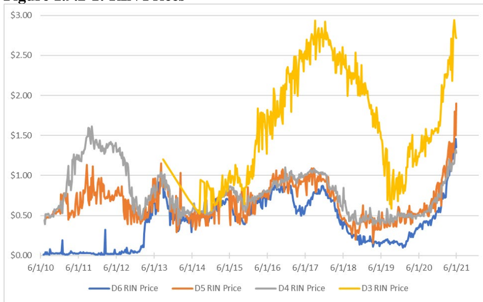
Figure 1.9.2-1: RIN Prices
