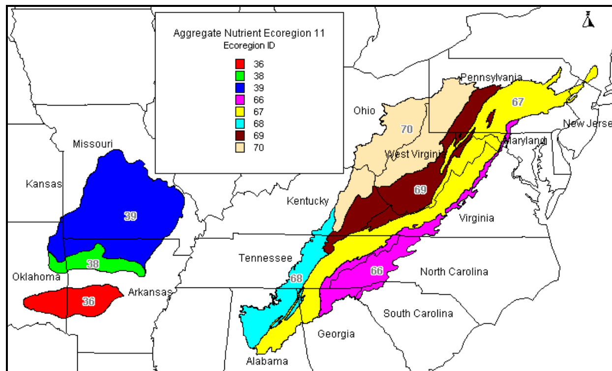
Figure 2. Ecoregion XI with level III ecoregions shown
