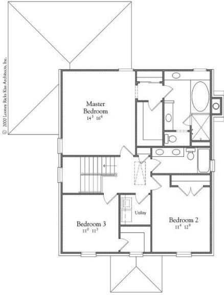
Second Floor Plan - 1,015 Sq. Ft.
