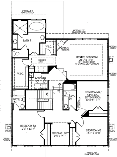
UPPER LEVEL PLAN (Elevation A)
