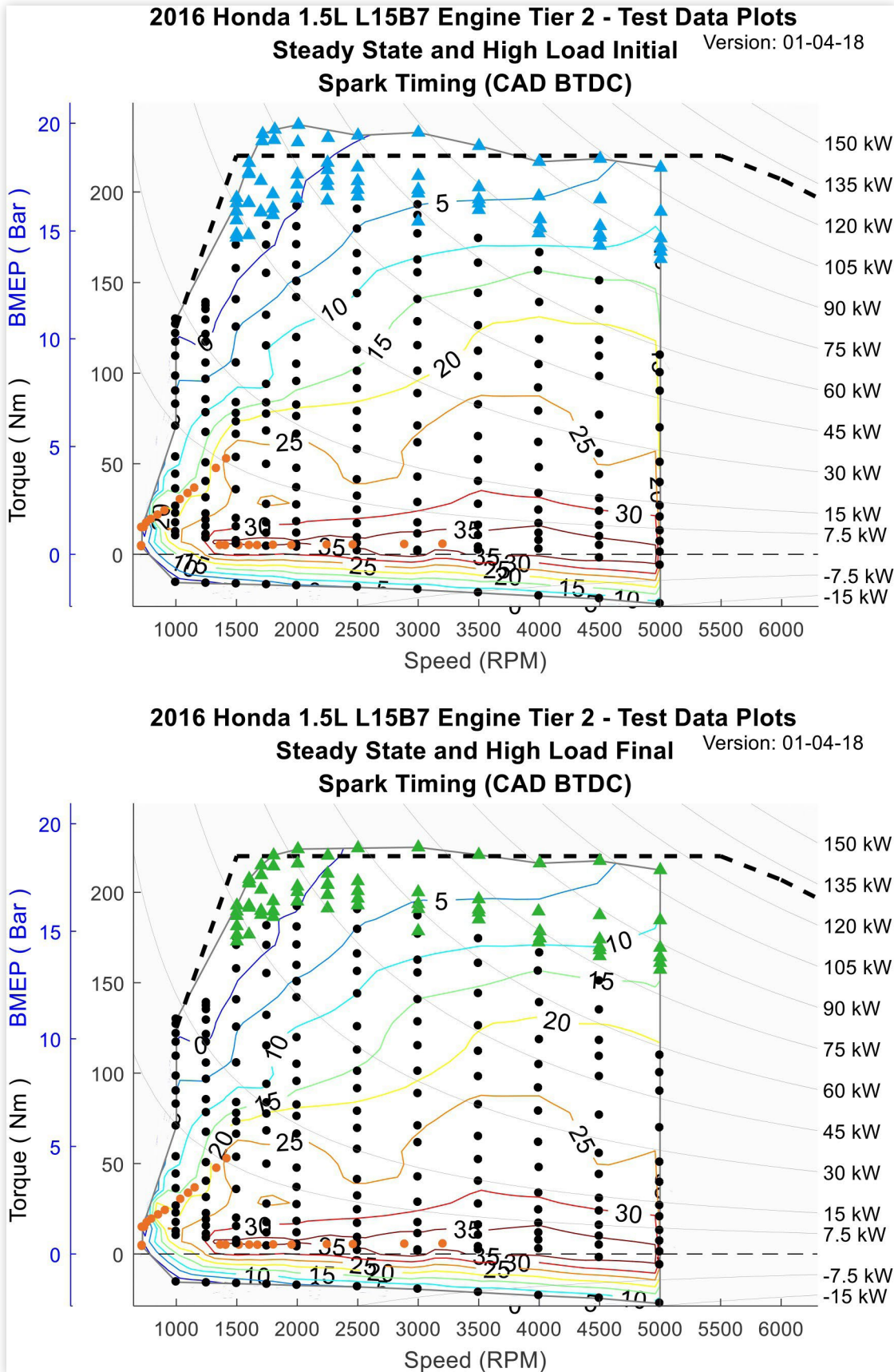
FIGURE A8 Steady-State and High Load Initial and Final Spark Timing Maps for the 2016 Honda 1.5-liter L15B7 Engine.
