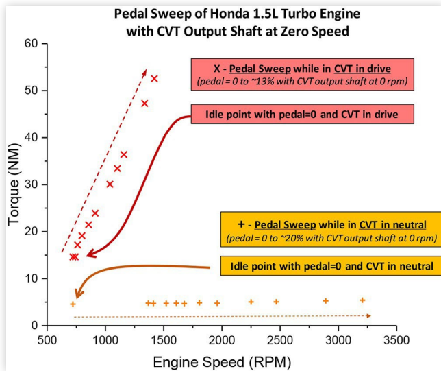
FIGURE 11 Test Phase 3 with Idle-Low Loading.
