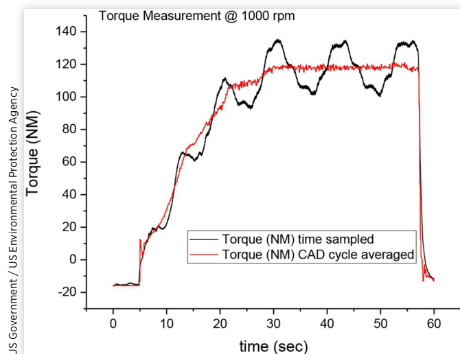
FIGURE 4 Engine Torque Measurement Load Sweep.
