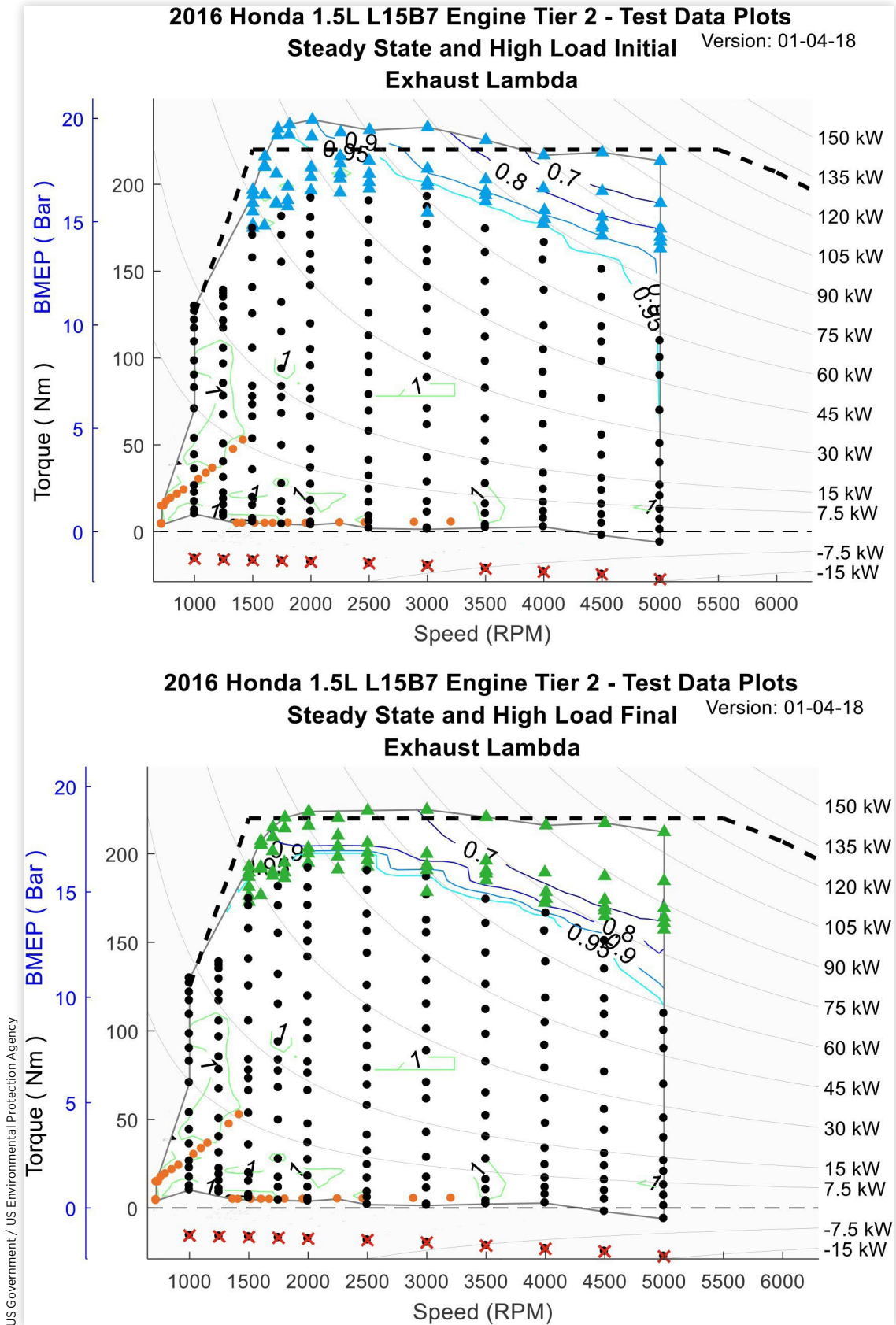
FIGURE A3 Steady-State and High Load Initial and Final Exhaust Lambda Maps for the 2016 Honda 1.5-liter L15B7 Engine.
