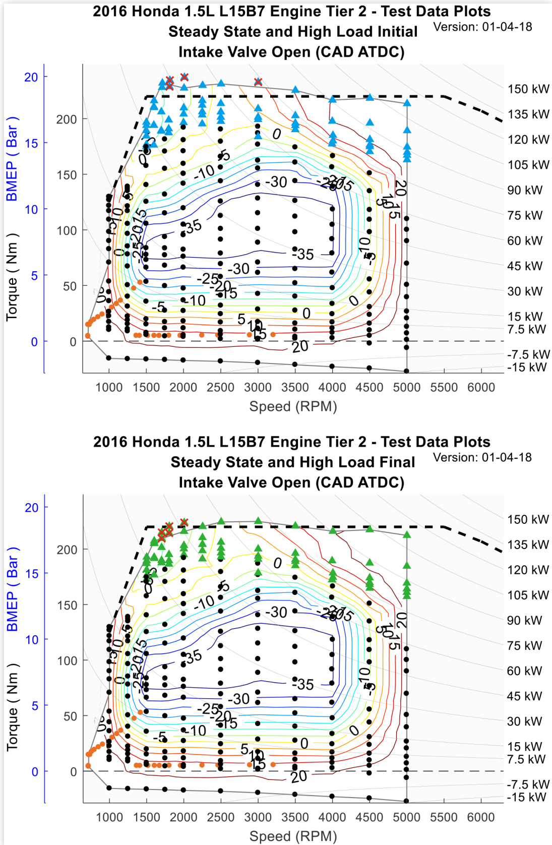
FIGURE A6 Steady-State and High Load Initial and Final Intake Cam Phase Maps for the 2016 Honda 1.5-liter L15B7 Engine.
