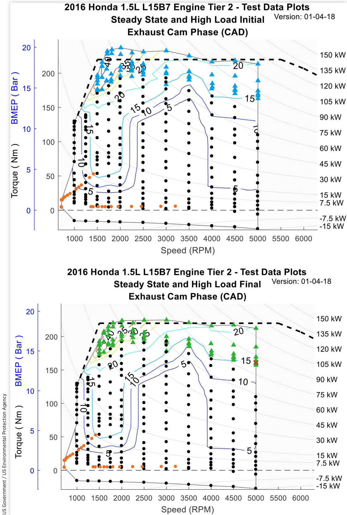
FIGURE A5 Steady-State and High Load Initial and Final Exhaust Cam Phase Maps for the 2016 Honda 1.5-liter L15B7 Engine.
