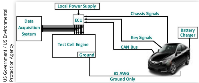
FIGURE 1 Vehicle and engine tethered wire harness.
