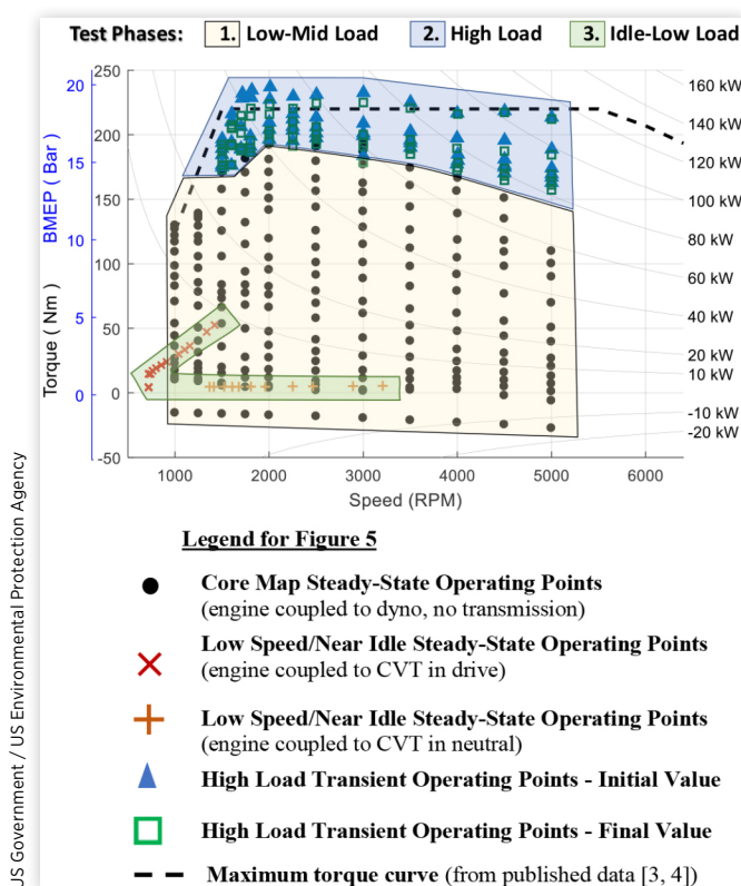
FIGURE 5 Engine Mapping Test Data Points from benchmarking 2016 Honda 1.5-liter L15B7 using Tier 2 Test Fuel.
