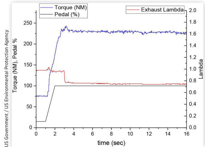
FIGURE 6 Example of data collected during Transient test.
