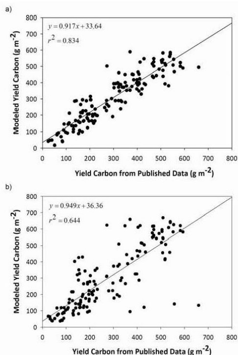
Figure A-9: Modeled versus measured net primary production ( \text{g C m}^{-2} )
