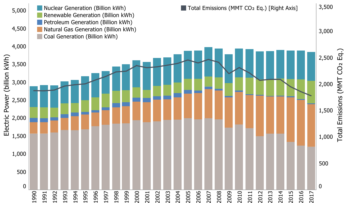
Figure 2-9: Electric Power Generation (Billion kWh) and Emissions (MMT CO 2 Eq.)
