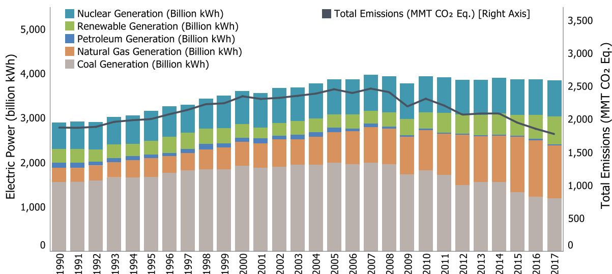
Figure ES-8: Electric Power Generation (Billion kWh) and Emissions (MMT CO 2 Eq.)
