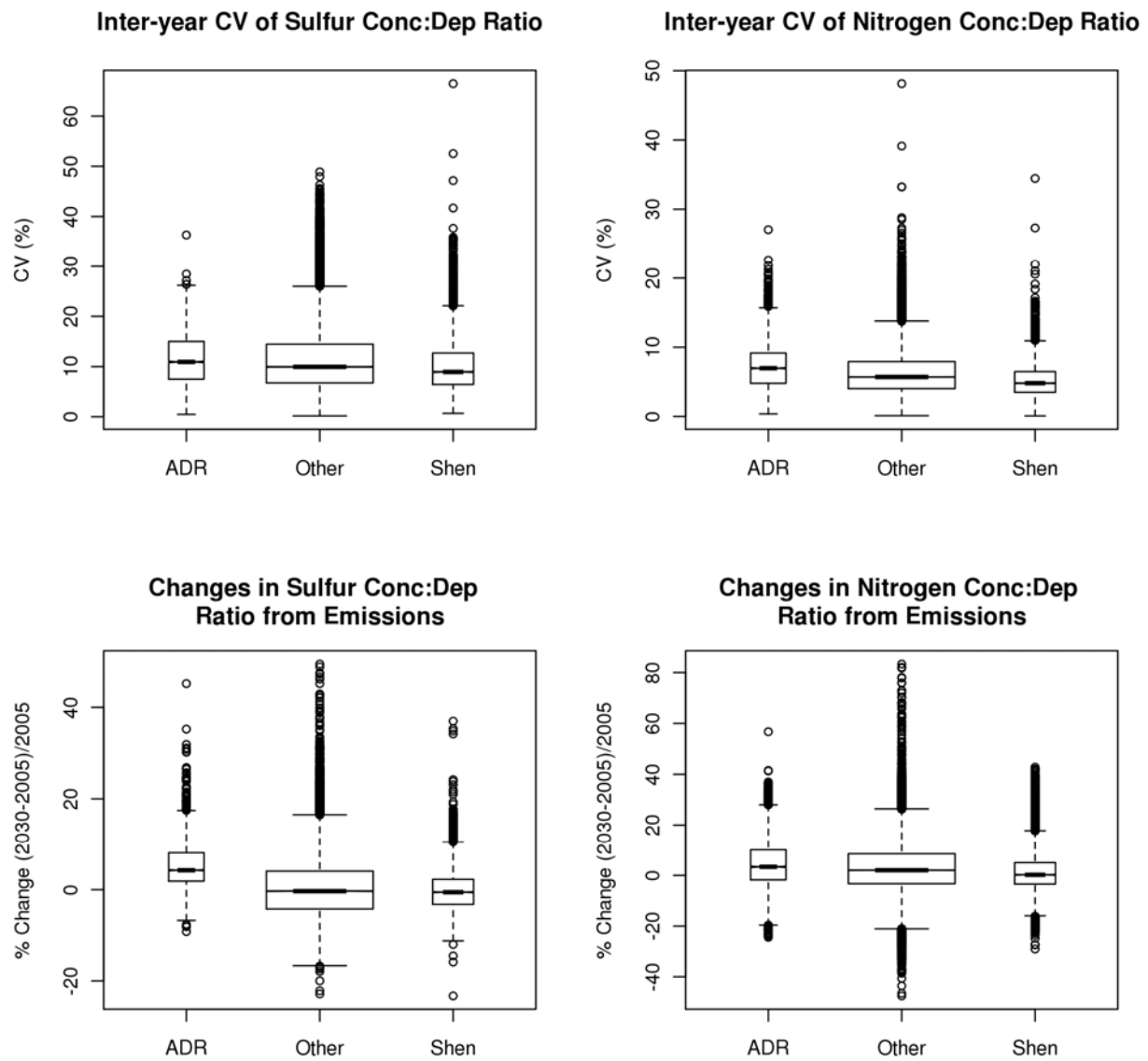
1 Figure F-16. Summary of inter-annual and emissions sensitivity variability of sulfur and 2 nitrogen deposition transference ratios.
