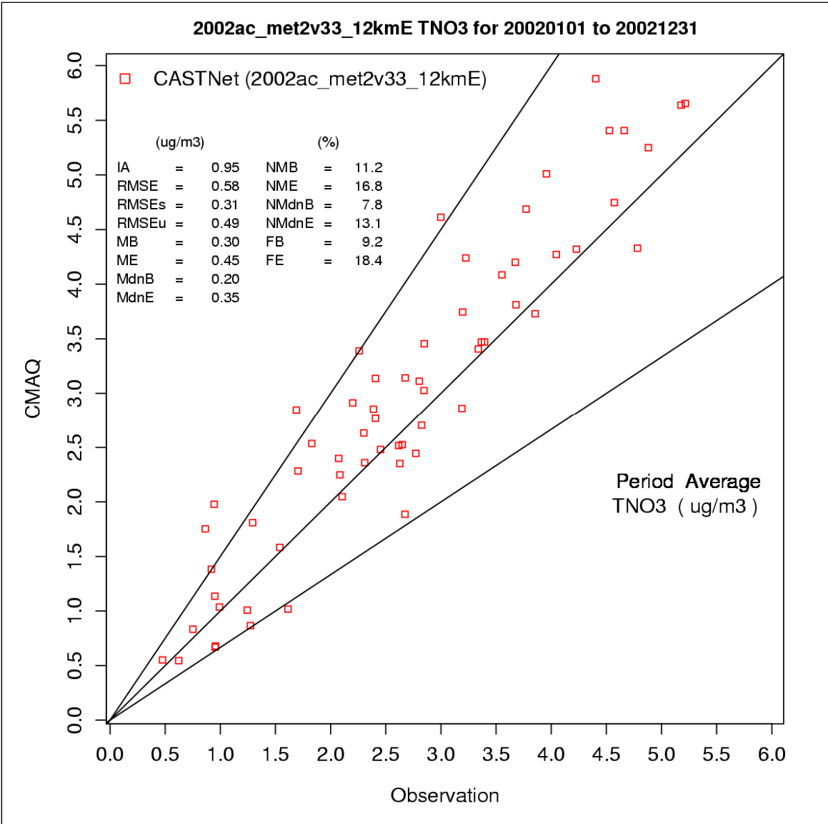
1 2 Figure F-3 2002 CMAQv4.6 annual average TNO 3 predicted concentrations versus 3 observations at CASTNet sites in the eastern domain (note, units are in actual mass for NO 3 , 4 including oxygen). 5
