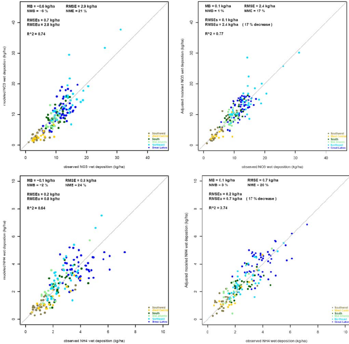
2 Figure F-13 Unadjusted (left) and PRISM and bias (right) adjusted CMAQ annual wet 3 deposition of nitrate (top) and ammonium (bottom) (note, units are in actual mass for NH 4 and 4 NH 3 , including hydrogen).
