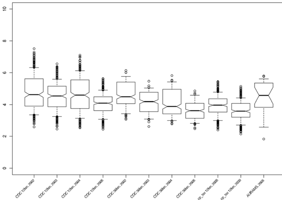
Figure F-21. Modeled generated T SOx ratios in the Adirondacks area showing CMAQ 12 and 36 km values 2002 – 2005 and AURAMS 2005.
