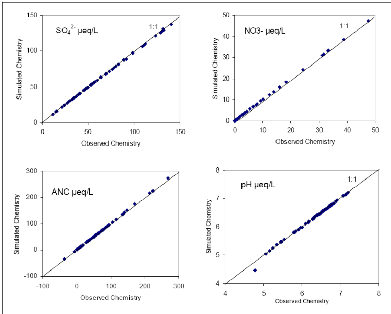
1 2 Figure F-23. Simulated versus observed annual average surface water SO 4 2- , NO 3 - , ANC, and 3 pH during the model calibration period for each of the 60 streams in the Shenandoah Case Study 4 AreF. The black line is the 1:1 line. (Source: reproduced from REA, Appendix 4, Figure 1.1-2) . 5
