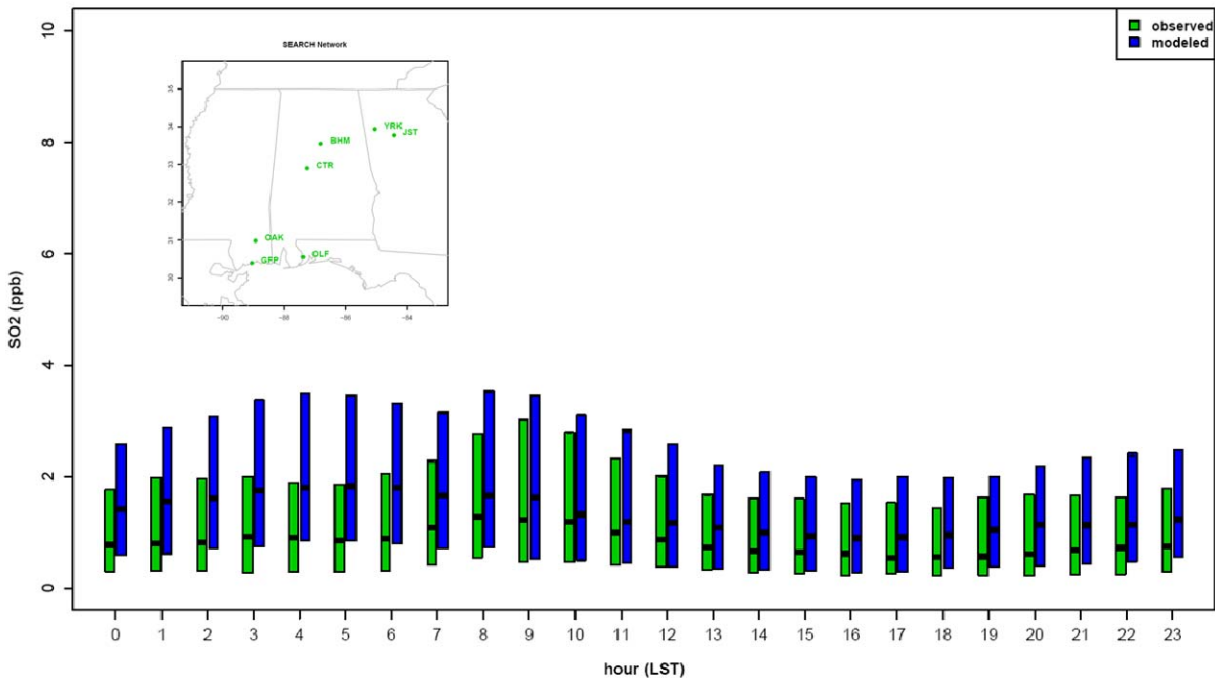
Figure F- 10. 2006 hour by hour comparisons of CMAQ and CSEARCH SO2 data at the Centerville, AL site (source, K. Foley, U.S. EPA-ORD)
