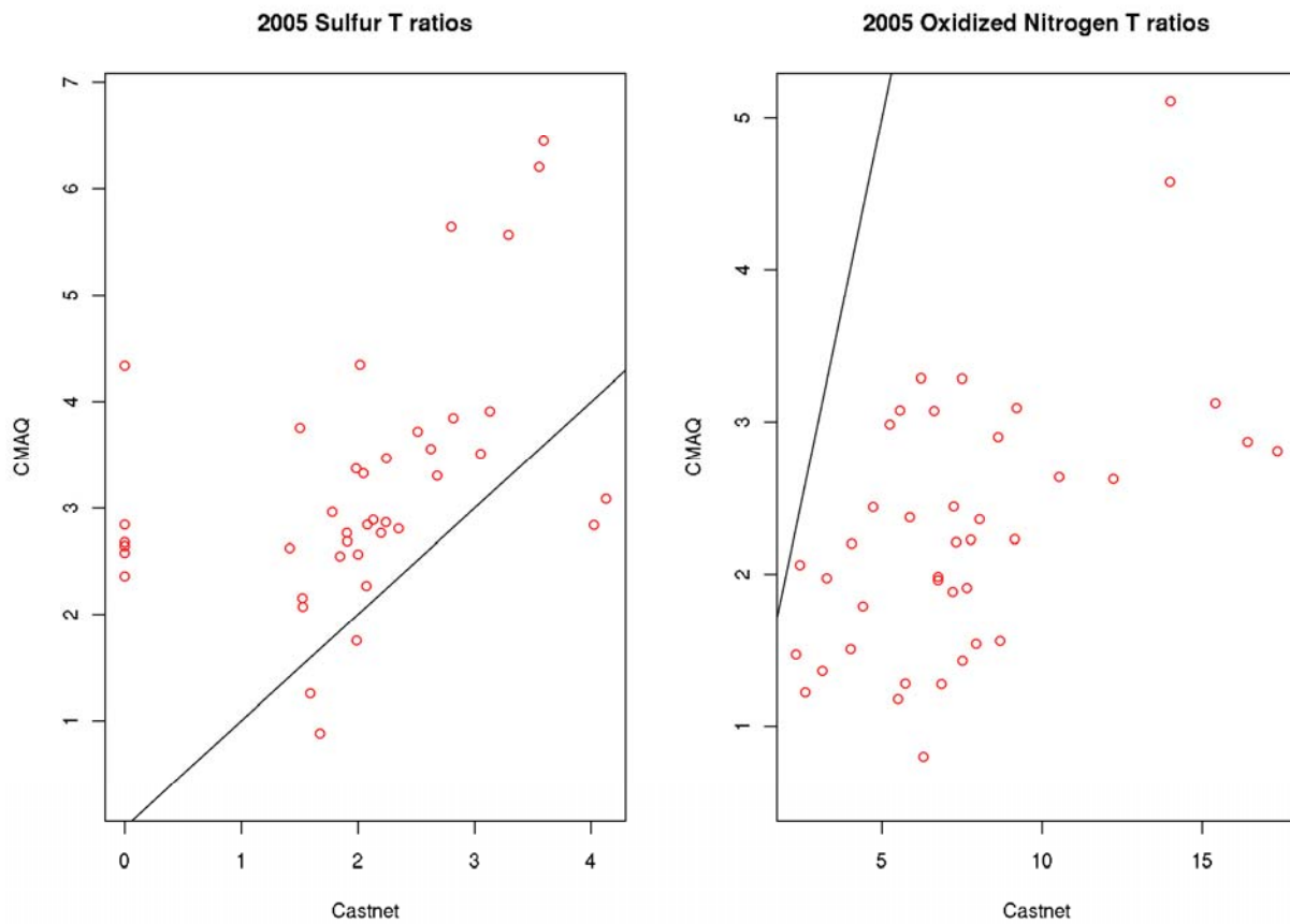
1 Figure F-17. Comparison of observation based and CMAQ derived transference ratios. Each 2 point represents an annual average at the grid cell of the CASNET station. The Observed values 3 used NADP wet precipitation data, CASTNET air quality data and modeled dry deposition 4 based on the CASTNET observations and the dry deposition model specific to CASTNET. 5
