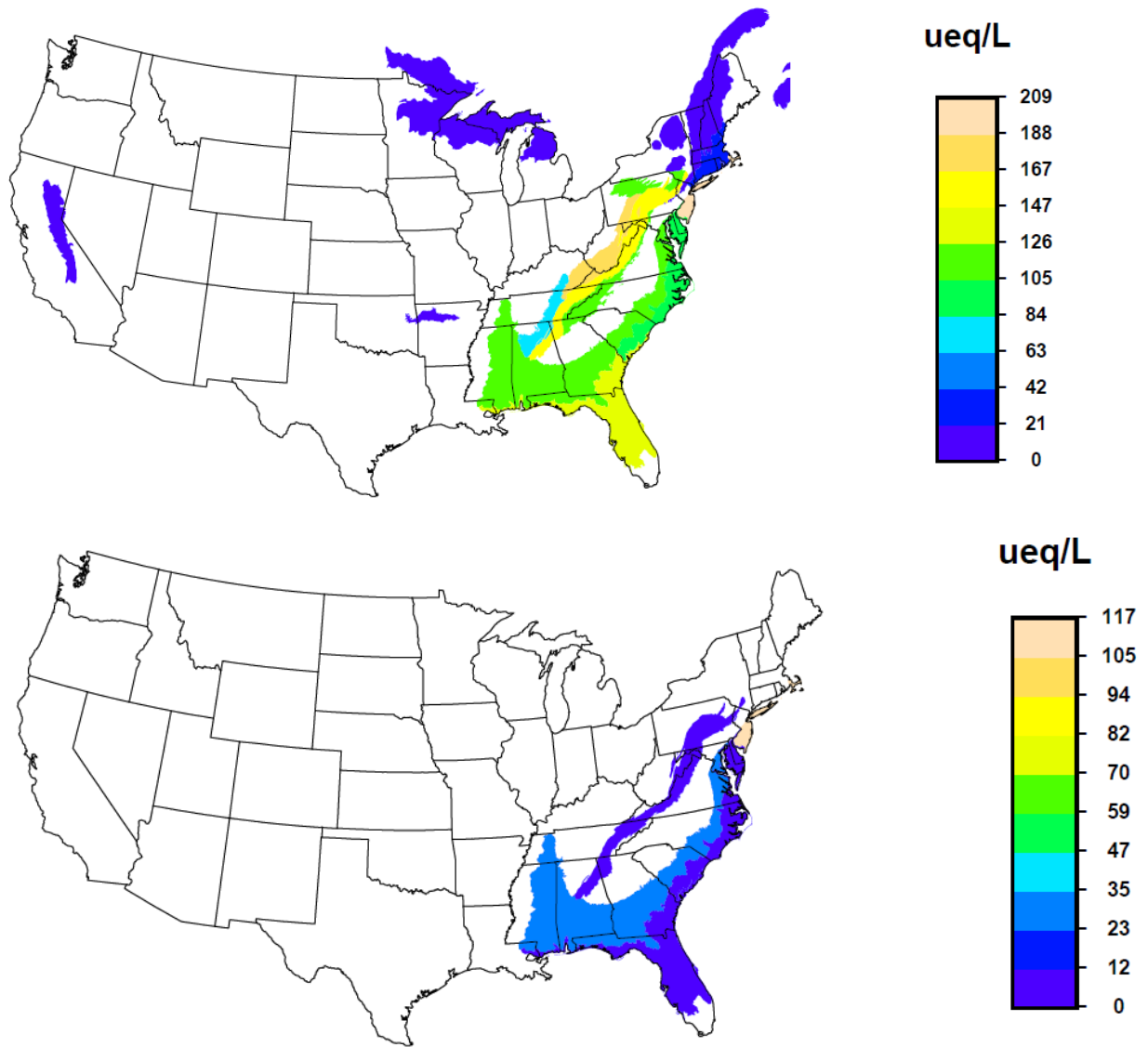
Figure D-2. Acid sensitive ecoregion level III areas likely not meeting the standard when the level = 35 µeq/L and the form is based on the 80 th percentile water body; based on CMAQ 2005 (top) and emissions sensitivity(bottom) simulations. The legend reflects the magnitude of the exceedance relative to the specified level of the standard.
