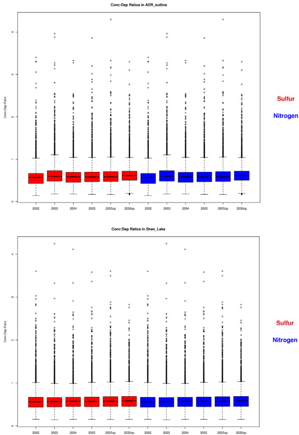
1 2 Figure F-15 Spatial and interannual variability of inverse deposition transference ratios, 1/T_{SO_x} 3 and 1/T_{NO_y} , for Adirondack (top) and Shenandoah case study areas.
