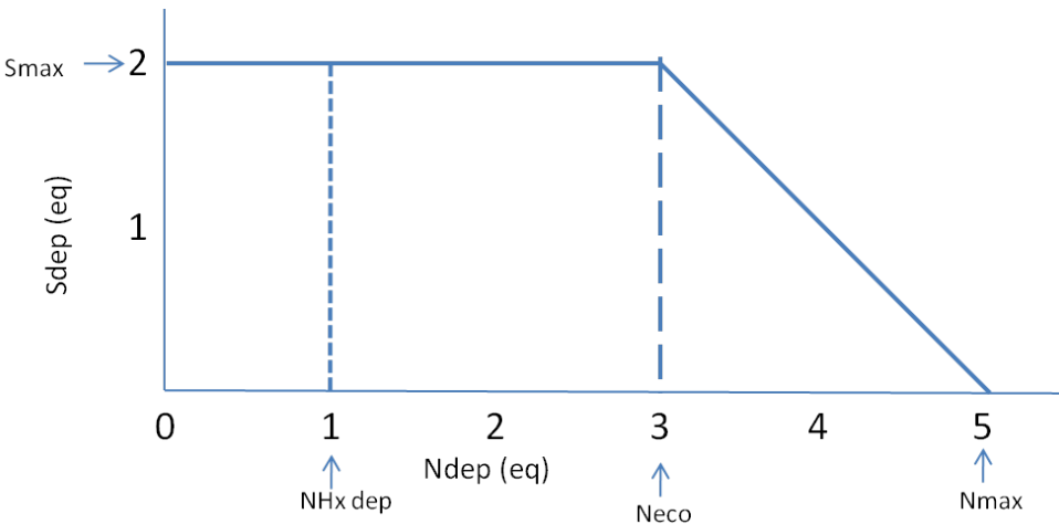
Figure 2. Hypothetical tradeoff diagram for acidifying nitrogen and sulfur deposition. The solid horizontal and diagonal lines represent the combinations of nitrogen and sulfur deposition to meet a target ANC. Deposition values within the area bounded by these lines do not exceed the target critical load and values outside the borders exceed a critical load. When all units are transformed to equivalent charge, there is a 1:1 slope in the region where nitrogen deposition exceeds Neco which illustrates the area of tradeoffs between nitrogen and sulfur deposition.
