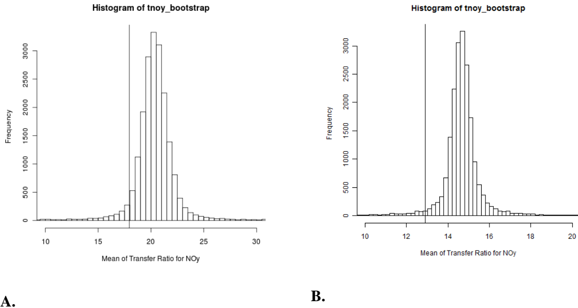
Figure G-3. Bootstrap distribution of mean nitrogen transference ratios ( T_{noy} ) for Regions 5.3.1 (A) and 9.3.3 (B)
