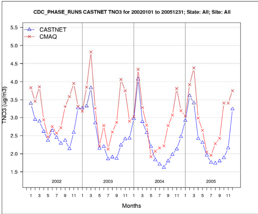
1 2 Figure F-6. 2002–2005 Domain-wide average TNO 3 predicted concentrations and 3 observations by month at CASTNet sites in the eastern domain (note, units are in actual mass for 4 NO 3 , including oxygen). 5
