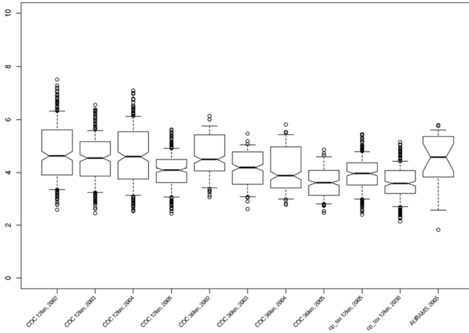
Figure F-18. Modeled generated T NOy ratios in the Shenadoah area showing CMAQ 12 and 36 km values 2002 – 2005 and AURAMS 2005.
