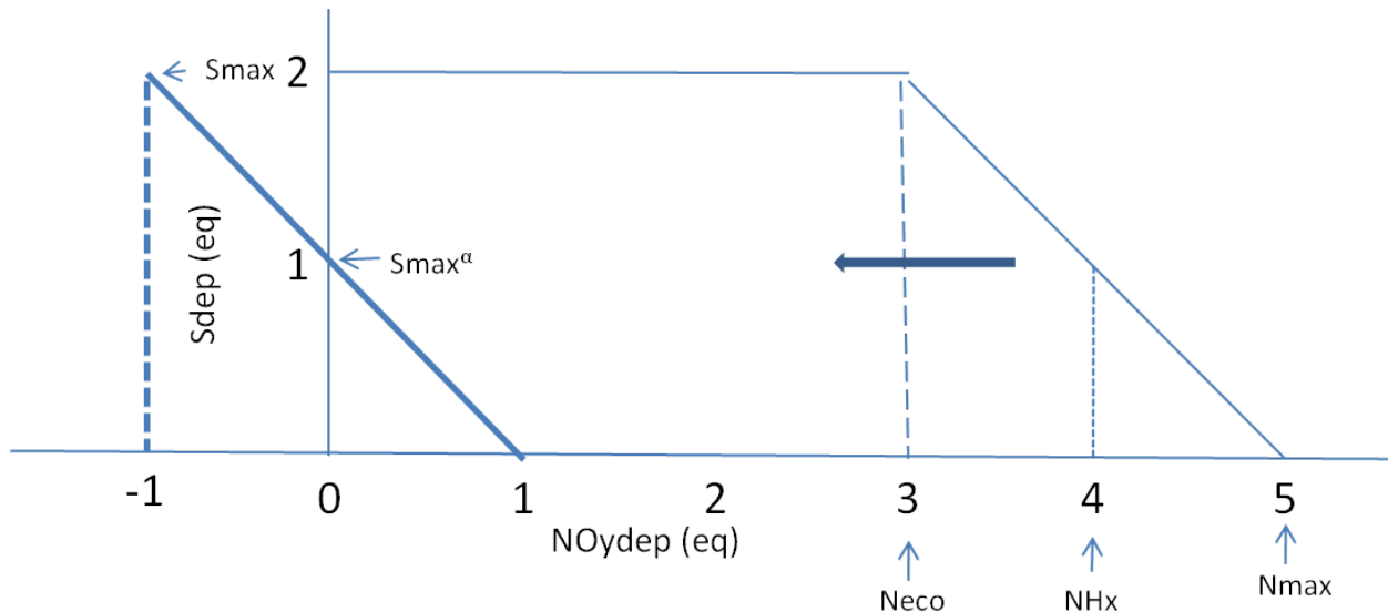
Figure 4. NOy and SOx deposition tradeoff curve for hypothetical case where NHx deposition exceeds Neco . The effect can be visualized as the system retaining a residual one equivalent unit of NHx that can not be neutralized by Neco with the consequent reduction on both allowable maximum amounts of SOx and NOy deposition.
