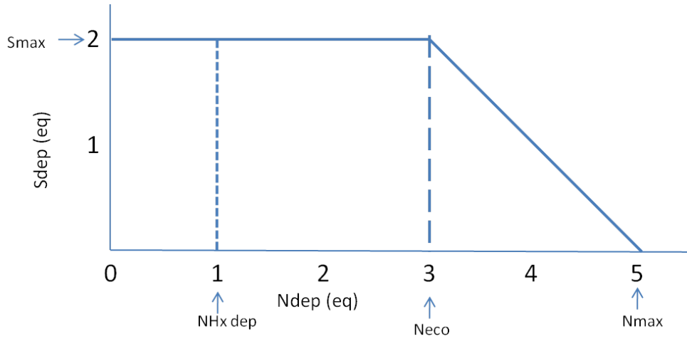
Figure D-4.1. Hypothetical tradeoff diagram for acidifying nitrogen and sulfur deposition. The solid horizontal and diagonal lines represent the combinations of nitrogen and sulfur deposition to meet a target ANC. Deposition values within the area bounded by these lines do not exceed the target critical load and values outside the borders exceed a critical load. When all units are transformed to equivalent charge, there is a 1:1 slope in the region where nitrogen deposition exceeds Neco which illustrates the area of tradeoffs between nitrogen and sulfur deposition.
