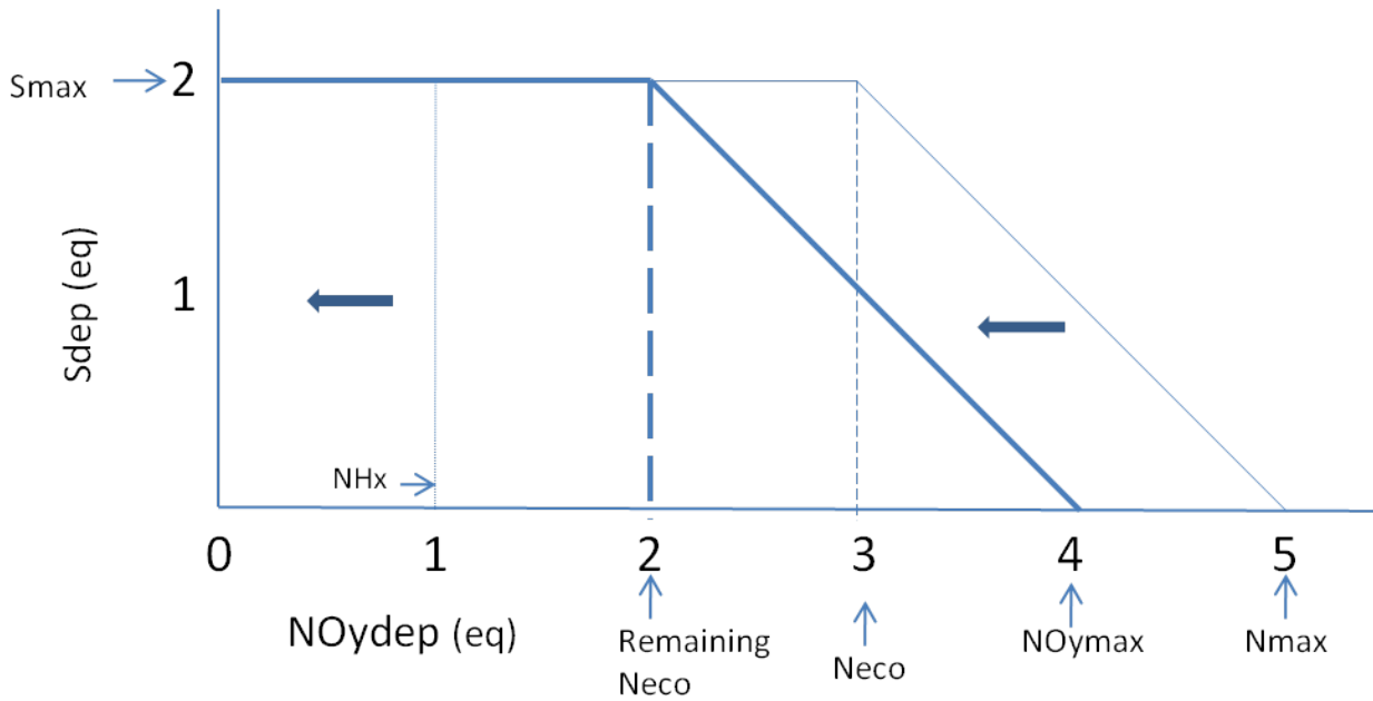
Figure D-4.1. Deposition tradeoff diagram for sulfur and the oxidized fraction of total nitrogen deposition with 1 equivalent unit of \text{NH}_x deposition removed. The removal of one equivalent unit of \text{NH}_x from figure 1 shifts the original diagram to the left and defines the amount of allowable maximum \text{NO}_y deposition, which is simply the difference between N_{\text{max}} and \text{NH}_x in Figure 7-trade1.
