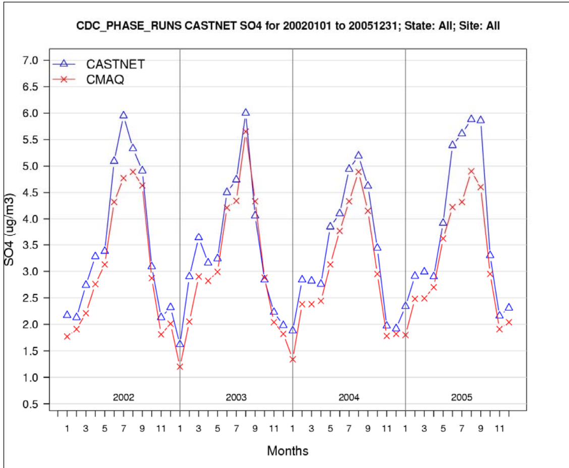
1 2 Figure F-5. 2002–2005 Domain-wide average SO 4 2- predicted concentrations and 3 observations by month at CASTNet Sites in the eastern domain (note, units are in actual mass for 4 SO 4 , including oxygen) . 5
