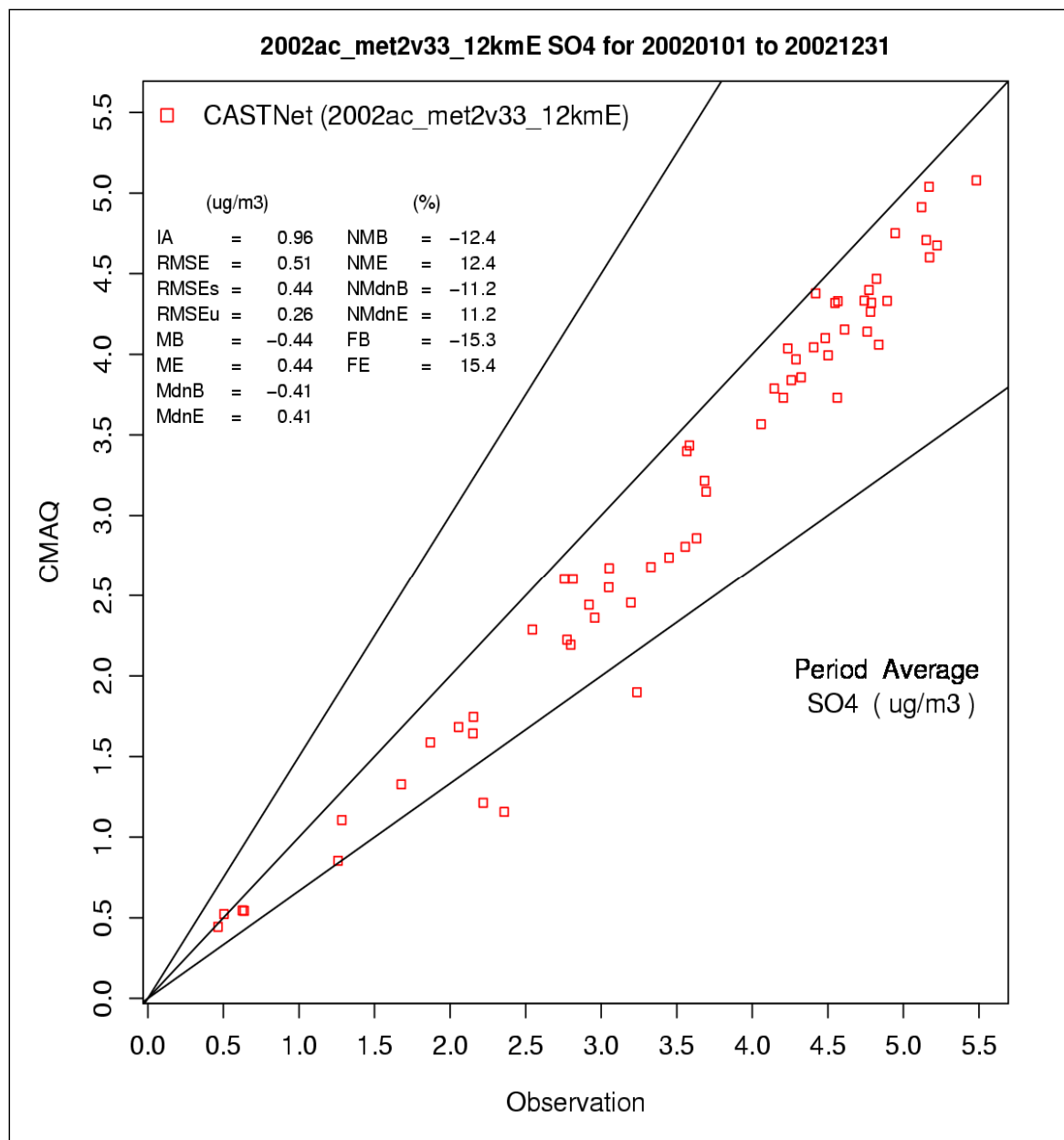
1 2 Figure F-2 2002 CMAQv4.6 annual average SO 4 2- predicted concentrations versus 3 observations at CASTNet sites in the eastern domain (note, units are in actual mass for SO 4 , 4 including oxygen). 5
