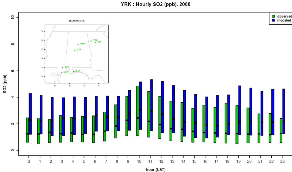
Figure F- 11. 2006 hour by hour comparisons of CMAQ and CSEARCH SO 2 data at the Yorkville, GA site (source, K. Foley, U.S. EPA-ORD)
