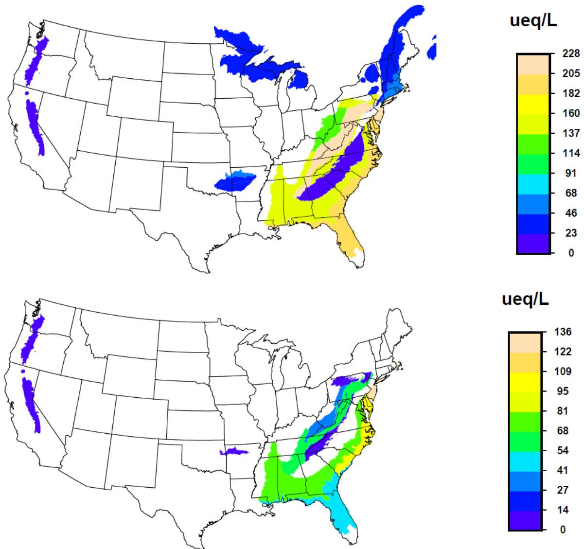
Figure D-3. Acid sensitive ecoregion level III areas likely not meeting the standard when the level = 35 µeq/L and the form is based on the 90 th percentile water body; based on CMAQ 2005 (top) and emissions sensitivity(bottom) simulations. The legend reflects the magnitude of the exceedance relative to the specified level of the standard.
