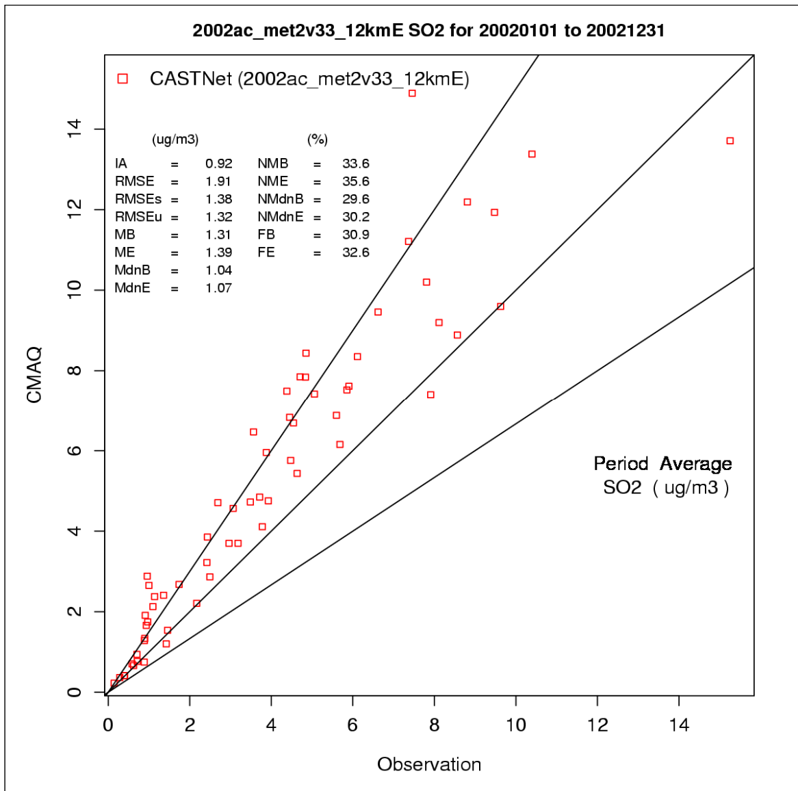
2 Figure F-1 2002 CMAQv4.6 annual average SO 2 predicted concentrations versus 3 observations at CASTNet sites in the eastern domain (note, units are in actual mass for SO 2 , 4 including oxygen).
