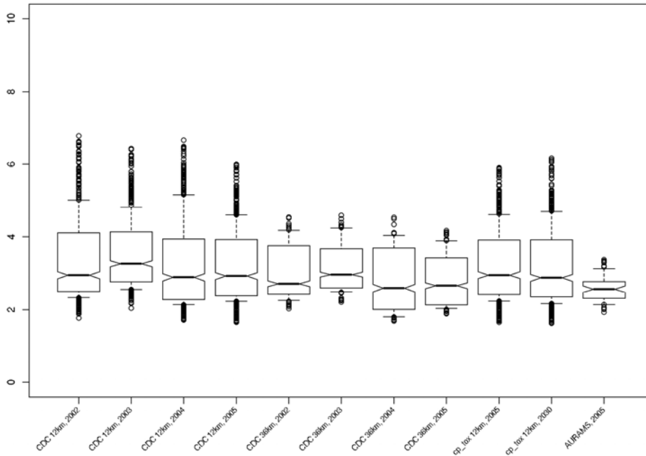
1 Figure F-20. Modeled generated T NOy ratios in the Adirondacks area showing CMAQ 12 and 36 km values 2002 – 2 2005 and AURAMS 2005.
