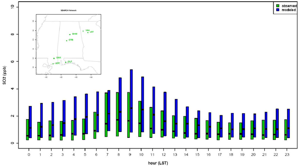
1 2 Figure F-9. 2006 hour by hour comparisons of CMAQ and SEARCH SO2 data at the Ook Grove, MS site (source, 3 K. Foley, U.S. EPA-ORD) 4
