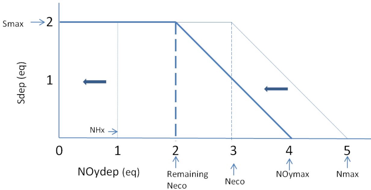
Figure 3. Deposition tradeoff diagram for sulfur and the oxidized fraction of total nitrogen deposition with 1 equivalent unit of NHx deposition removed. The removal of one equivalent unit of NHx from figure 1 shifts the original diagram to the left and defines the amount of allowable maximum NOy deposition, which is simply the difference between Nmax and NHx in Figure 1.
