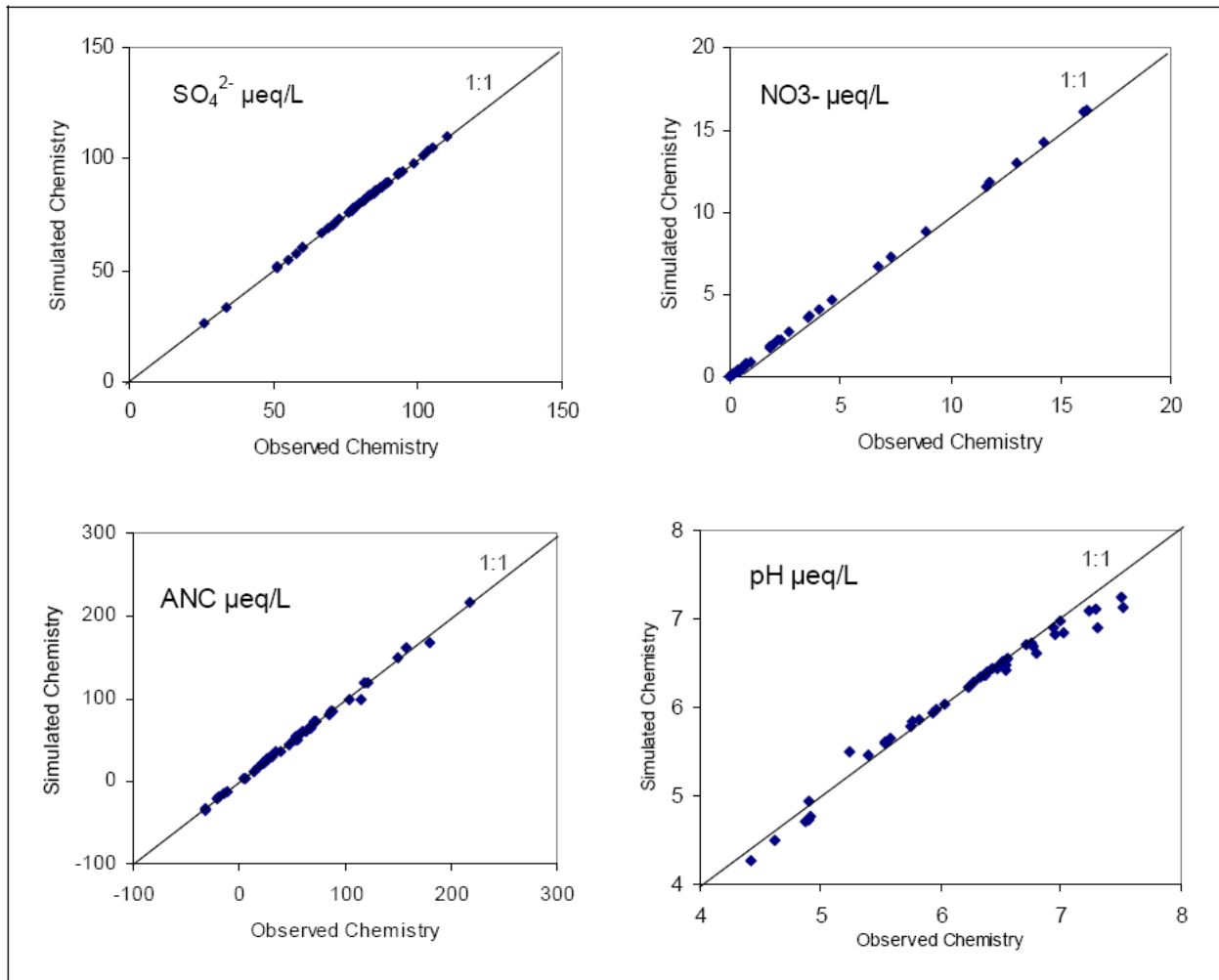
9 Figure F-22 Simulated versus observed annual average surface water SO 4 2- , NO 3 - , ANC, and 10 pH during the model calibration period for each of the 44 lakes in the Adirondacks Case Study 11 AreF. The black line is the 1:1 line. (Source: reproduced from REA, Appendix 4, Figure 1.1-1).
