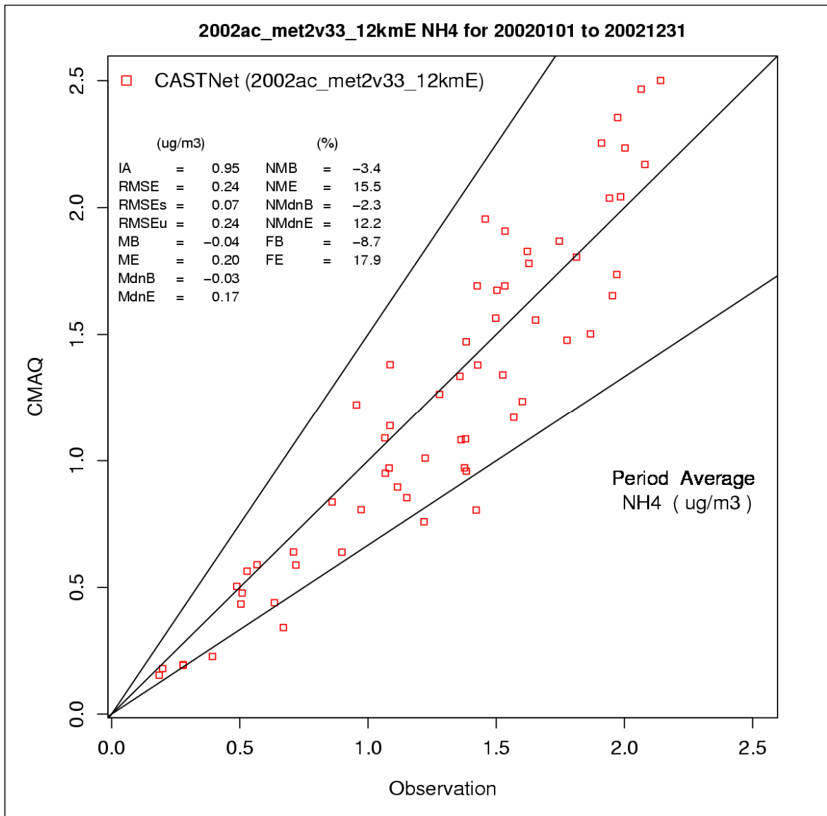
2 Figure F-4. 2002 CMAQv4.6 annual average \text{NH}_4^+ predicted concentrations versus 3 observations at CASTNet sites in the eastern domain (note, units are in actual mass for \text{NH}_4 , 4 including hydrogen). 5
