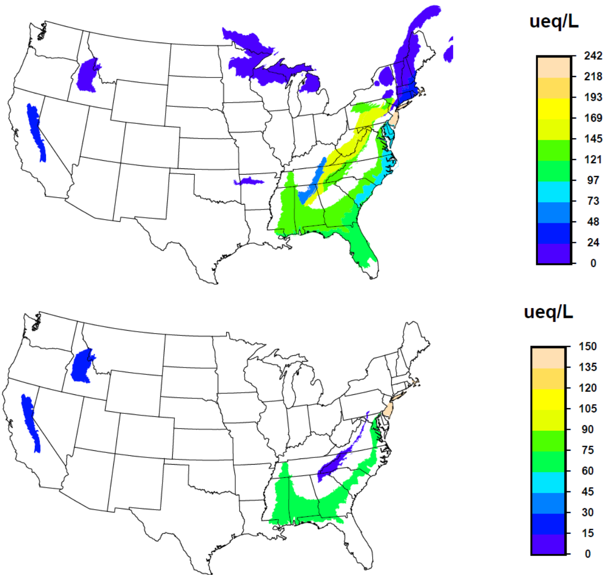
Figure D-8. Acid sensitive ecoregion level III areas likely not meeting the standard when the level = 75 \mu\text{eq/L} and the form is based on the 80 th percentile water body; based on CMAQ 2005 (top) and emissions sensitivity(bottom) simulations. The legend reflects the magnitude of the exceedance relative to the specified level of the standard.
