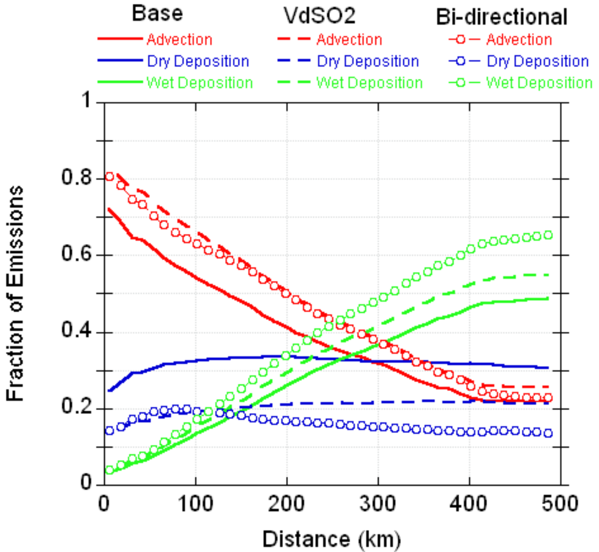
3 Figure F-14. Cumulative regional NH 3 budget of advection, wet- and dry deposition, 4 calculated for an expanding box starting at the high-emitting Sampson County NC cell (from 5 Dennis et al, 2010)
