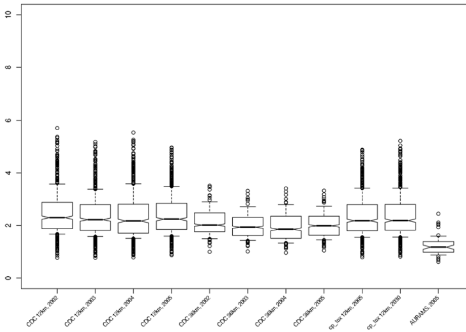
Figure F-19. Modeled generated T SOx ratios in the Shenadoah area showing CMAQ 12 and 36 km values 2002 – 2005 and AURAMS 2005.
