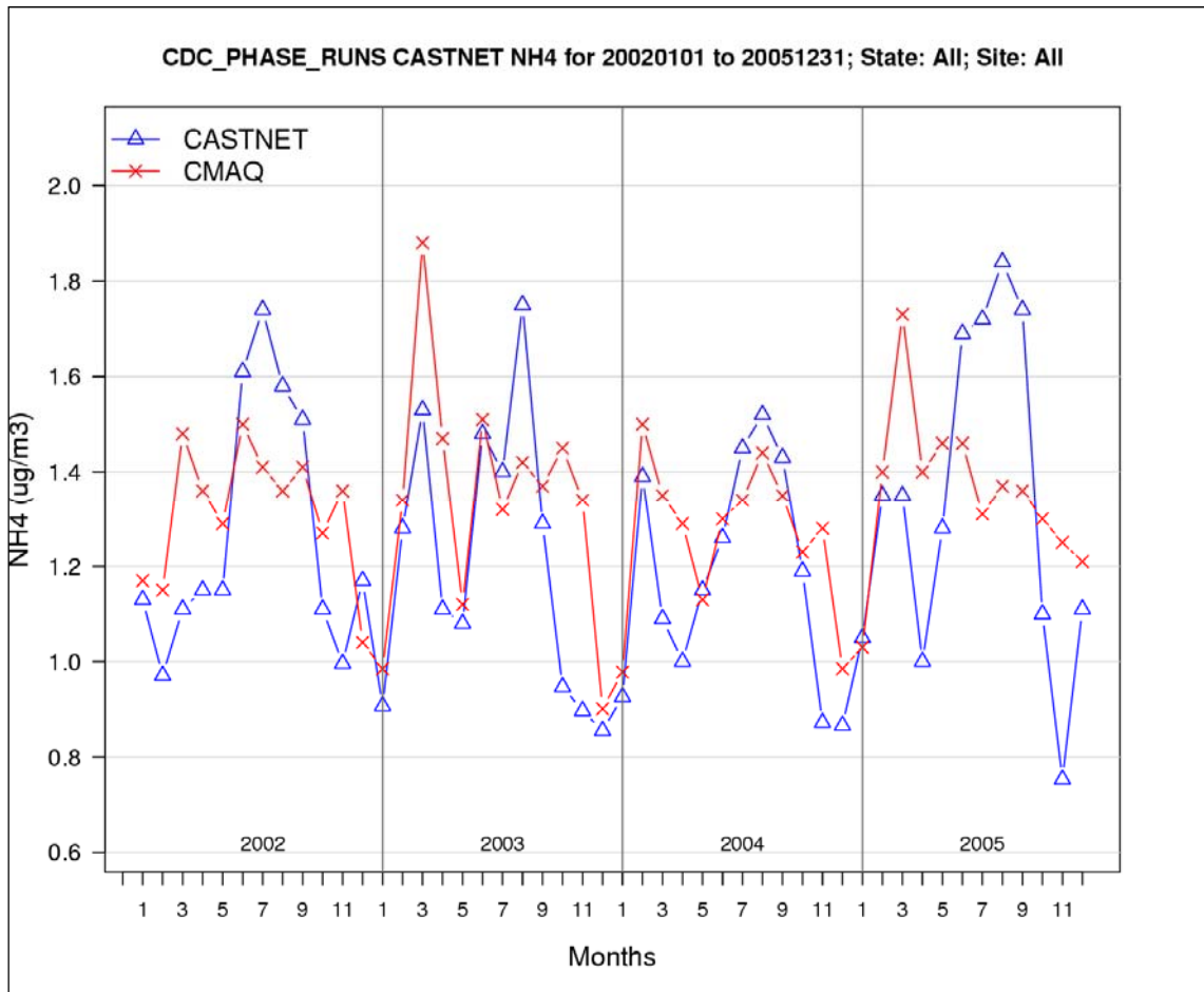
2 Figure F-7 2002–2005 Domain-wide average NH 4 + predicted concentrations and observations 3 by month at CASTNet sites in the eastern domain (note, units are in actual mass for NH 4 , 4 including hydrogen).
