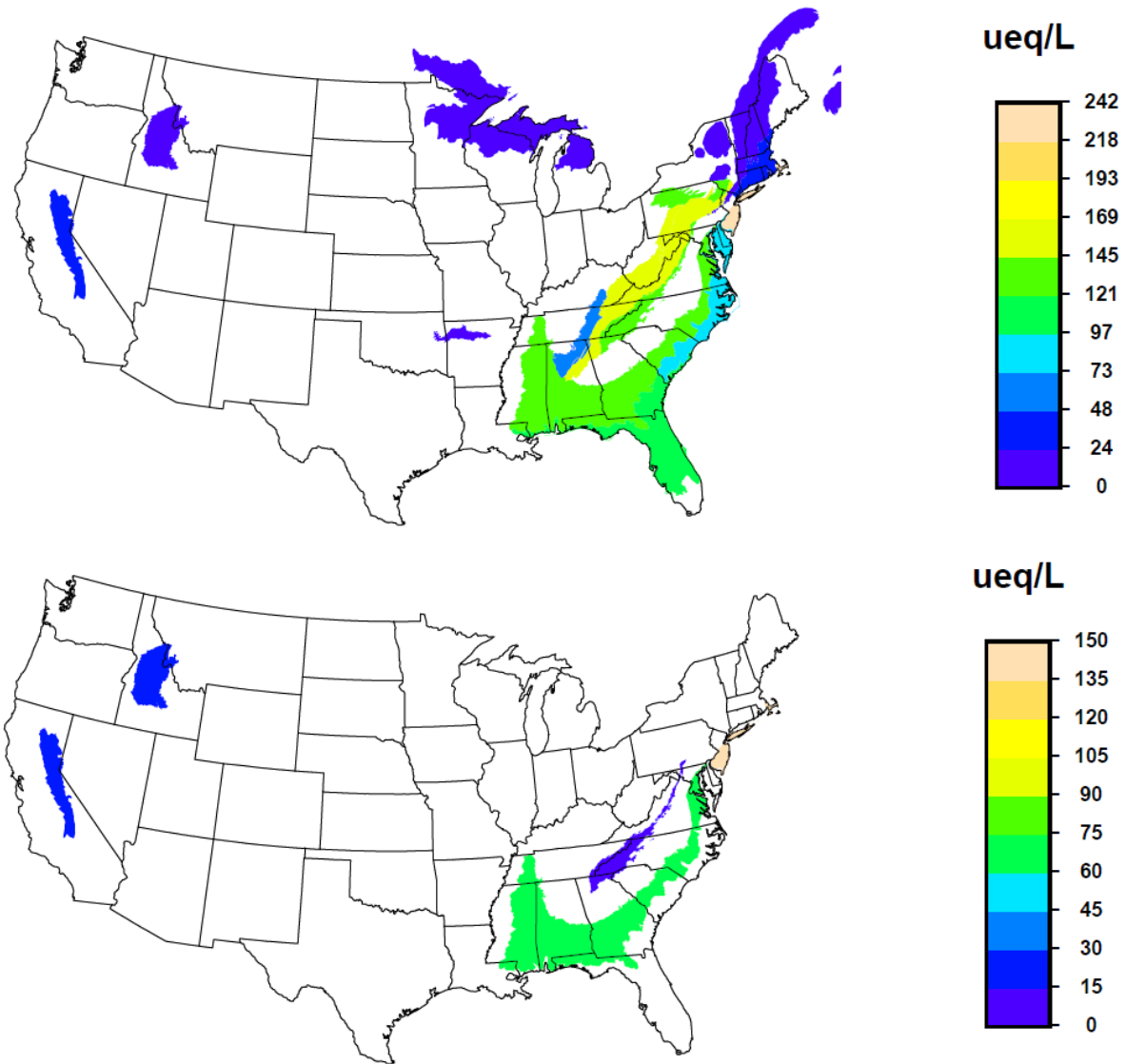
Figure D-7. Acid sensitive ecoregion level III areas likely not meeting the standard when the level = 75 \mu\text{eq/L} and the form is based on the 70 th percentile water body; based on CMAQ 2005 (top) and emissions sensitivity(bottom) simulations. The legend reflects the magnitude of the exceedance relative to the specified level of the standard.
