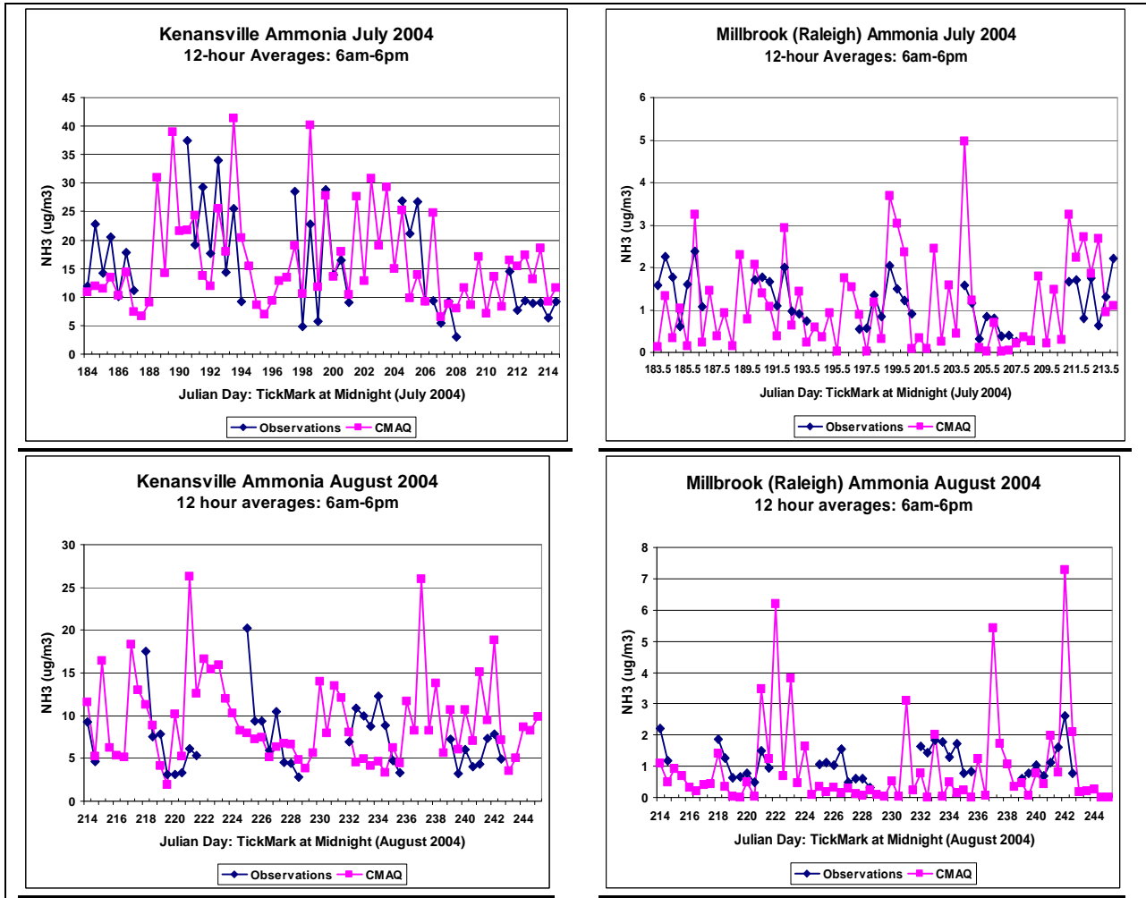
3 Figure F-8. Comparison of CMAQ predictions and measurements for 12-hour (6am-6pm) 4 average NH 3 concentrations, with a monitoring cycle of 4 days on and 4 days off, at a high 5 emission site (Kenansville) and a low emission urban site (Raleigh) in North Carolina compared 6 to CMAQ for July 2004 (top) and August 2004 (bottom), from Dennis et al., 2010 (note, units 7 are in actual mass for NH 3 , including hydrogen). 8 9
