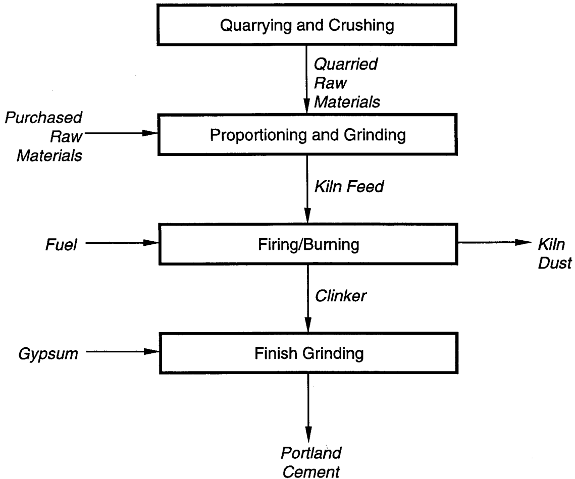
Figure 2-1. Basic flow diagram of the Portland cement manufacturing process.
