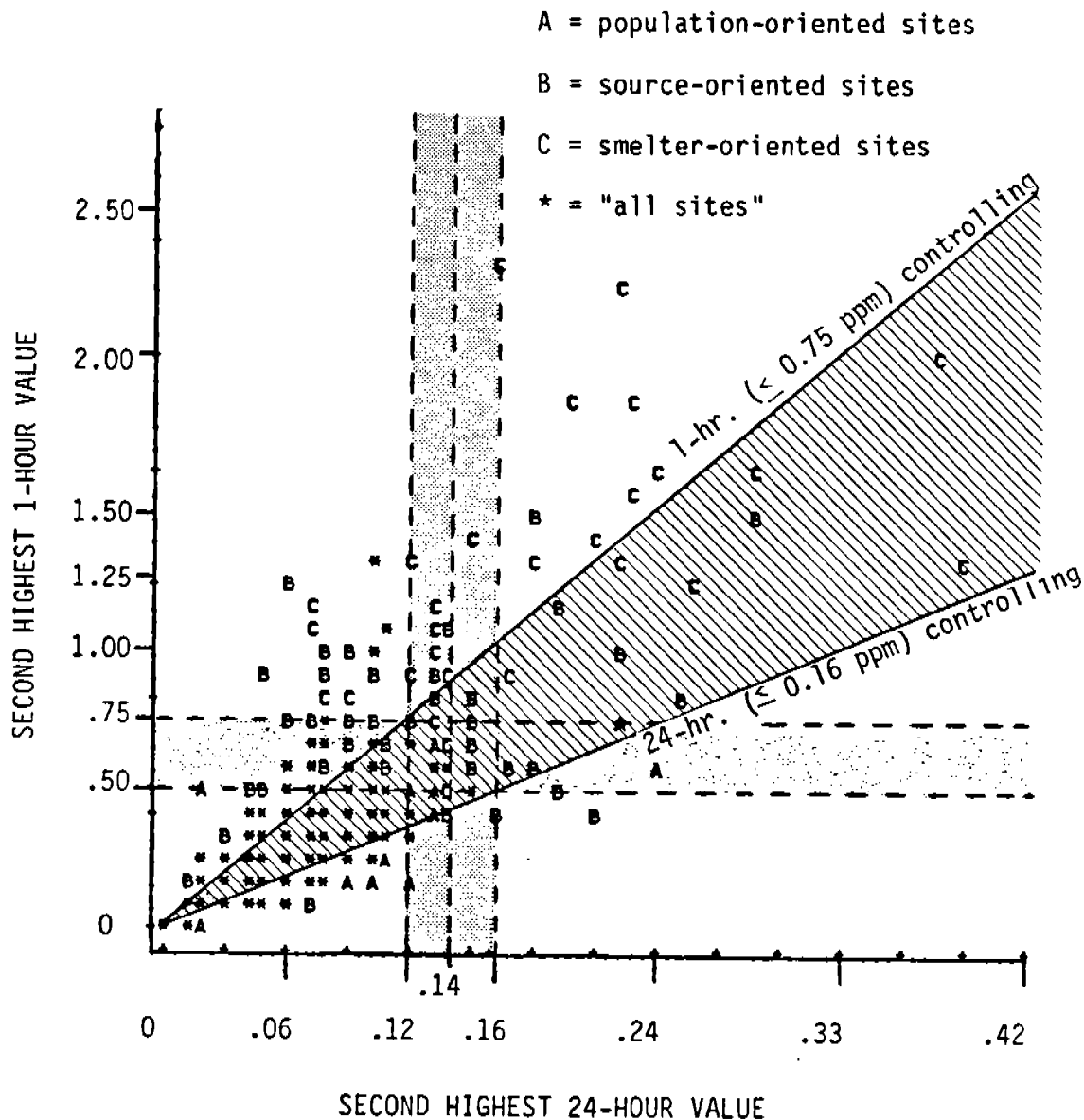
Figure D-1. Basic relationships between the second highest 1-hour value per year and the second highest 24-hour value (After Frank and Thrall, 1982). The initial staff ranges of interest for 1-hour standard (0.5 to 0.75 ppm) and possible 24-hour surrogates (0.12 to 0.16 ppm) are indicated by shading. Sites with data above the diagonal line(s) would be "controlled" by 1-hour standards, while those below the diagonals would be controlled by 24-hour standards. In the hatched area, the controlling standard would vary. Based on the data in this figure, the current 24-hour standard would keep 1-hour values below 0.5 ppm in almost all of the population oriented sites, but would not prevent many of the source and most of the smelter sites from having at least two 1-hour values per year in excess of the indicated range.
