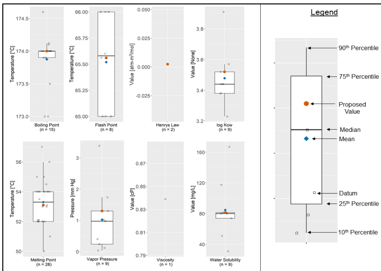
Figure 2-12. Box and Whisker Plots of Reported Physical and Chemical Property Value
