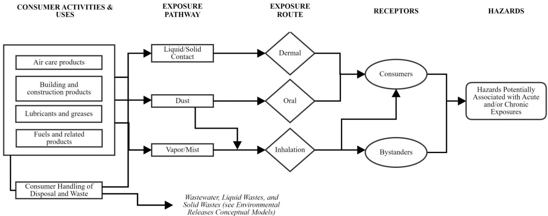
Figure 2-14. p -Dichlorobenzene Conceptual Model for Consumer Activities and Uses: Consumer Exposures and Hazards
