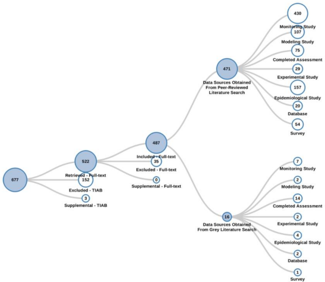
Figure 2-7. Peer-reviewed and Gray Literature Inventory Tree – Exposure Search Results for Butyl Benzyl Phthalate
