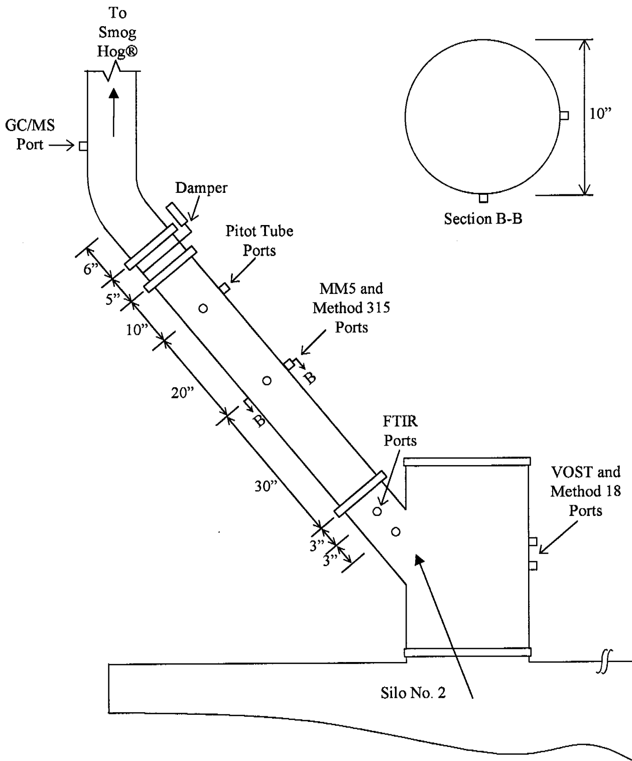
Figure 4.3 Silo Exhaust Duct Sampling Locations, Asphalt Plant C, California
