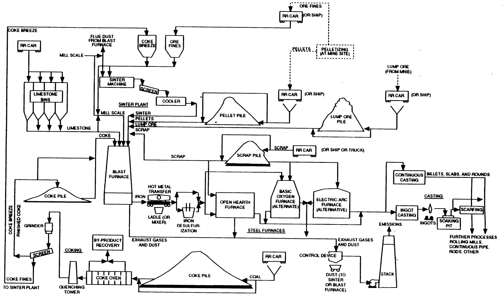
Figure 8-1. General flow diagram for the iron and steel industry. 90
