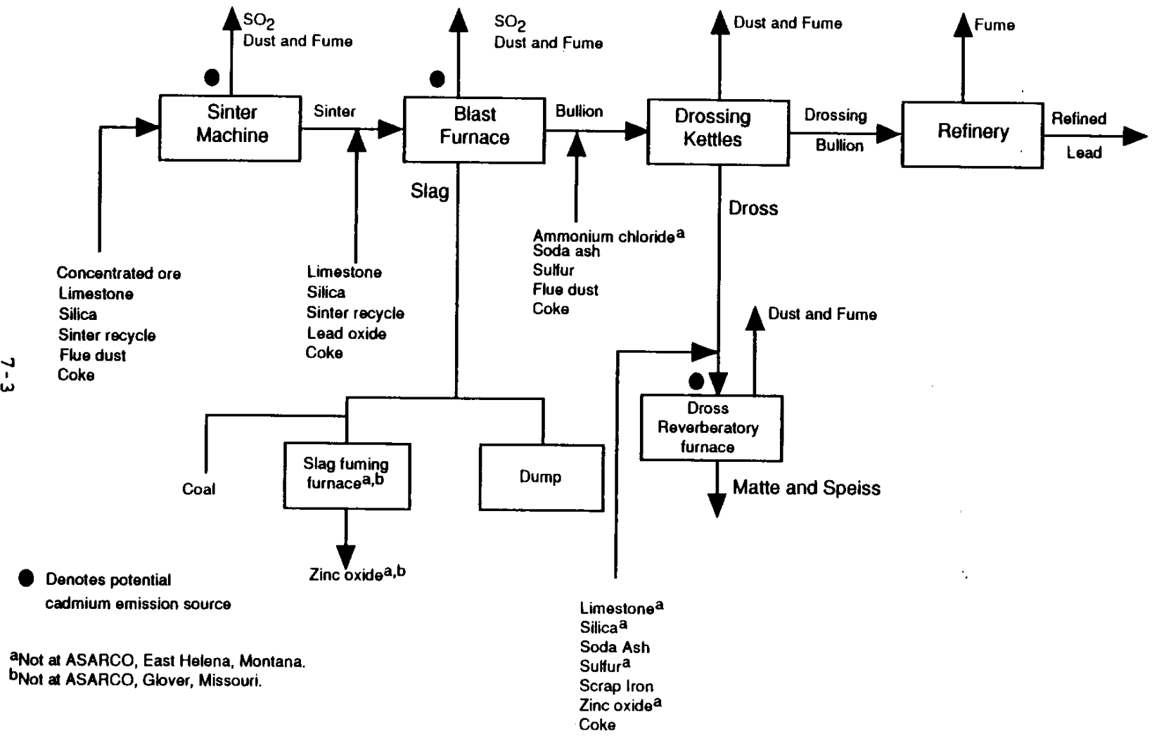
Figure 7-1. Typical primary lead-processing scheme. 90
