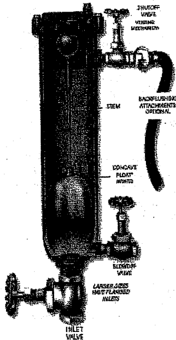
Figure 1: Air and Vacuum Relief Valve Assembly
