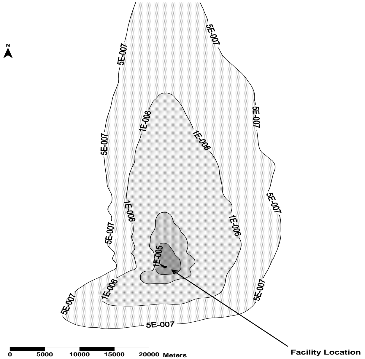
Figure 3-4. Cancer Risk Isopleths Around Erie Coke
