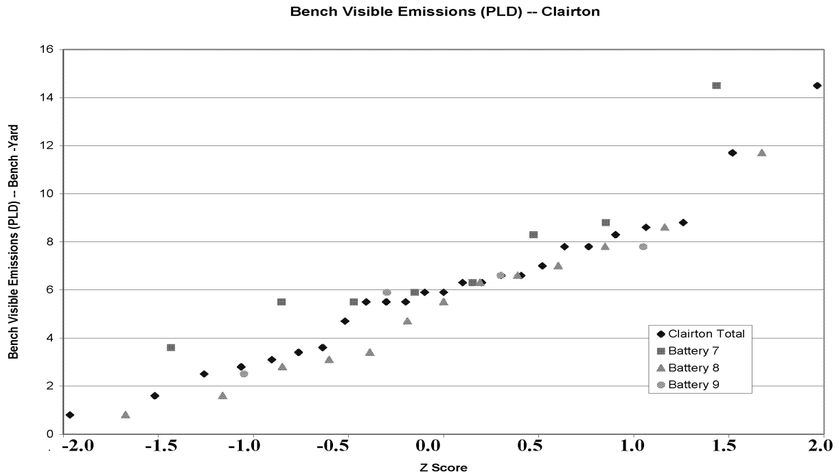
Figure 2-9. Comparison of Bench-only Visible Leaking Doors Across Batteries
