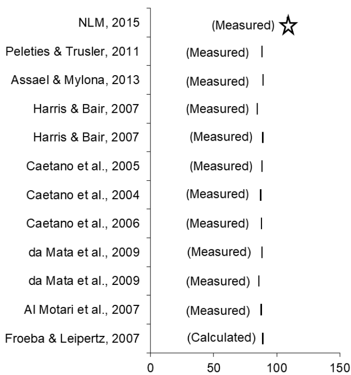
Figure_Apx B-1. Tornado Diagram for Viscosity Data Identified in Systematic Review
