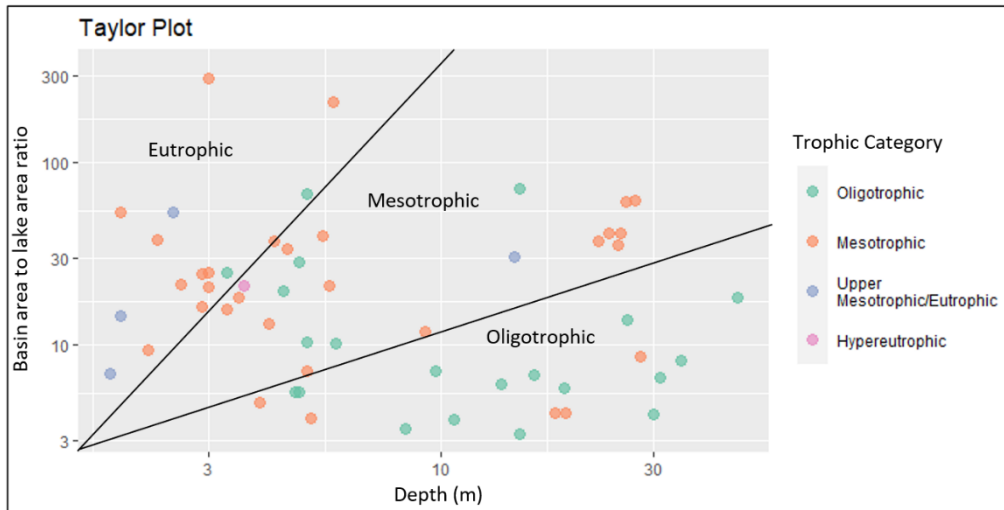
Figure 2-2 Base Plot of Lake Trophic Determination using Taylor Analysis
