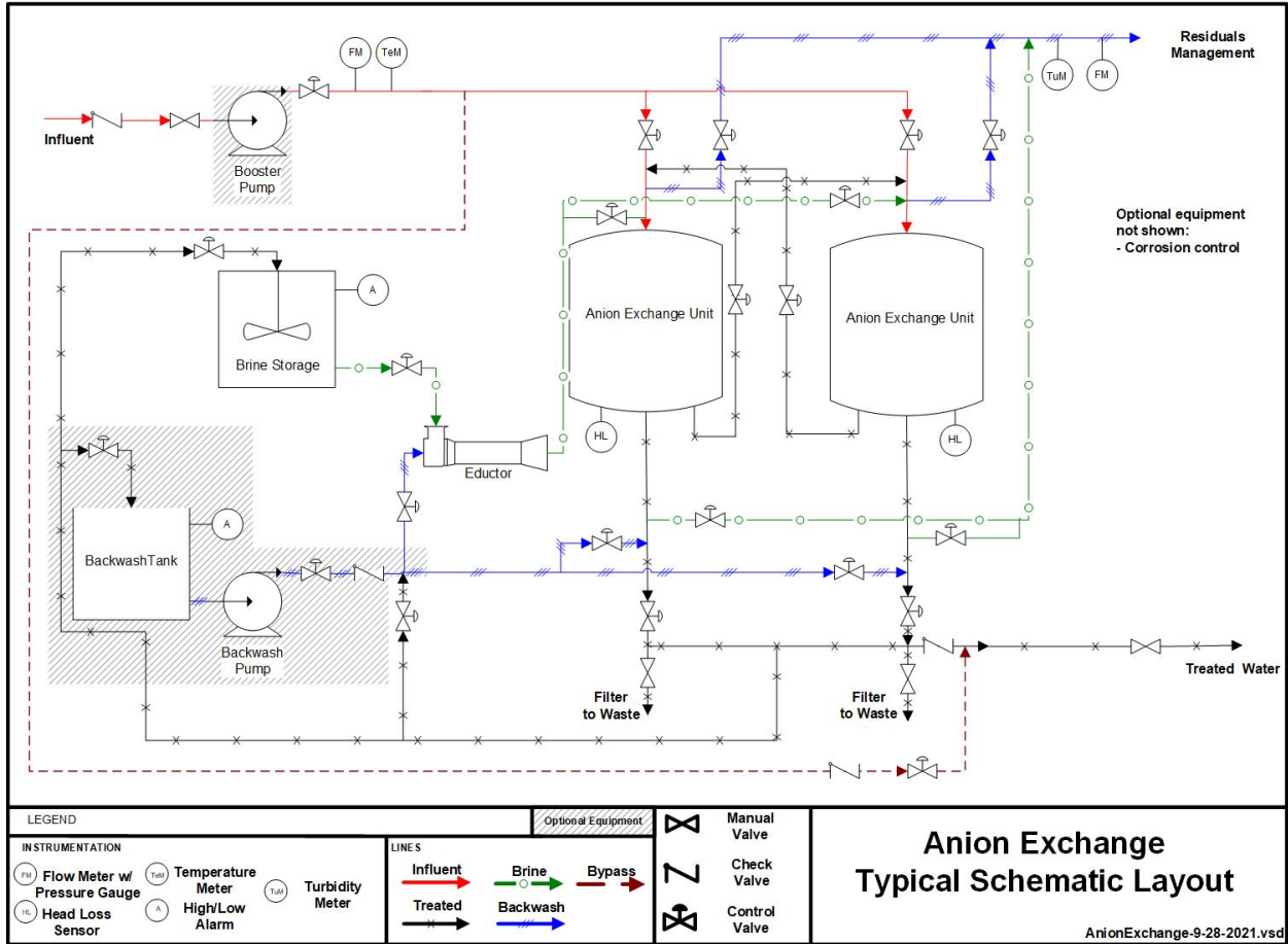
Exhibit 3-2. Typical Schematic Layout for Perchlorate Removal by Ion Exchange with Brine Regeneration
