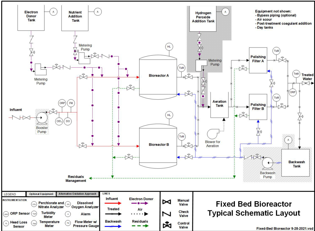
Exhibit 3-2. Typical Schematic Layout for Fixed Bed Bioreactor
