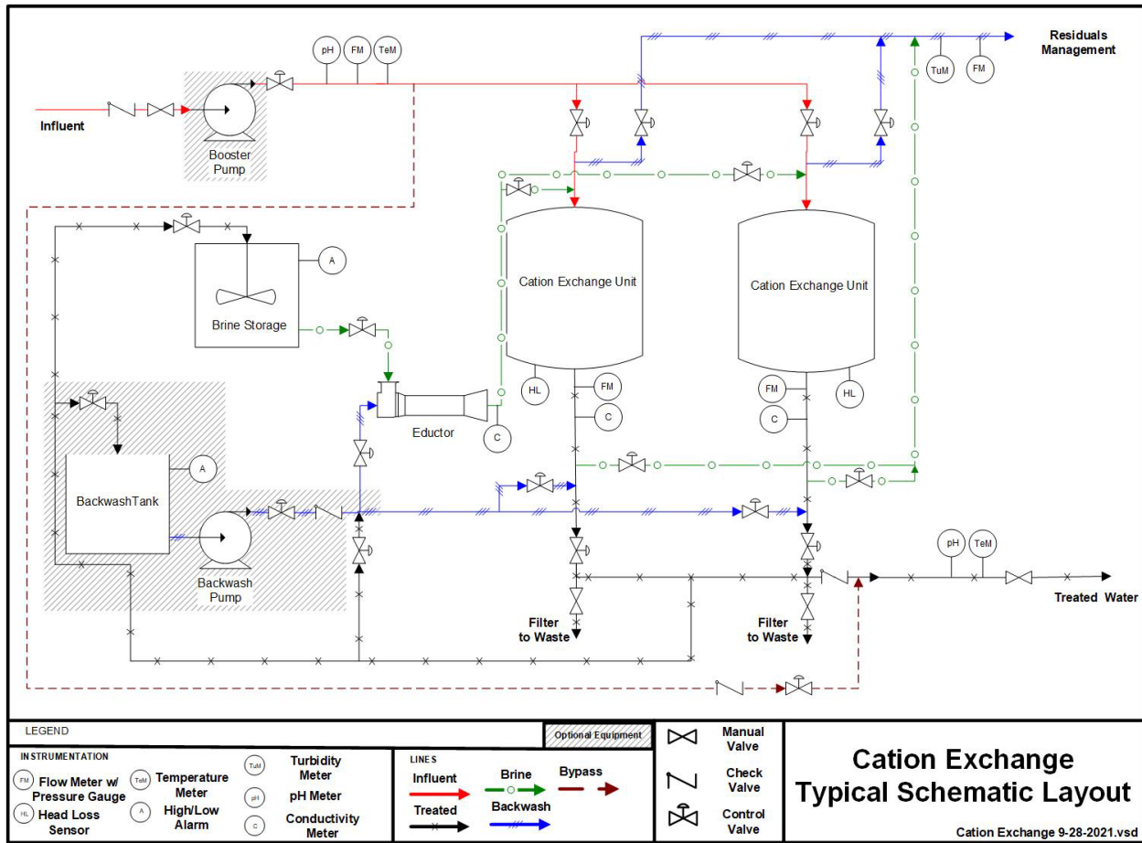
Exhibit 3-1. Typical Schematic Layout for Cation Exchange
