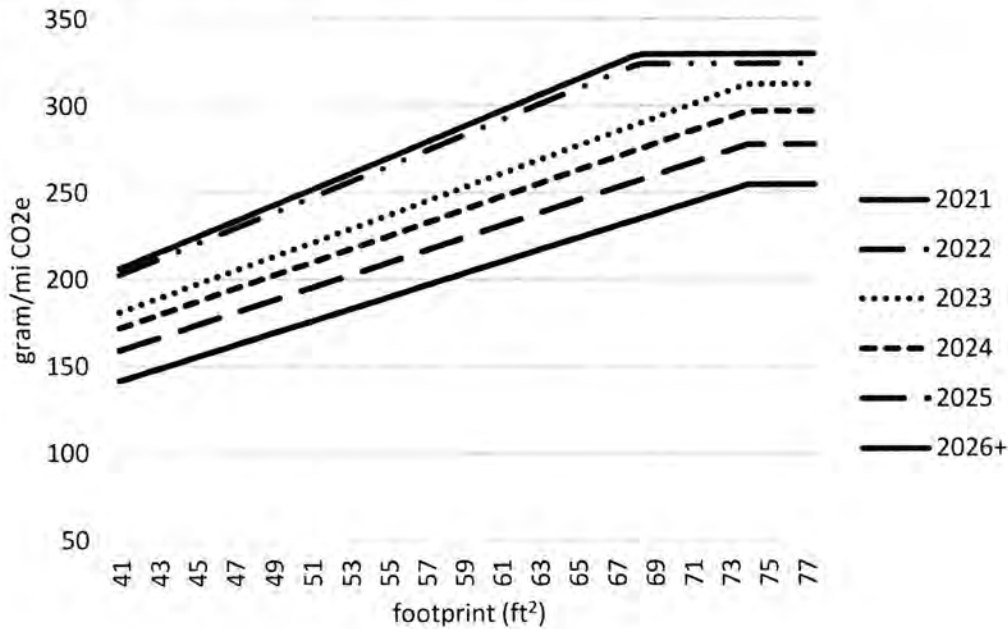
Figure 4 Truck Curves
