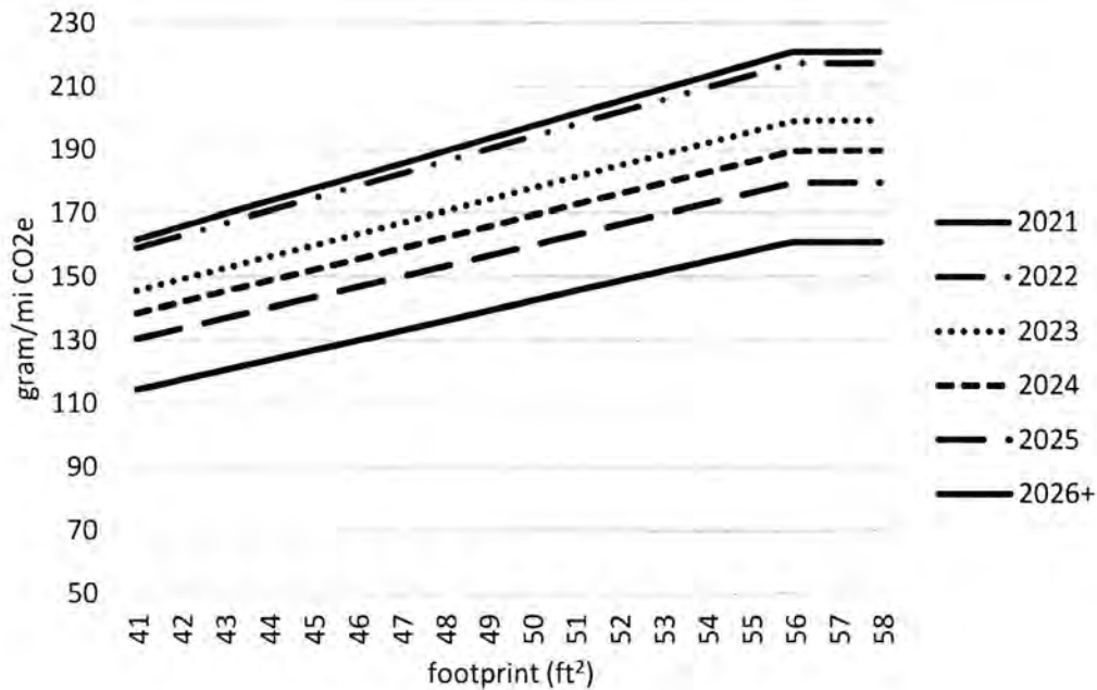
Figure 3 Car Curves
