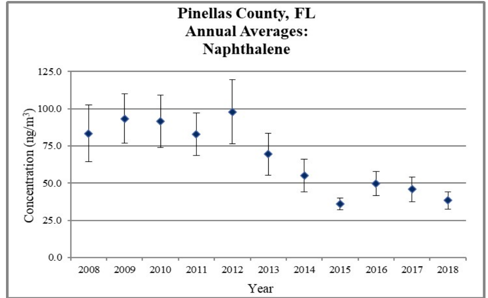
Figure 3. Pinellas County, FL Annual Average Concentrations
