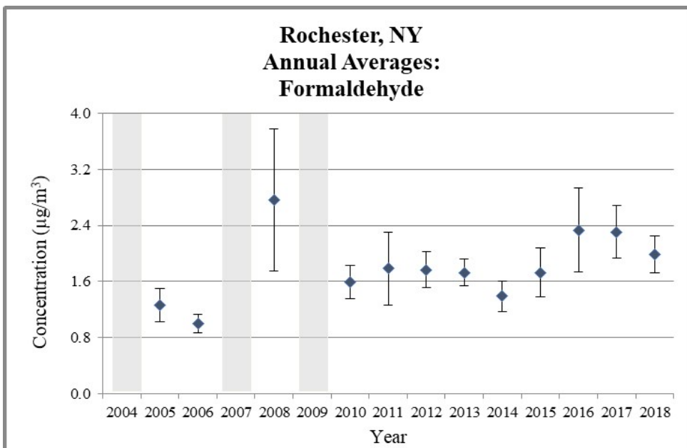
Figure 3. Rochester, NY Annual Average Concentrations
