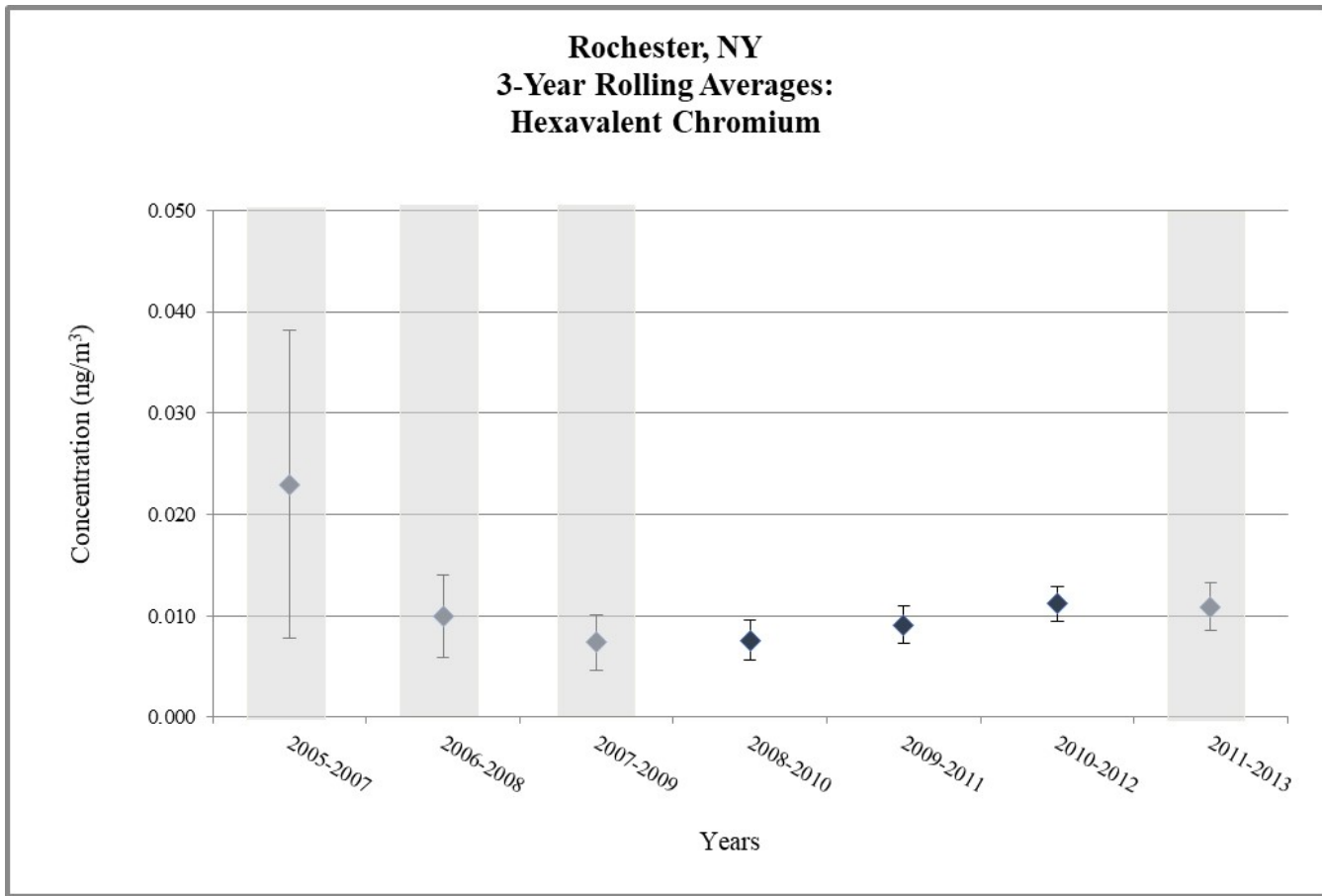
Figure 4. Rochester, NY - 3-Year Rolling Average Concentrations
