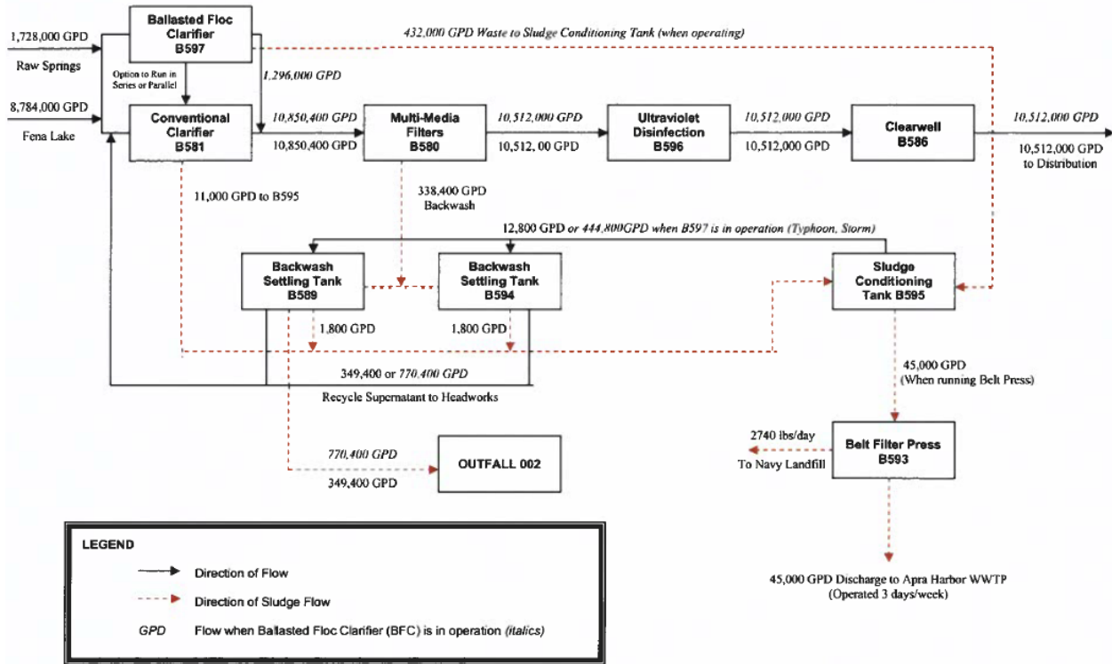
FWTP Water and Waste Flow Line Diagram
