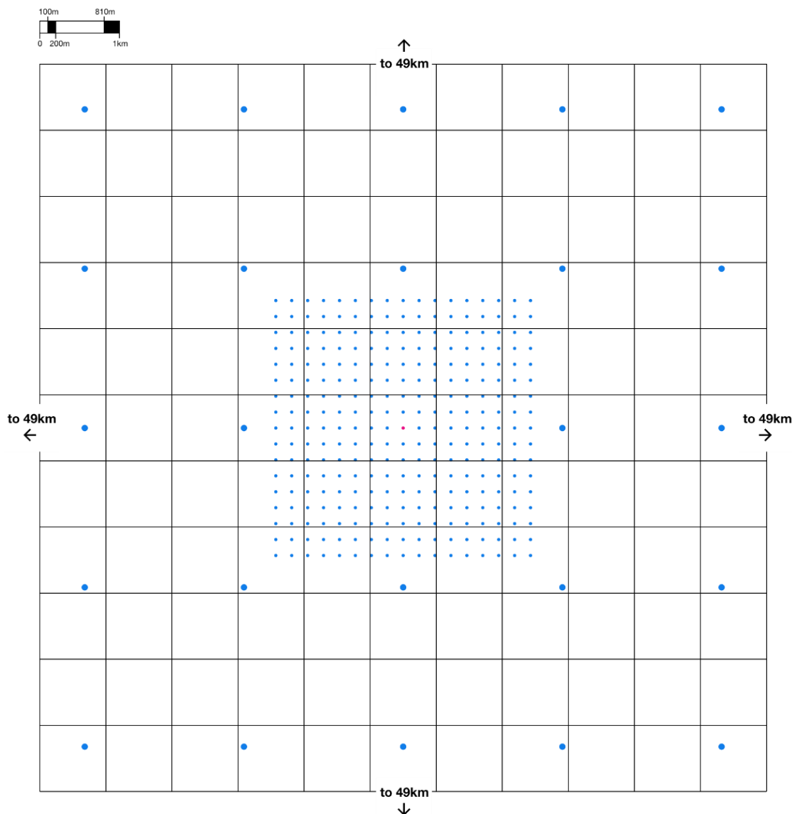
Exhibit 5.2 RSEI Grid Cells and AERMOD Receptor Points for Area Closest to Facility
